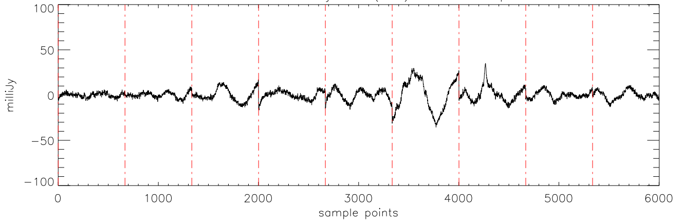
a2471 J07271824 02jan11 (AST) StokesI freq:5176.
