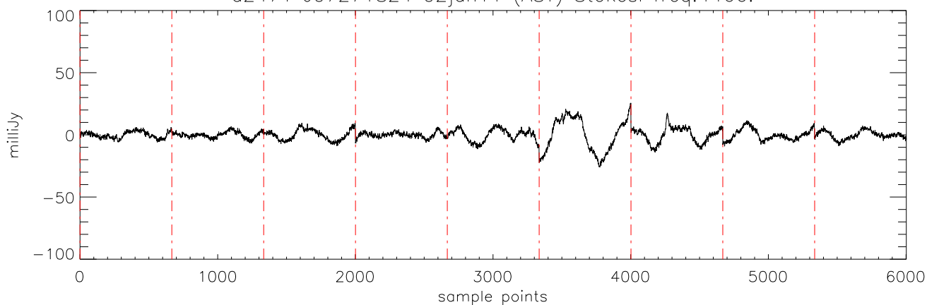
a2471 J07271824 02jan11 (AST) StokesI freq:4608.
