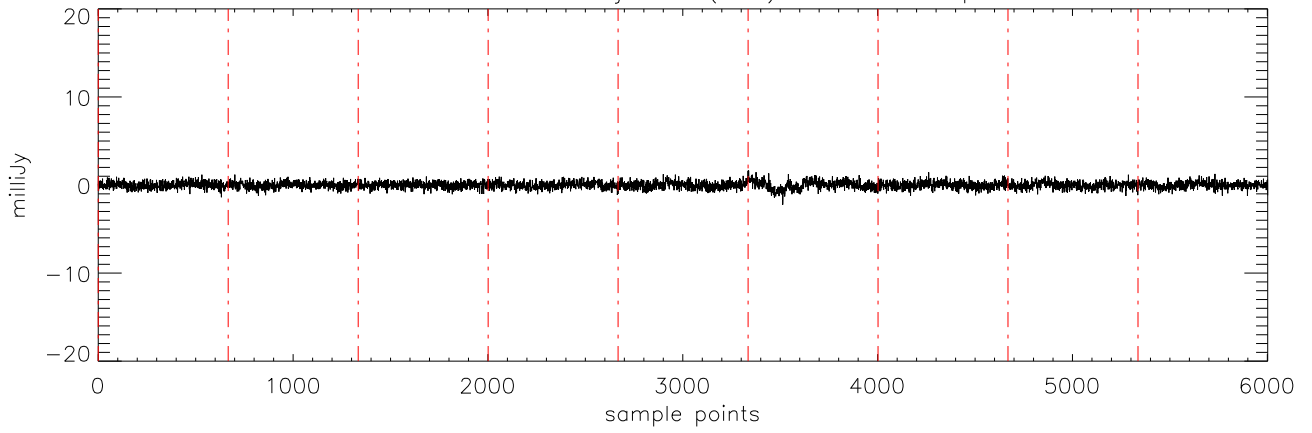
a2471 J07271824 02jan11 (AST) StokesV freq:4608.
