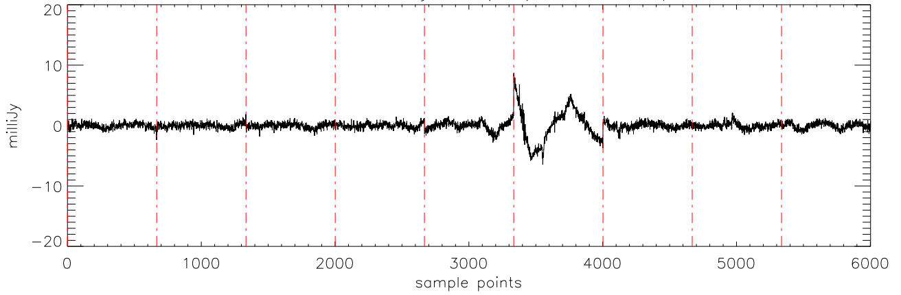
a2471 J07271824 02jan11 (AST) StokesU freq:4750.
