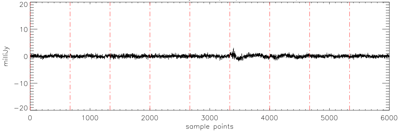
a2471 J07271824 02jan11 (AST) StokesV freq:4750.
