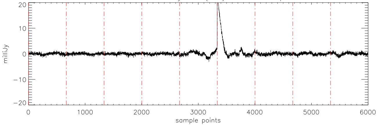
a2471 J07271824 02jan11 (AST) StokesU freq:4608.
