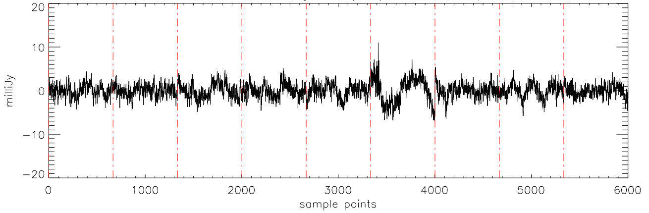
a2471 J07271824 02jan11 (AST) StokesQ freq:4750.
