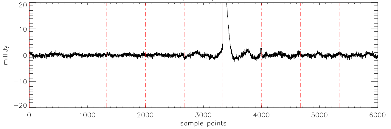
a2471 J07271824 02jan11 (AST) StokesU freq:5176.
