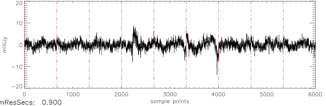
a2471 J07271824 02jan11 (AST) StokesQ freq:4466.
