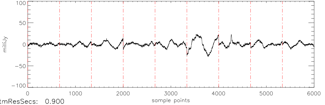
a2471 J07271824 02jan11 (AST) StokesI freq:5034.
