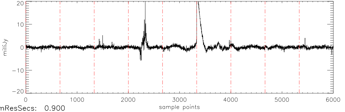
a2471 J07271824 02jan11 (AST) StokesU freq:4466.
