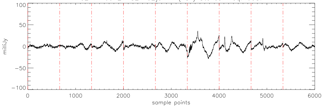
a2471 J07271824 02jan11 (AST) StokesI freq:4750.
