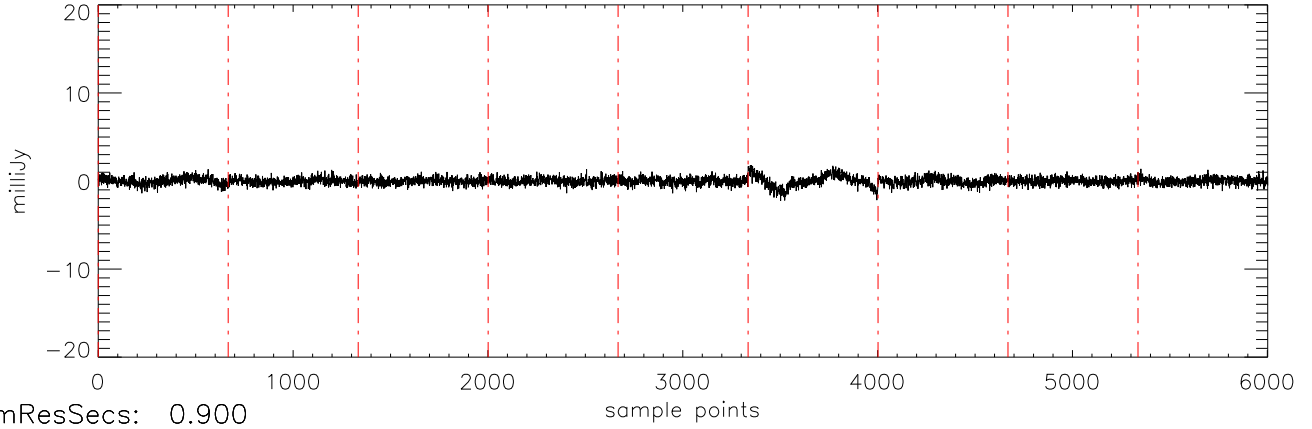
a2471 J07271824 02jan11 (AST) StokesV freq:5034.
