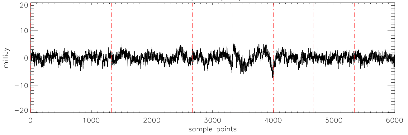
a2471 J07271824 02jan11 (AST) StokesQ freq:4608.
