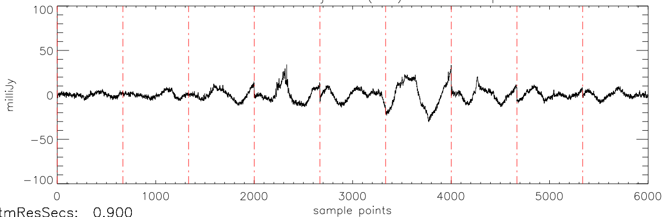
a2471 J07271824 02jan11 (AST) StokesI freq:4466.
