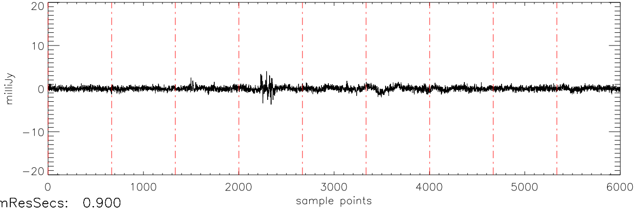
a2471 J07271824 02jan11 (AST) StokesV freq:4466.
