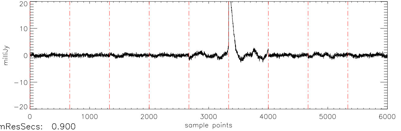
a2471 J07271824 02jan11 (AST) StokesU freq:5034.
