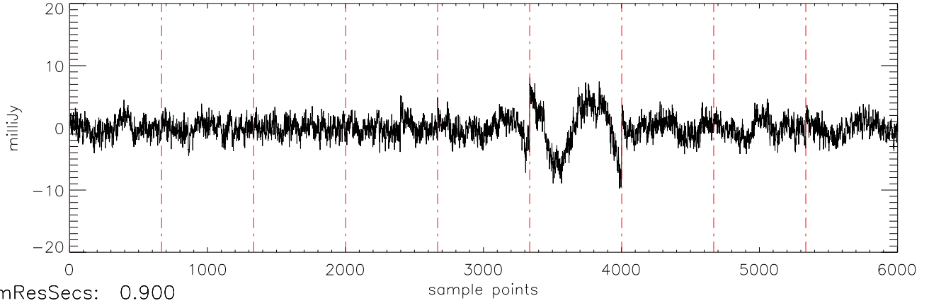
a2471 J07271824 02jan11 (AST) StokesQ freq:5034.
