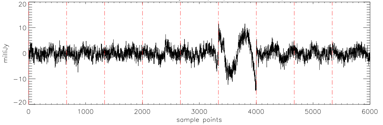
a2471 J07271824 02jan11 (AST) StokesQ freq:5176.
