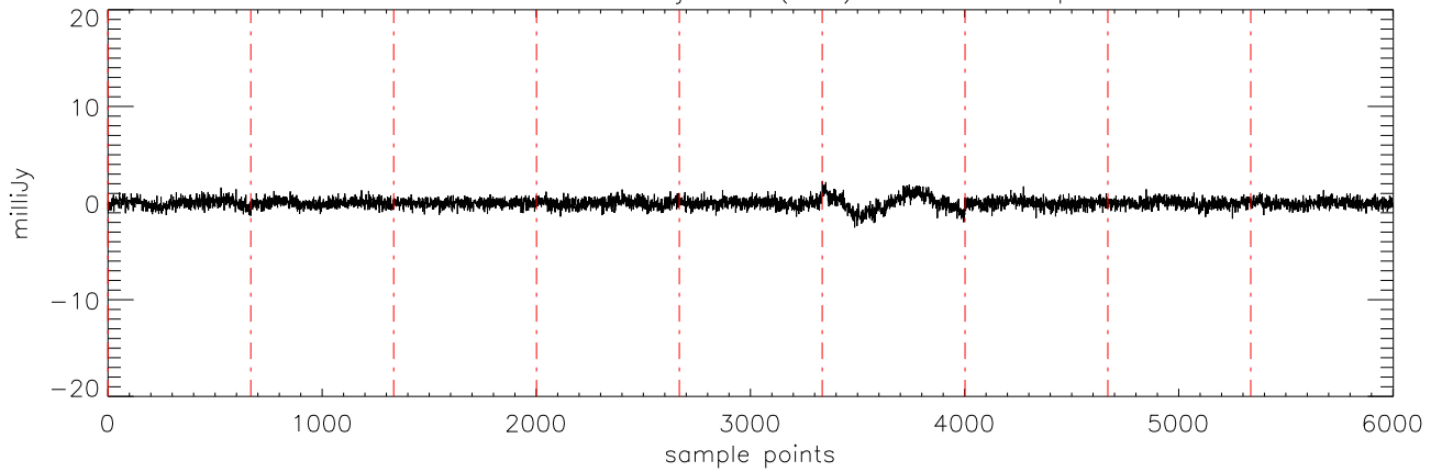
a2471 J07271824 02jan11 (AST) StokesV freq:5176.
