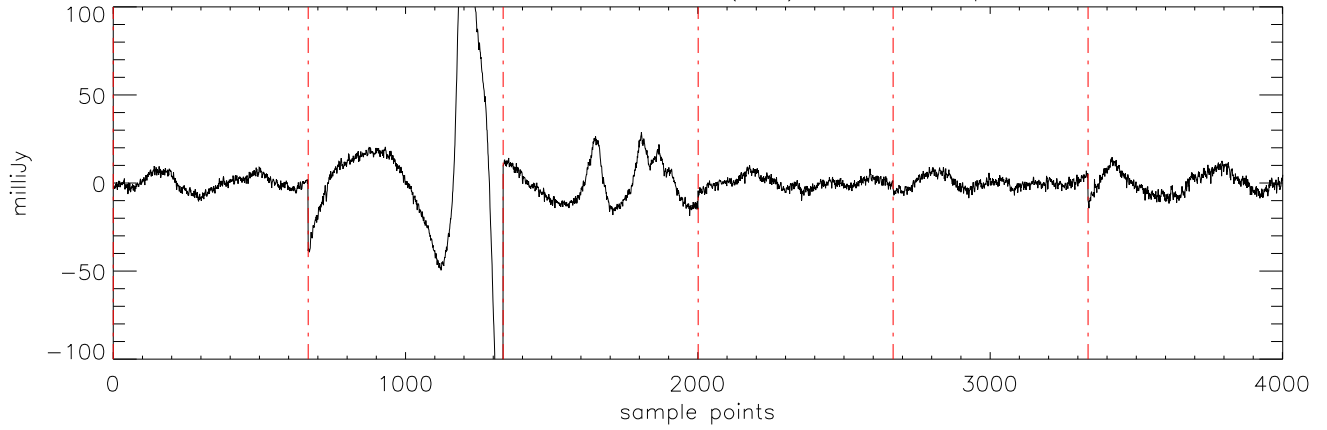
α2471 J03284265 21oct11 (AST) StokesI freq:5176.
