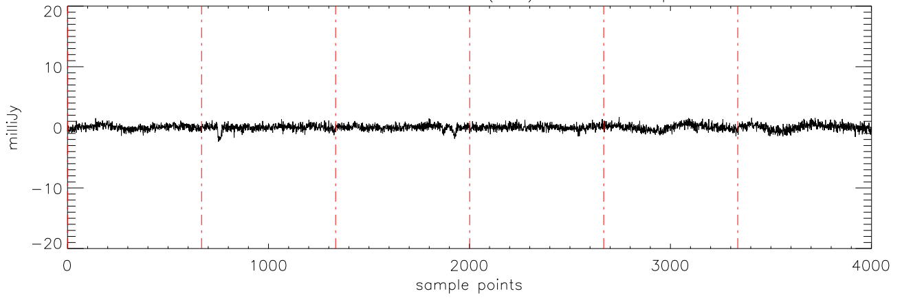
a2471 J03284265 21oct11 (AST) StokesV freq:4608.
