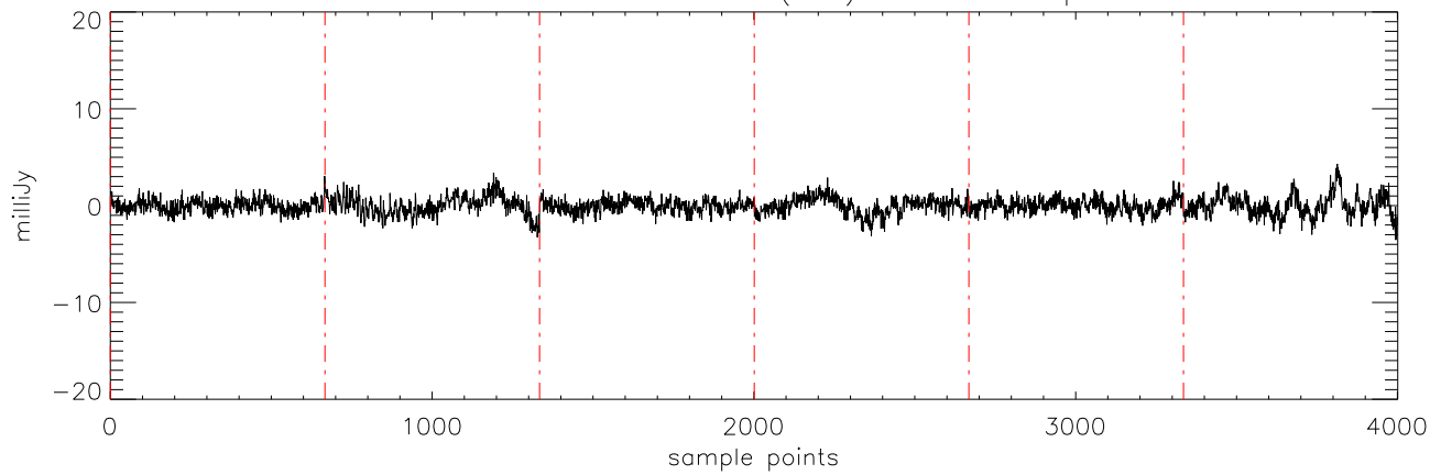
a2471 J03284265 21oct11 (AST) StokesU freq:5176.
