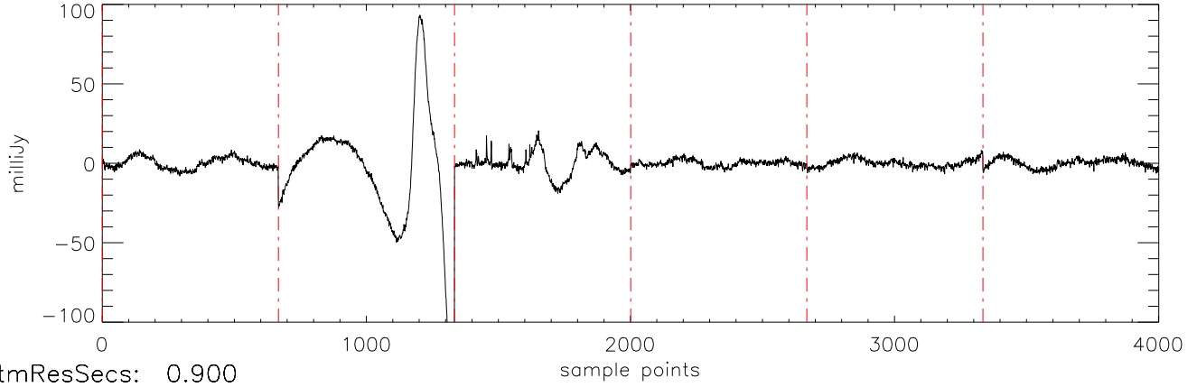
a2471 J03284265 21oct11 (AST) StokesI freq:4466.
