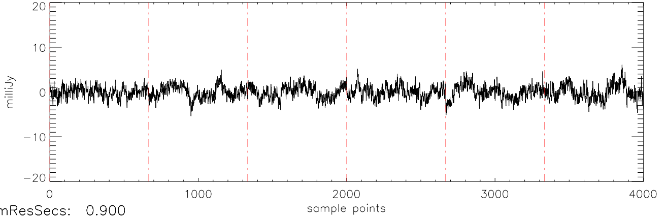
a2471 J03284265 21oct11 (AST) StokesQ freq:5034.
