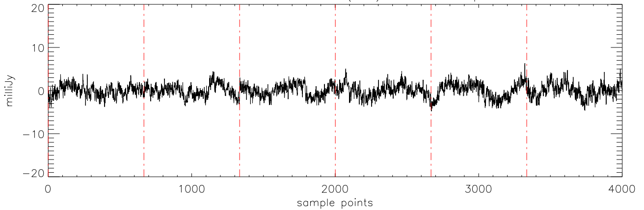
a2471 J03284265 21oct11 (AST) StokesQ freq:4750.
