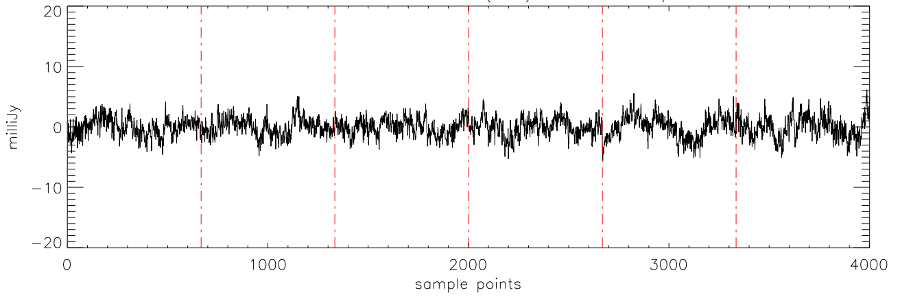
a2471 J03284265 21oct11 (AST) StokesQ freq:5176.
