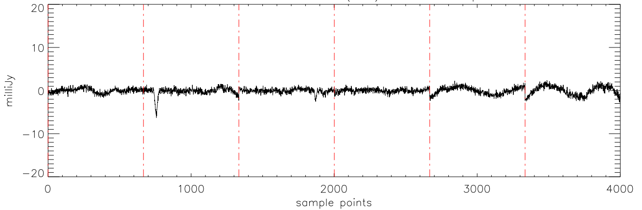
a2471 J03284265 21oct11 (AST) StokesU freq:4750.
