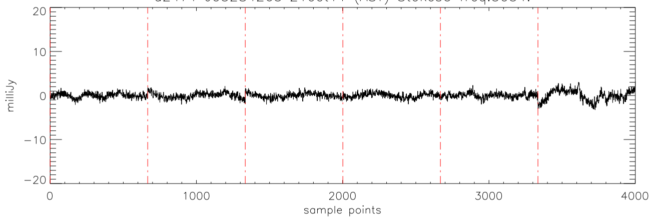
a2471 J03284265 21oct11 (AST) StokesU freq:5176.
