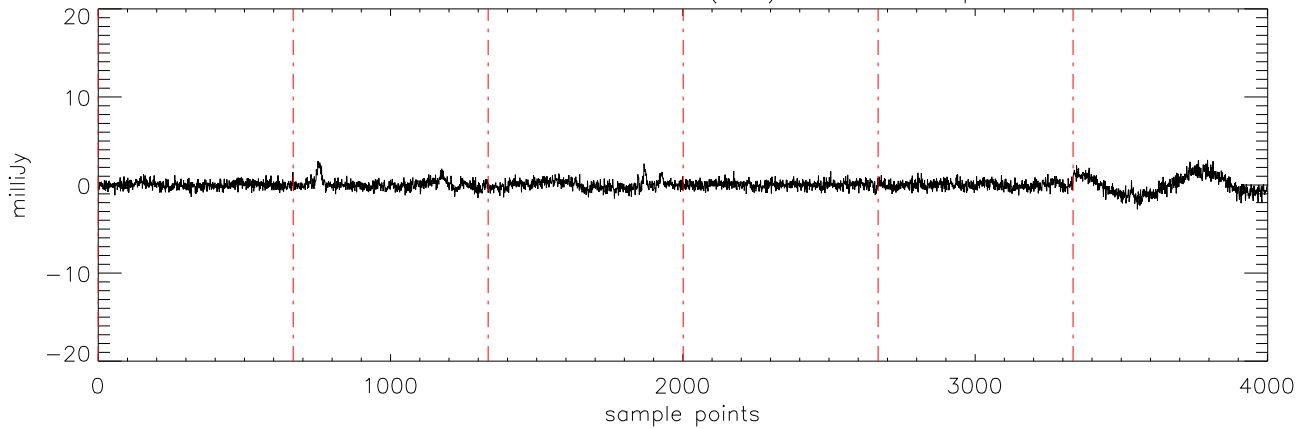
a2471 J03284265 21oct11 (AST) StokesV freq:4750.
