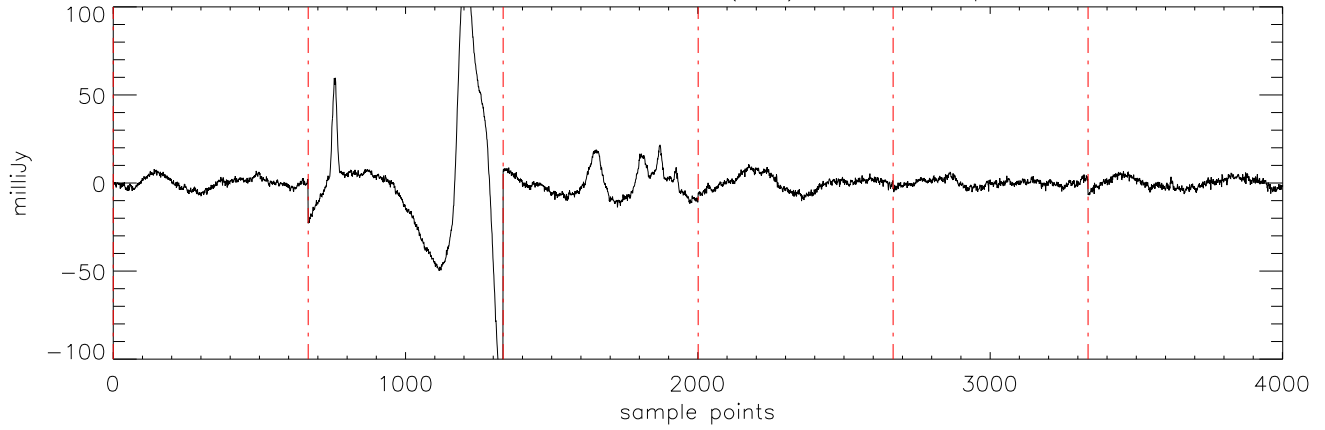
a2471 J03284265 21oct11 (AST) StokesI freq:4750.
