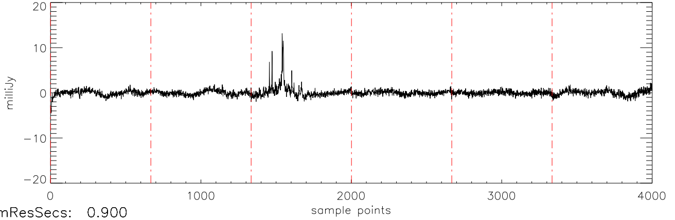
a2471 J03284265 21oct11 (AST) StokesU freq:4466.
