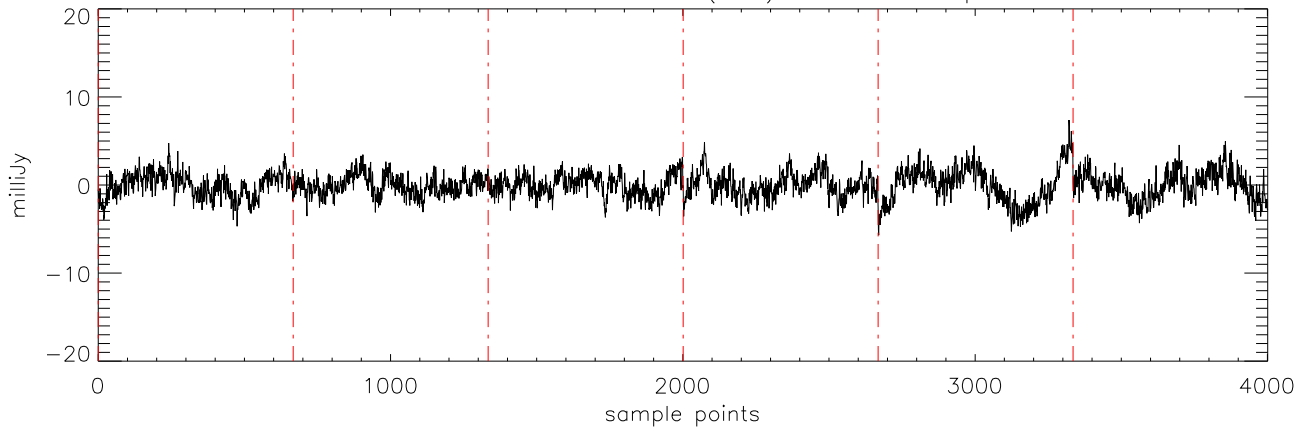
a2471 J03284265 21oct11 (AST) StokesQ freq:4608.
