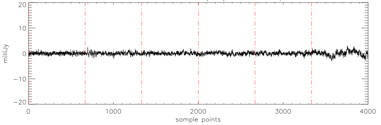
a2471 J03284265 21oct11 (AST) StokesV freq:5176.
