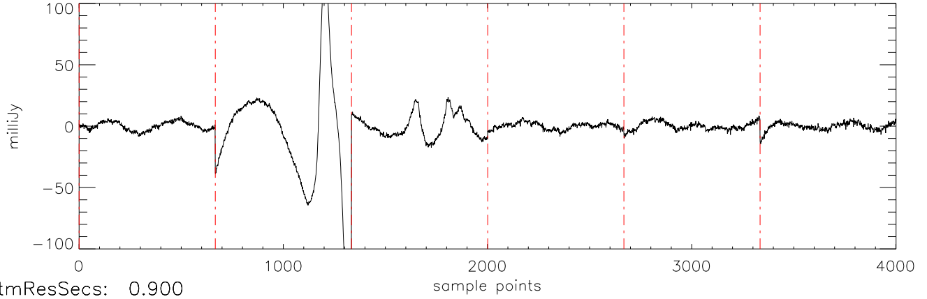
α2471 J03284265 21oct11 (AST) StokesI freq:5034.
