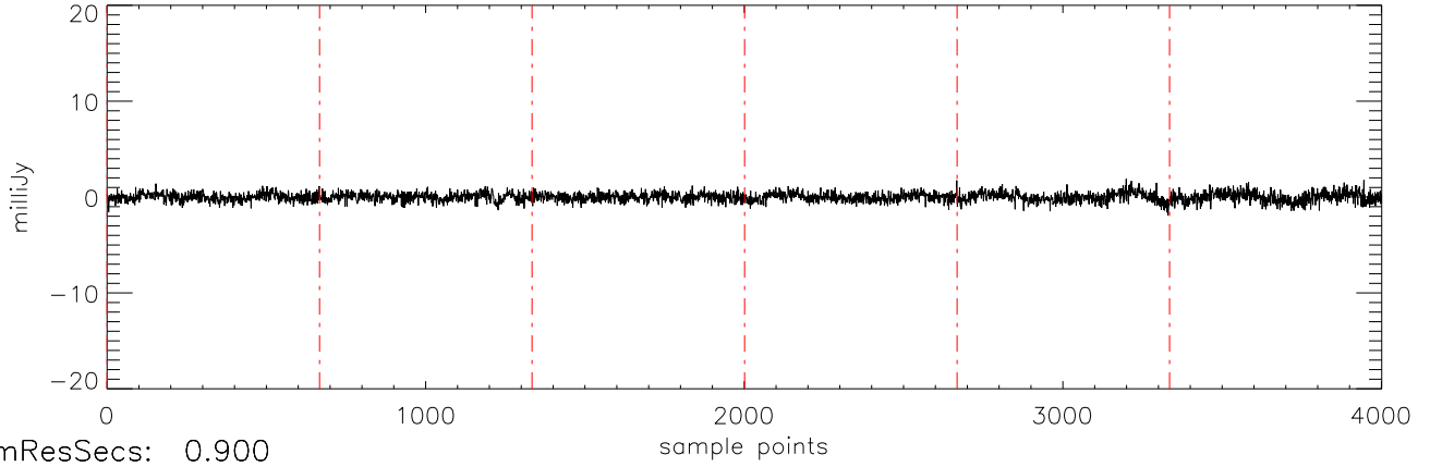
a2471 J03284265 21oct11 (AST) StokesV freq:5034.
