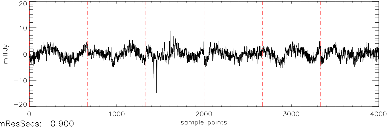
a2471 J03284265 21oct11 (AST) StokesQ freq:4466.
