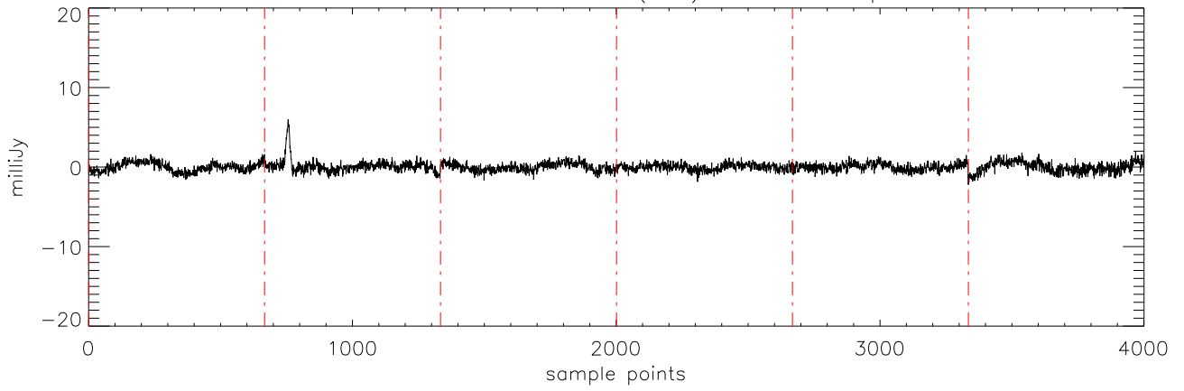
a2471 J03284265 21oct11 (AST) StokesU freq:4608.
