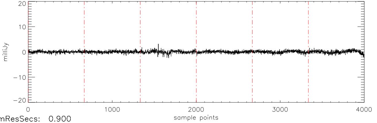
a2471 J03284265 21oct11 (AST) StokesV freq:4466.
