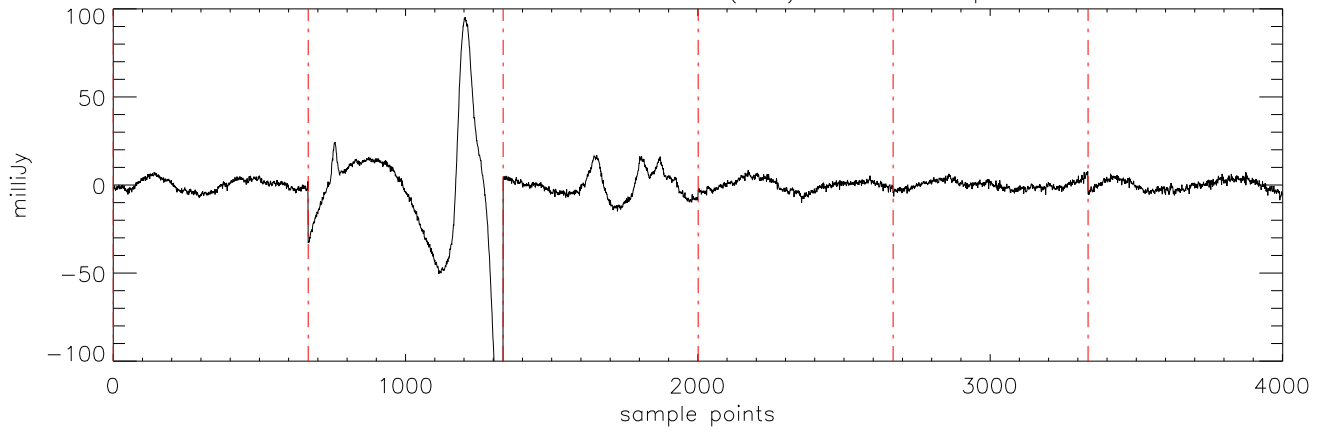
a2471 J03284265 21oct11 (AST) StokesI freq:4608.
