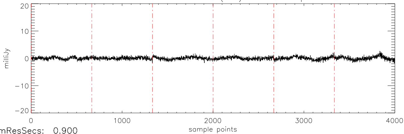
a2471 J03284265 21oct11 (AST) StokesU freq:5034.
