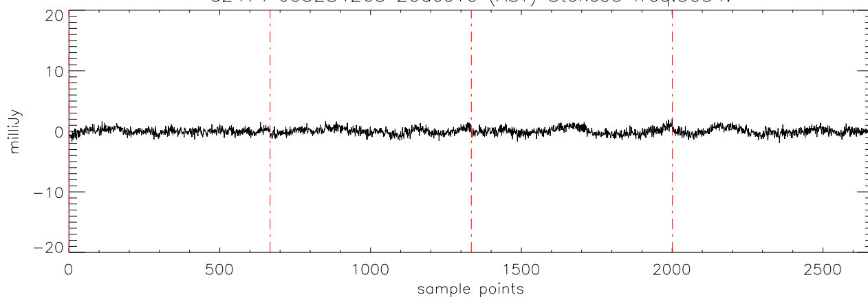
a2471 J03284265 20dec10 (AST) StokesU freq:5176.
