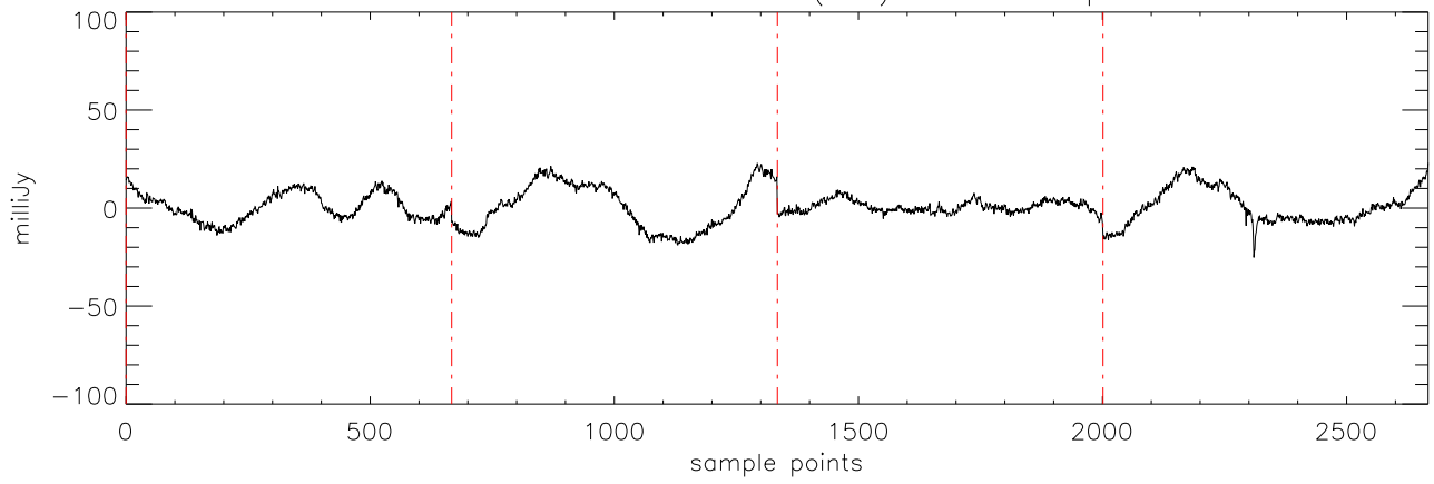
a2471 J03284265 20dec10 (AST) StokesI freq:5176.
