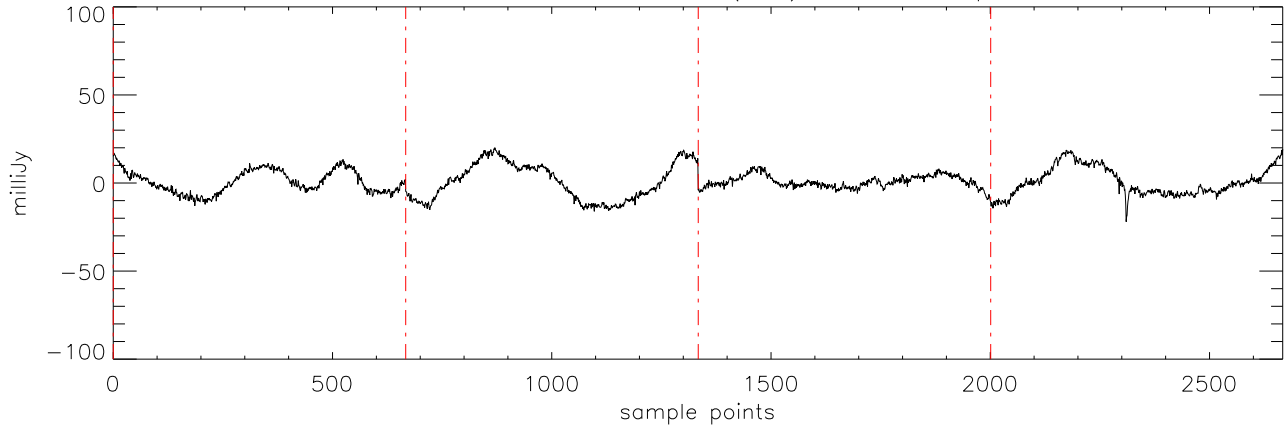
a2471 J03284265 20dec10 (AST) StokesI freq:4750.
