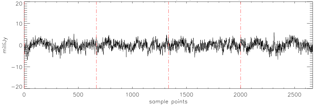
a2471 J03284265 20dec10 (AST) StokesQ freq:5176.
