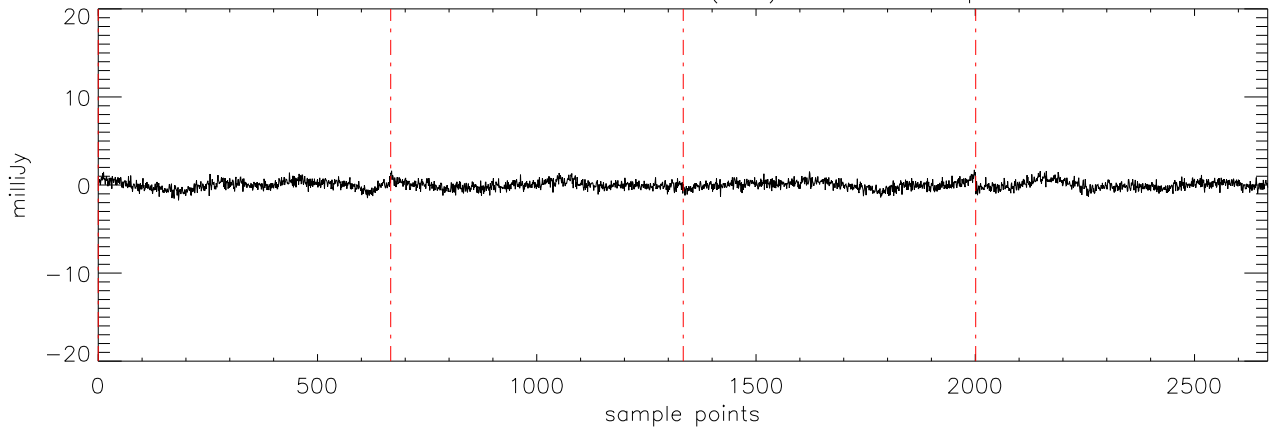
a2471 J03284265 20dec10 (AST) StokesU freq:4608.
