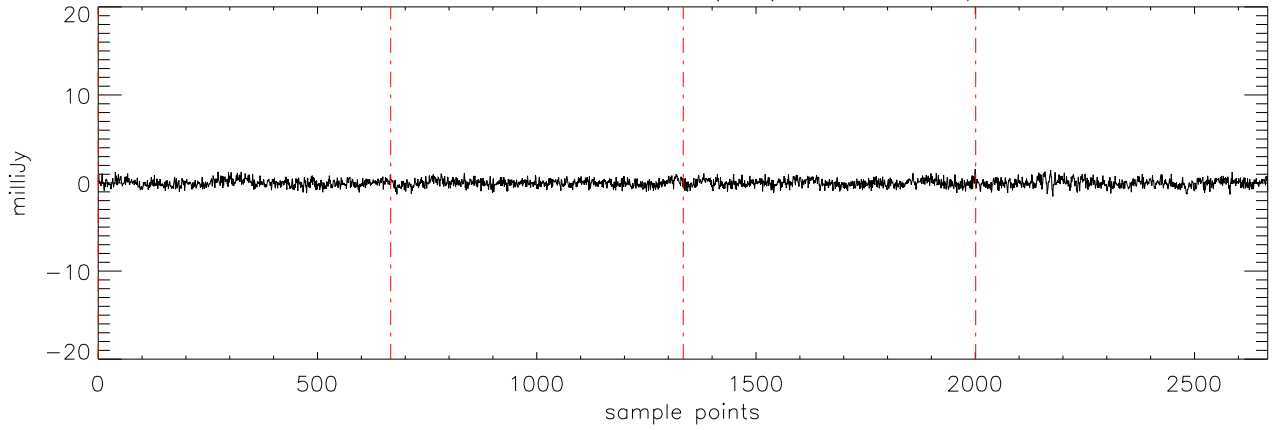
a2471 J03284265 20dec10 (AST) StokesV freq:4750.
