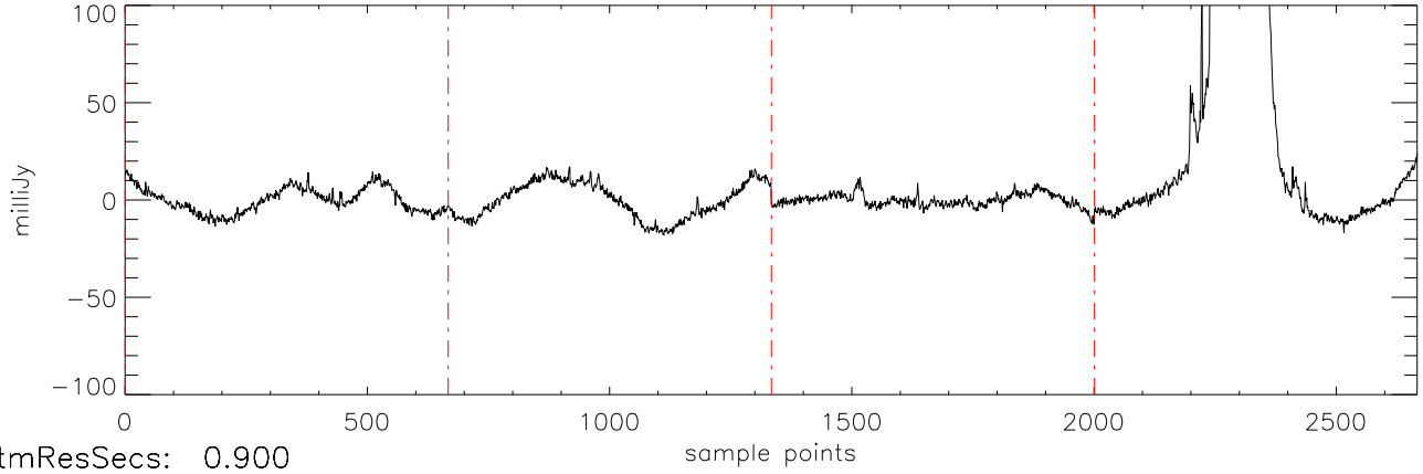
a2471 J03284265 20dec10 (AST) StokesI freq:4466.
