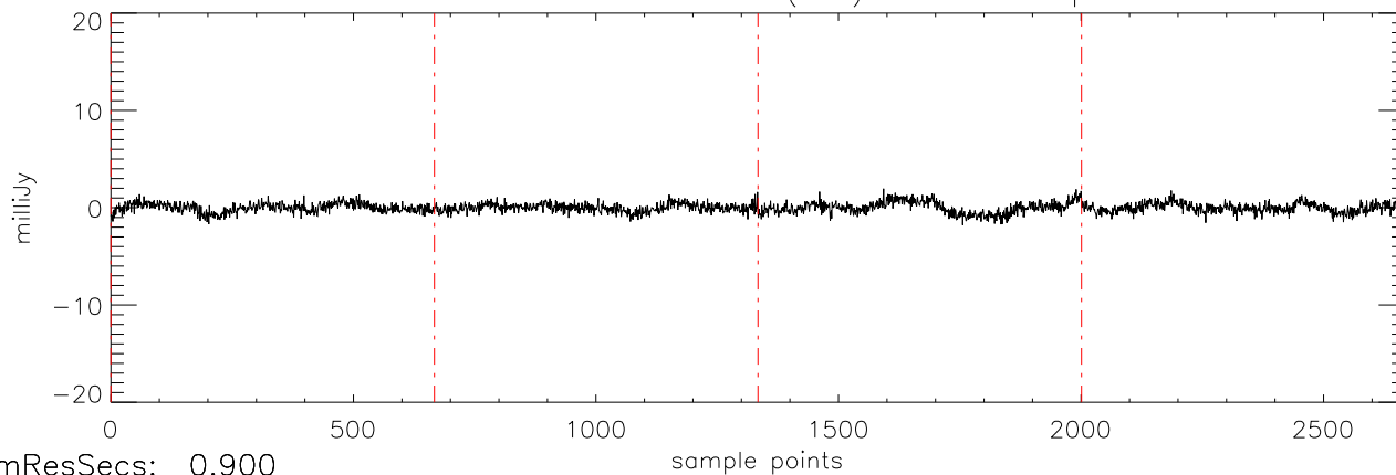
a2471 J03284265 20dec10 (AST) StokesU freq:5034.
