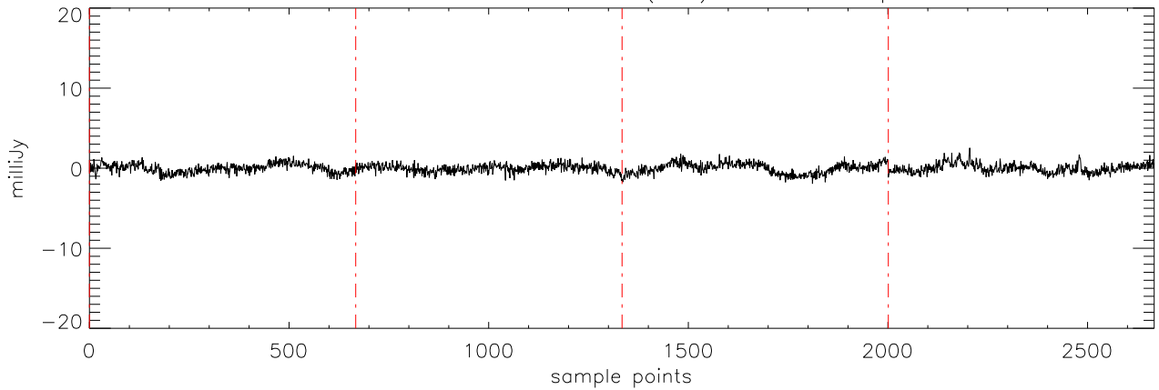
a2471 J03284265 20dec10 (AST) StokesU freq:4750.
