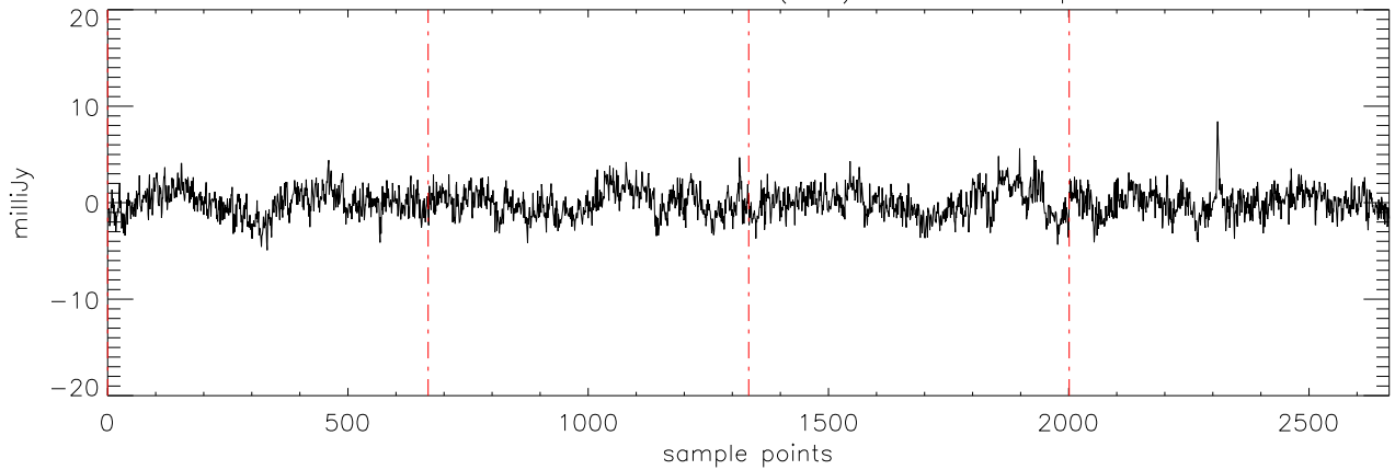
a2471 J03284265 20dec10 (AST) StokesQ freq:4750.
