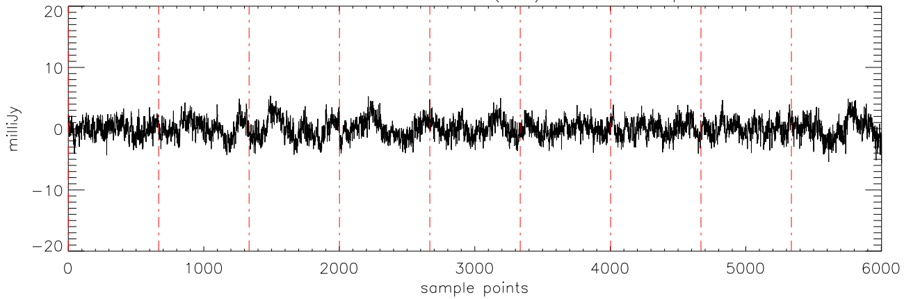
a2471 J03284265 17dec10 (AST) StokesQ freq:4608.
