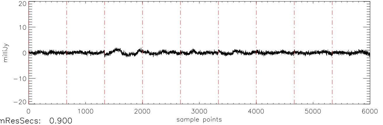
a2471 J03284265 17dec10 (AST) StokesU freq:5034.
