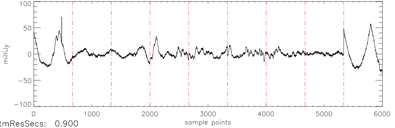
a2471 J03284265 17dec10 (AST) StokesI freq:5034.
