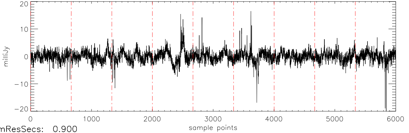
a2471 J03284265 17dec10 (AST) StokesQ freq:4466.
