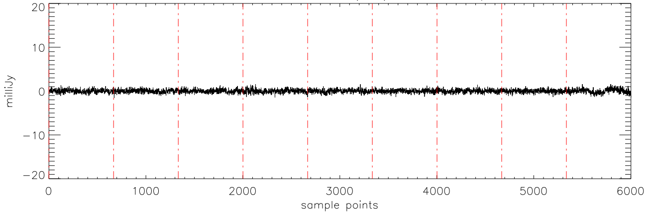
a2471 J03284265 17dec10 (AST) StokesV freq:4750.
