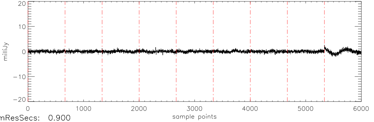
a2471 J03284265 17dec10 (AST) StokesV freq:5034.
