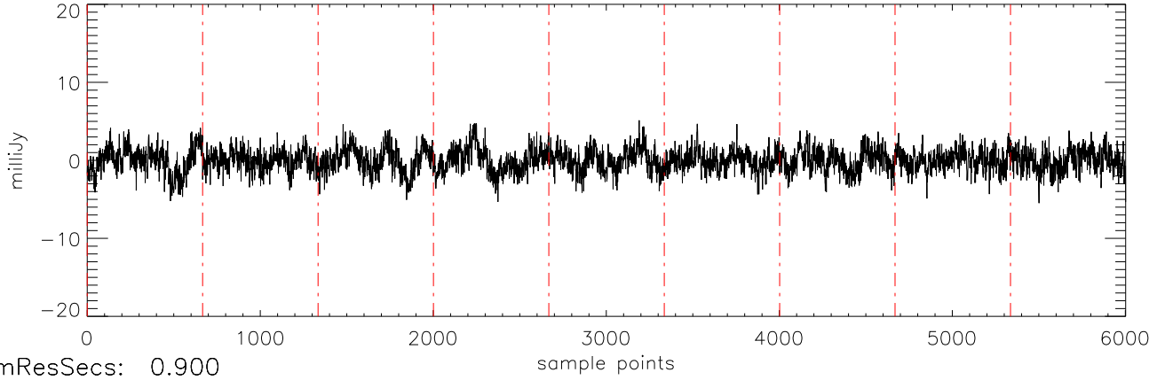
a2471 J03284265 17dec10 (AST) StokesQ freq:5034.
