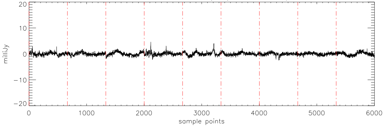
a2471 J03284265 17dec10 (AST) StokesU freq:4750.
