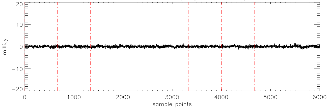
a2471 J03284265 17dec10 (AST) StokesV freq:4608.
