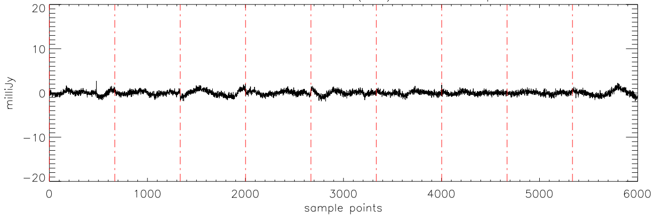
a2471 J03284265 17dec10 (AST) StokesU freq:4608.
