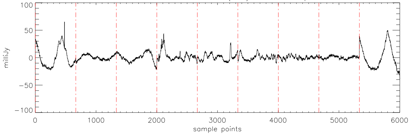
a2471 J03284265 17dec10 (AST) StokesI freq:4750.
