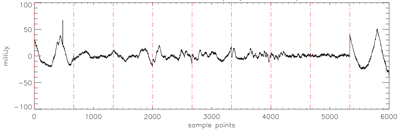
a2471 J03284265 17dec10 (AST) StokesI freq:4608.
