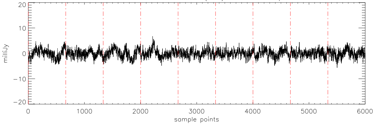
a2471 J03284265 17dec10 (AST) StokesQ freq:5176.
