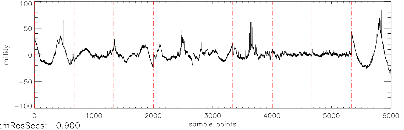
a2471 J03284265 17dec10 (AST) StokesI freq:4466.
