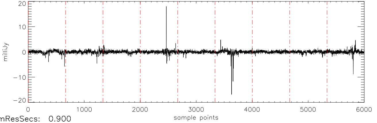
a2471 J03284265 17dec10 (AST) StokesV freq:4466.
