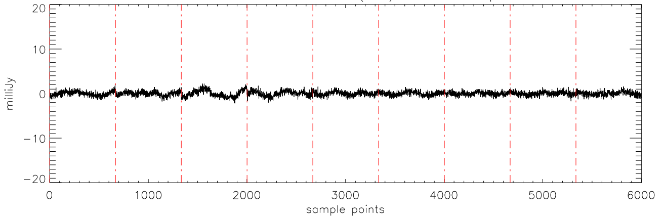
a2471 J03284265 17dec10 (AST) StokesU freq:5176.
