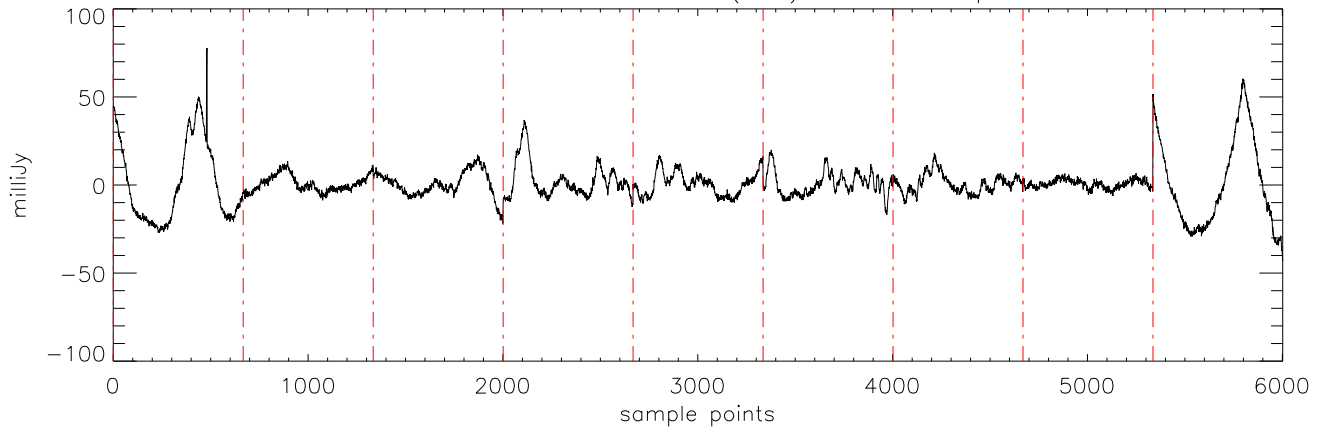
a2471 J03284265 17dec10 (AST) StokesI freq:5176.
