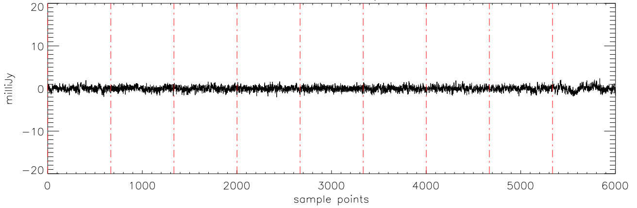
a2471 J03284265 17dec10 (AST) StokesV freq:5176.
