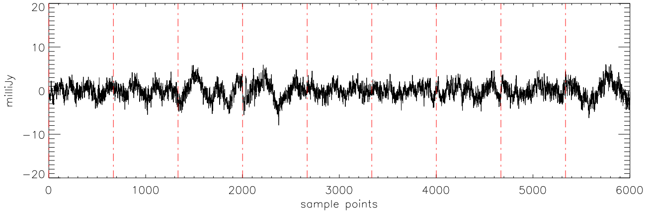
a2471 J03284265 17dec10 (AST) StokesQ freq:4750.
