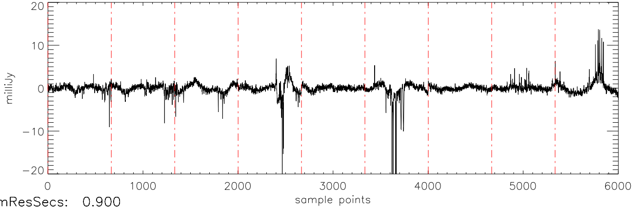
a2471 J03284265 17dec10 (AST) StokesU freq:4466.
