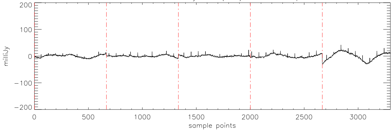
a2471 J03284265 09jan10 (AST) StokesI freq:5176.
