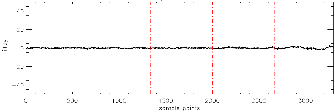
a2471 J03284265 09jan10 (AST) StokesU freq:4750.
