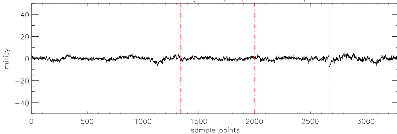
a2471 J03284265 09jan10 (AST) StokesQ freq:4608.
