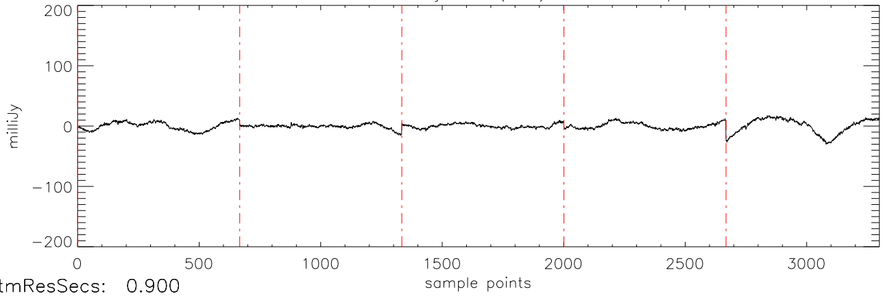
a2471 J03284265 09jan10 (AST) StokesI freq:5034.
