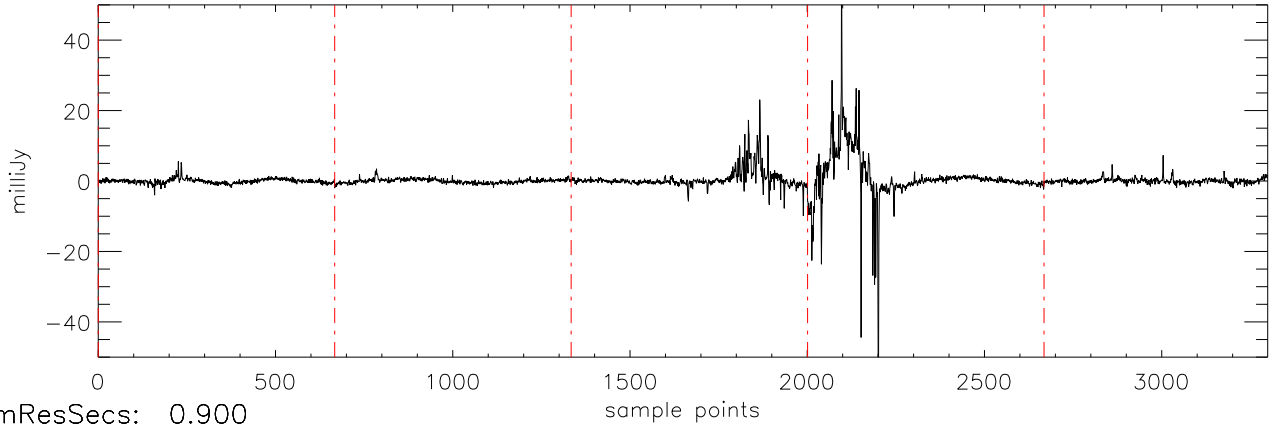
a2471 J03284265 09jan10 (AST) StokesU freq:4466.
