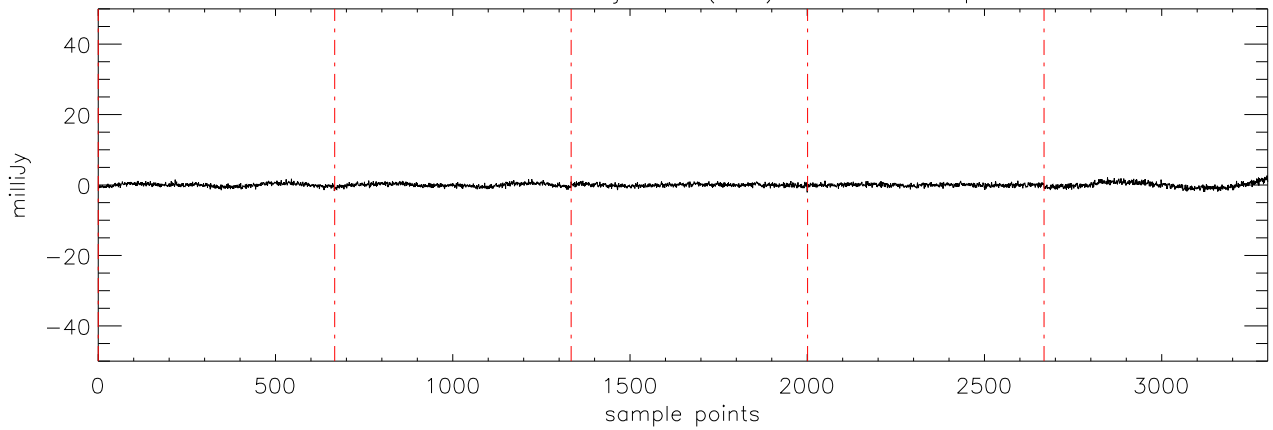
a2471 J03284265 09jan10 (AST) StokesU freq:4608.
