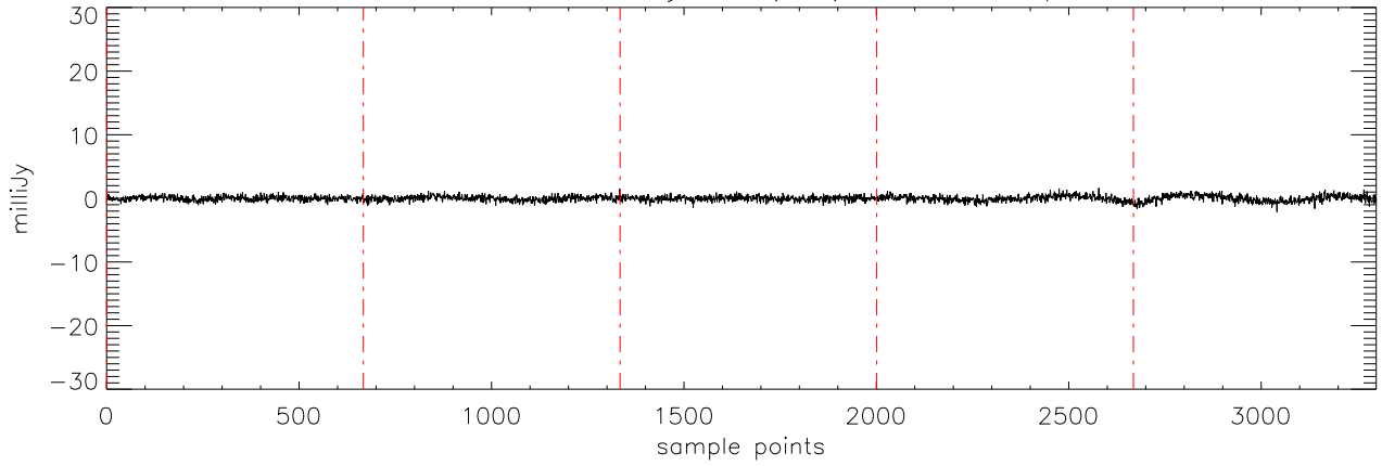
a2471 J03284265 09jan10 (AST) StokesV freq:4750.
