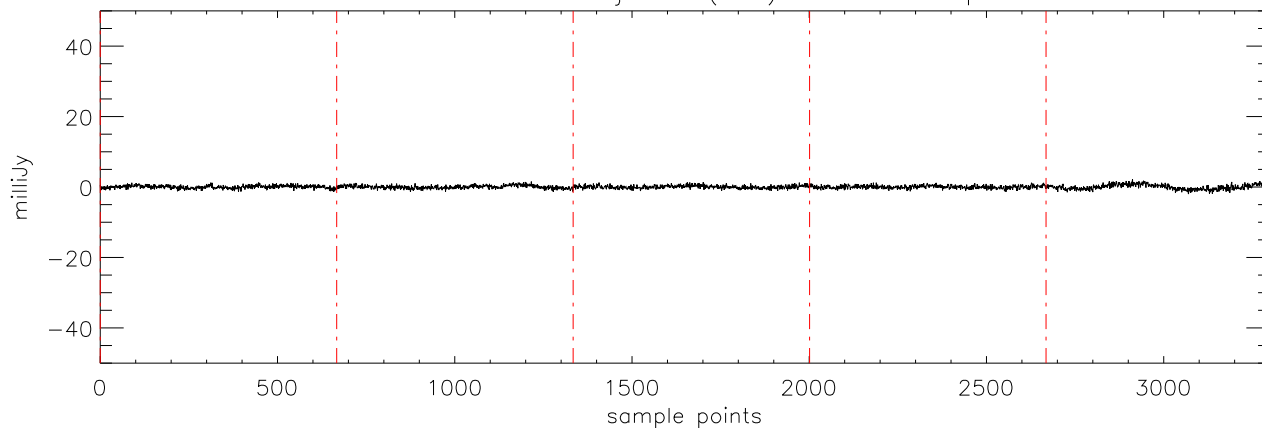
a2471 J03284265 09jan10 (AST) StokesU freq:5176.
