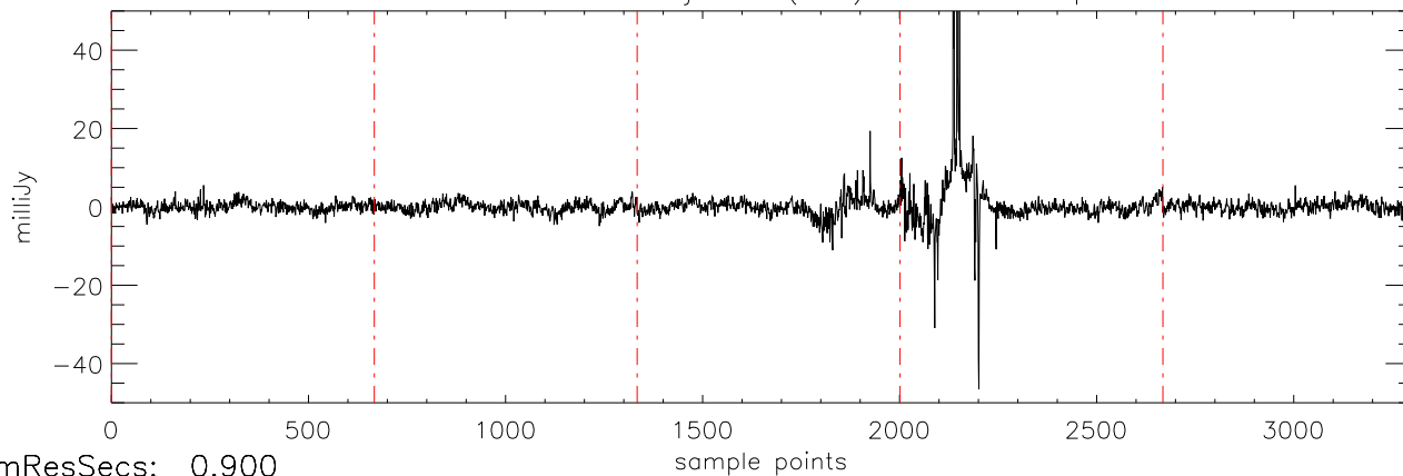
a2471 J03284265 09jan10 (AST) StokesQ freq:4466.
