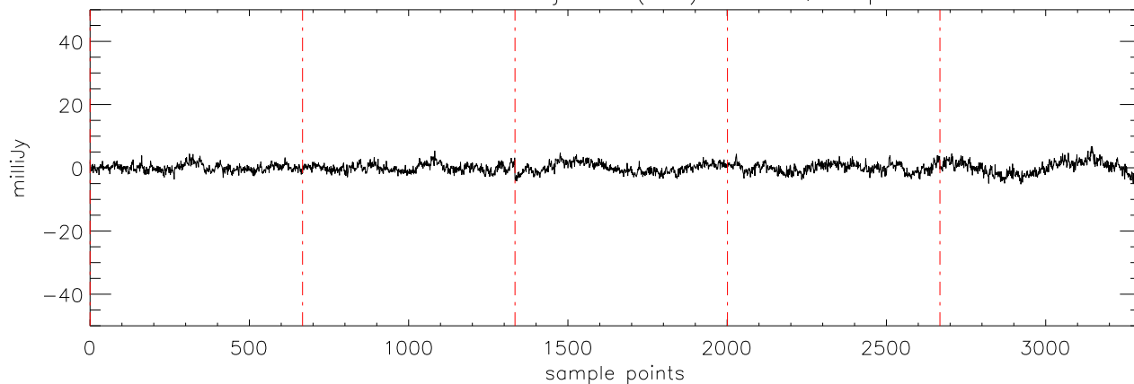
a2471 J03284265 09jan10 (AST) StokesQ freq:4750.
