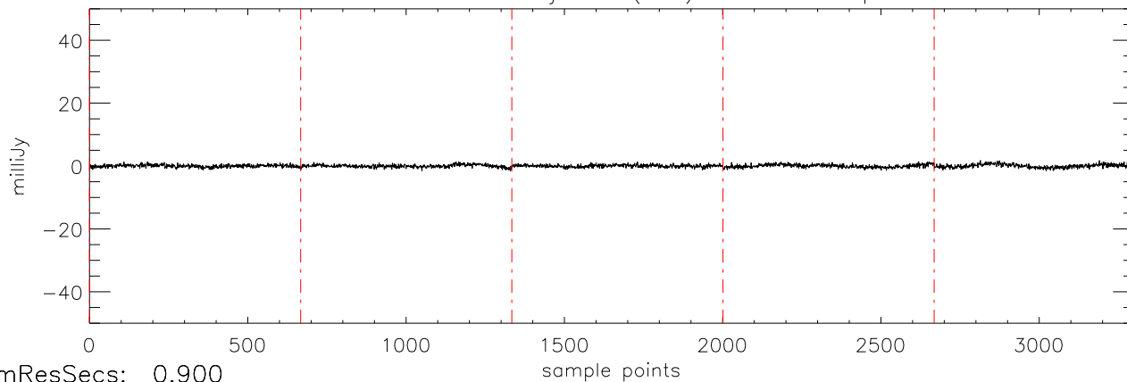
a2471 J03284265 09jan10 (AST) StokesU freq:5034.
