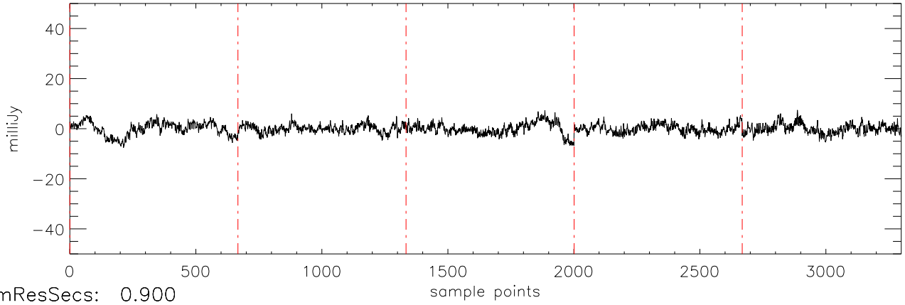
a2471 J03284265 09jan10 (AST) StokesQ freq:5034.
