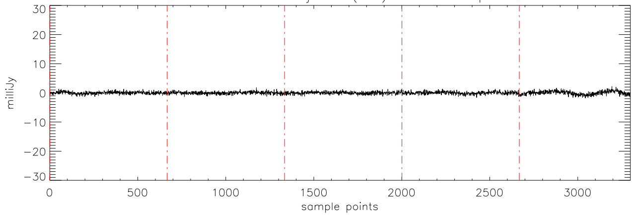
a2471 J03284265 09jan10 (AST) StokesV freq:5176.
