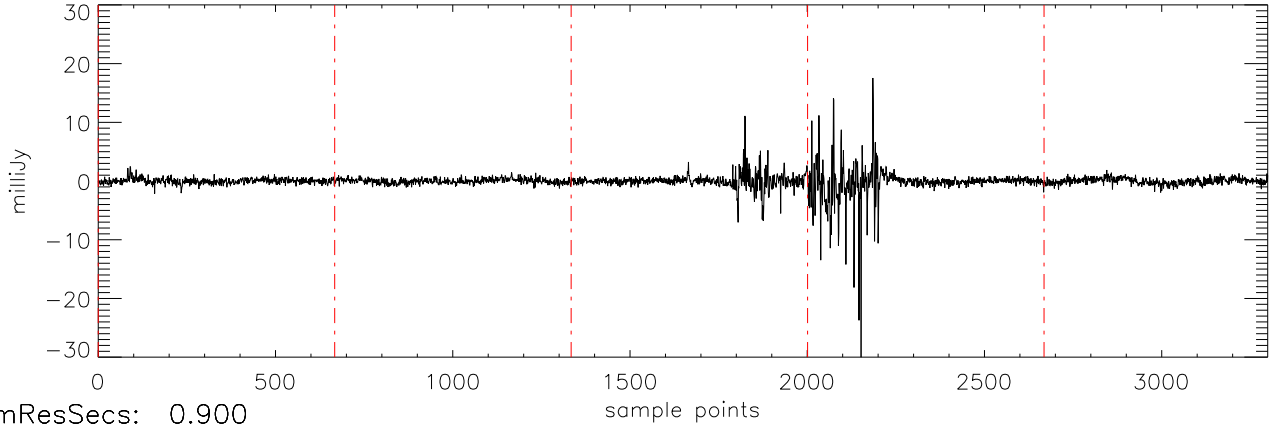
a2471 J03284265 09jan10 (AST) StokesV freq:4466.
