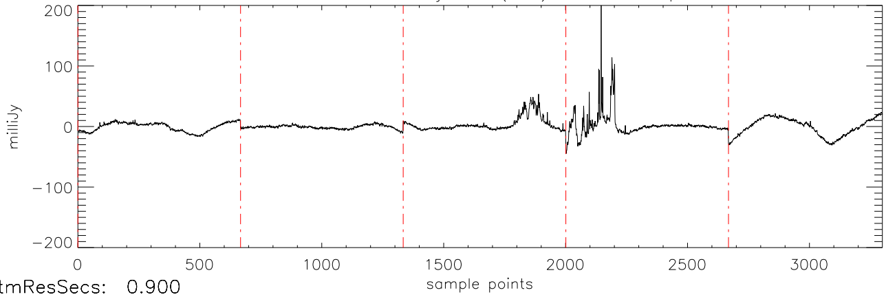
a2471 J03284265 09jan10 (AST) StokesI freq:4466.
