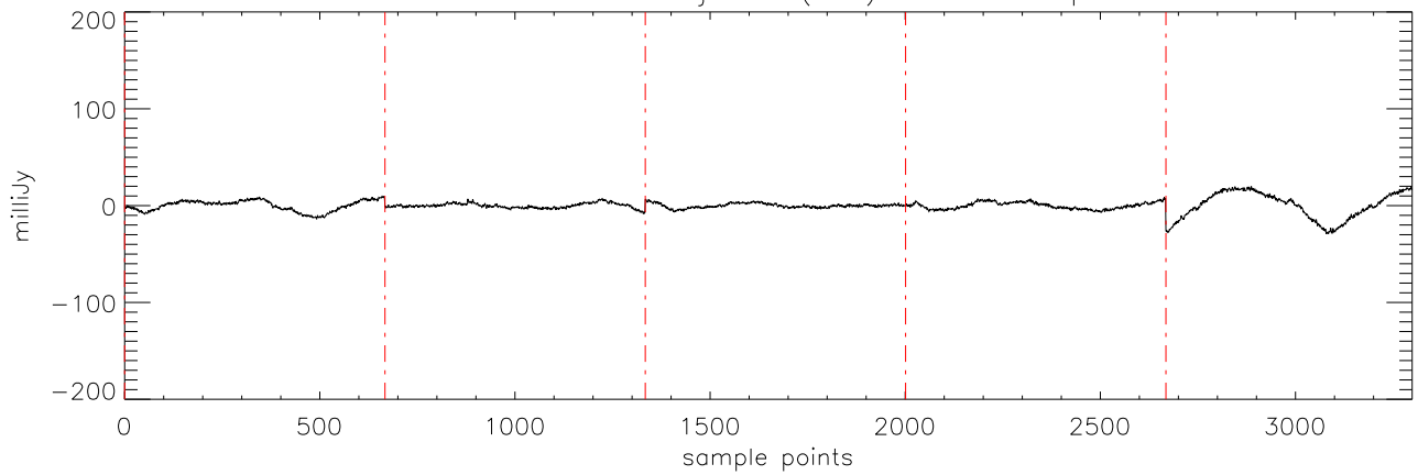
a2471 J03284265 09jan10 (AST) StokesI freq:4608.
