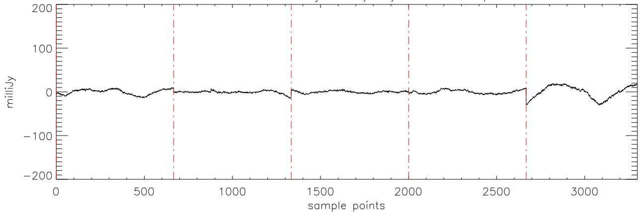
a2471 J03284265 09jan10 (AST) StokesI freq:4750.
