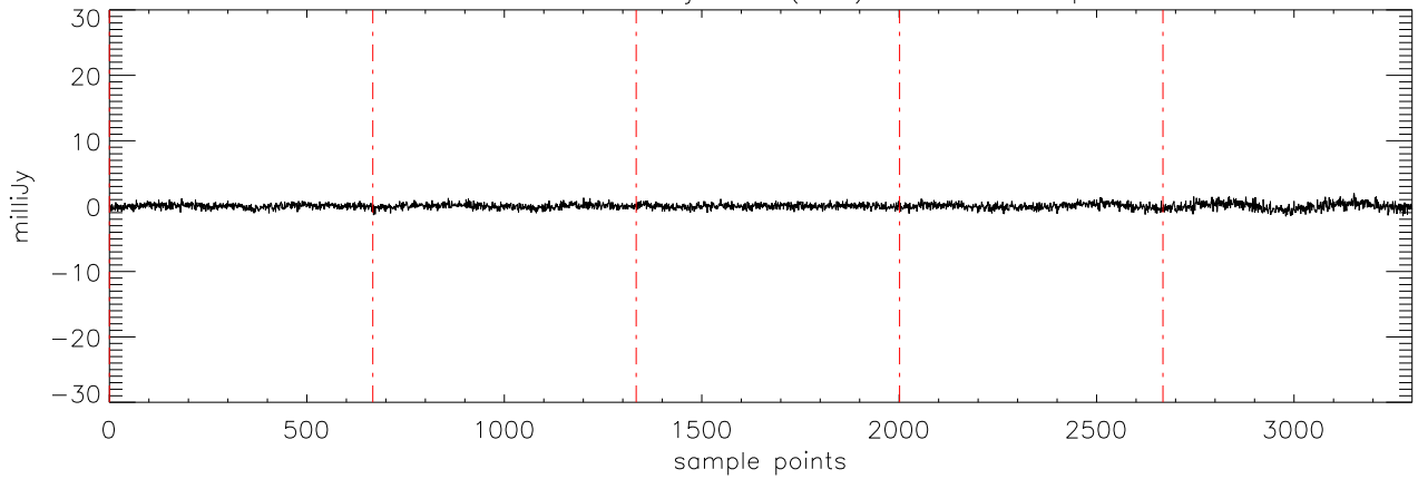
a2471 J03284265 09jan10 (AST) StokesV freq:4608.
