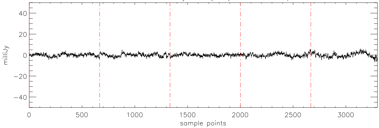
a2471 J03284265 09jan10 (AST) StokesQ freq:5176.
