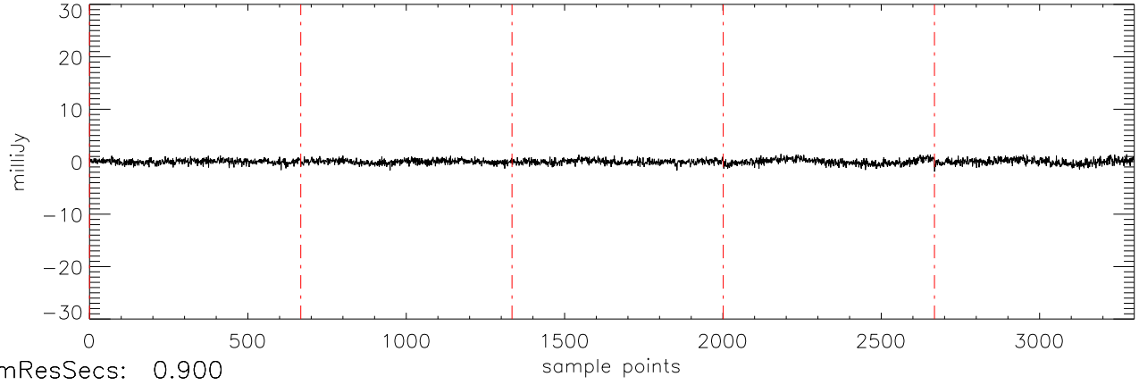
a2471 J03284265 09jan10 (AST) StokesV freq:5034.
