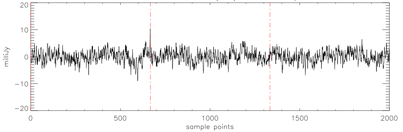
a2471 J0326137 19nov11 (AST) StokesQ freq:4750.
