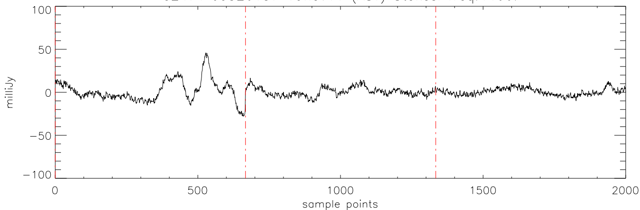
a2471 J0326137 19nov11 (AST) StokesI freq:4608.
