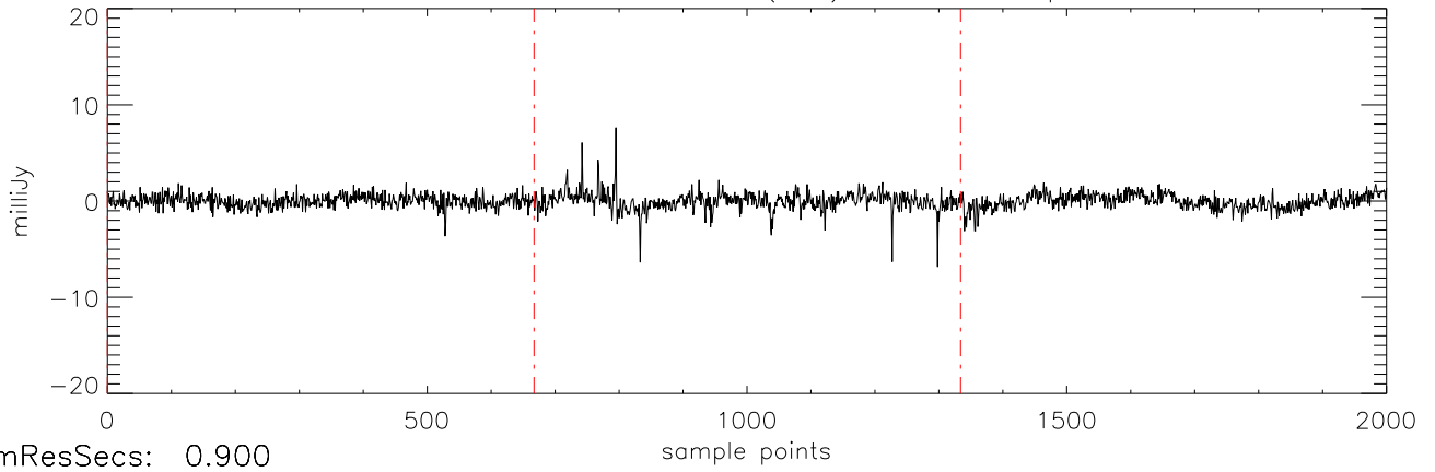
a2471 J0326137 19nov11 (AST) StokesU freq:4466.
