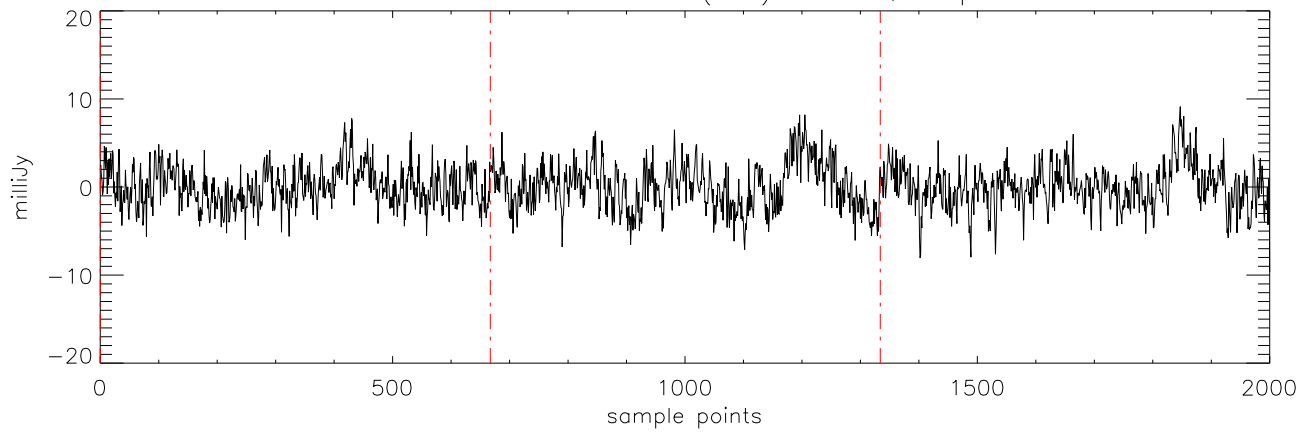
a2471 J0326137 19nov11 (AST) StokesQ freq:4608.
