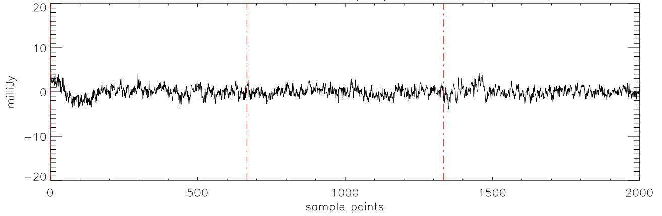
a2471 J0326137 19nov11 (AST) StokesU freq:5176.
