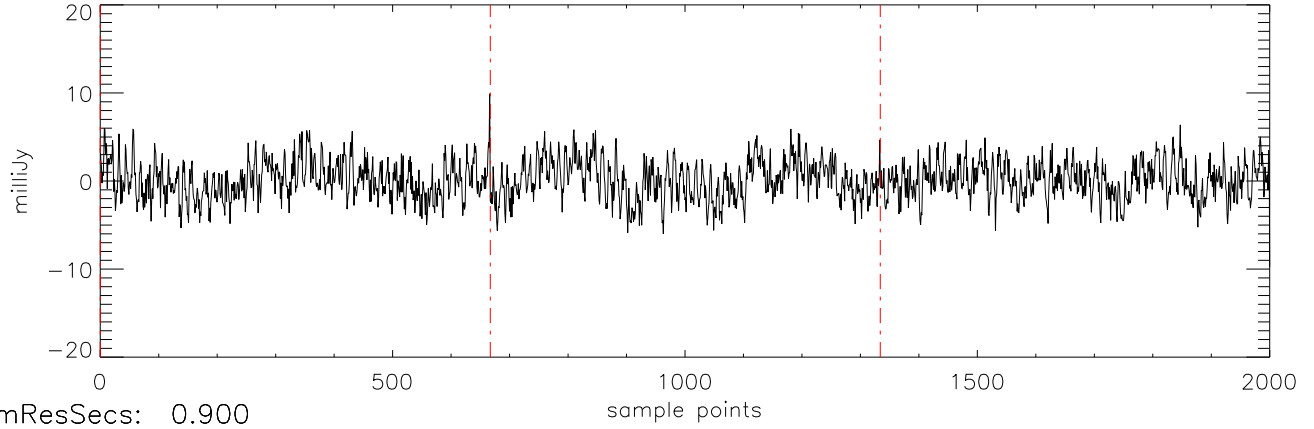
a2471 J0326137 19nov11 (AST) StokesQ freq:5034.
