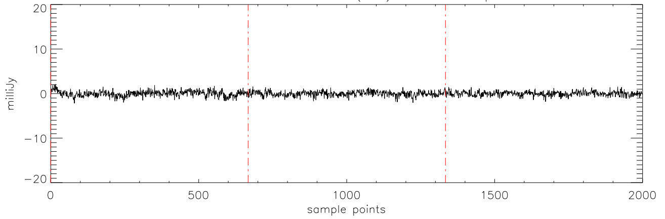
a2471 J0326137 19nov11 (AST) StokesV freq:5176.
