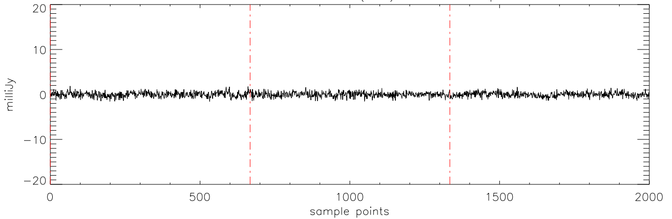
a2471 J0326137 19nov11 (AST) StokesV freq:4750.
