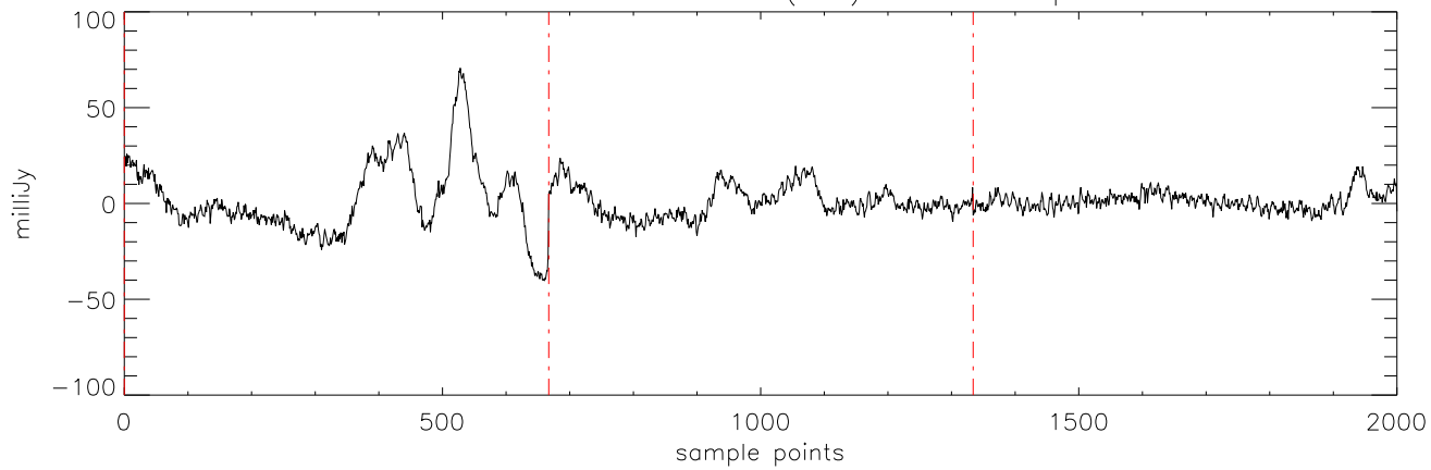
a2471 J0326137 19nov11 (AST) StokesI freq:5176.
