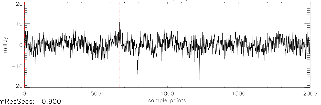
a2471 J0326137 19nov11 (AST) StokesQ freq:4466.
