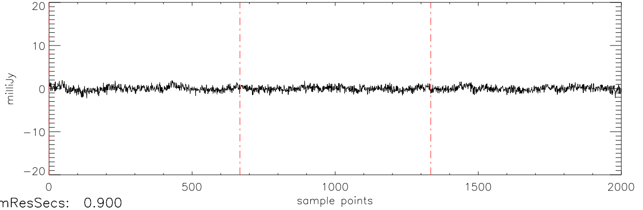
a2471 J0326137 19nov11 (AST) StokesU freq:5034.
