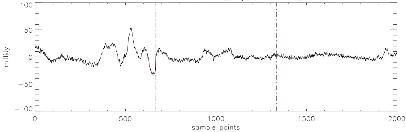
a2471 J0326137 19nov11 (AST) StokesI freq:4750.
