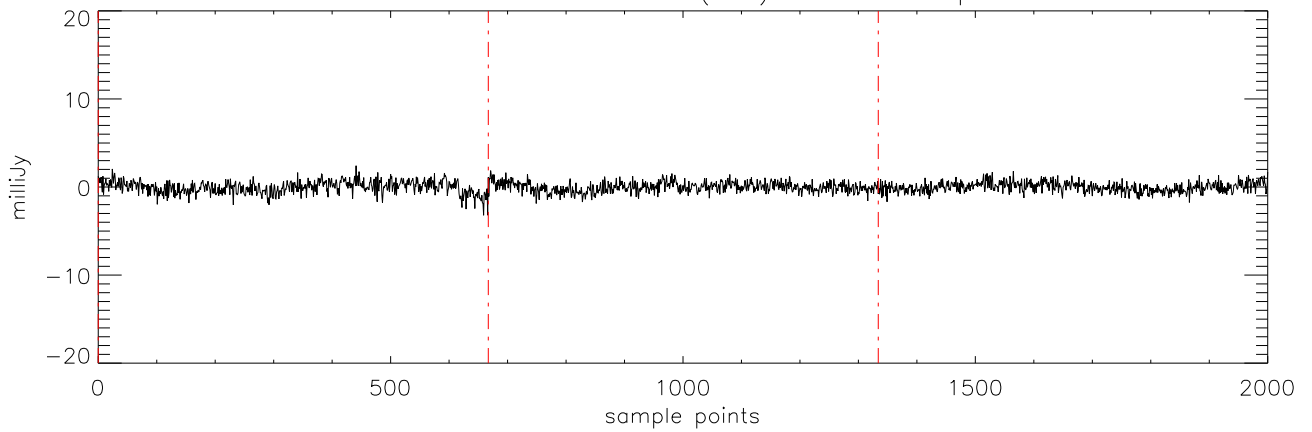
a2471 J0326137 19nov11 (AST) StokesU freq:4608.
