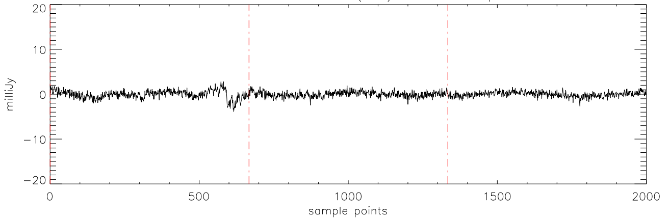
a2471 J0326137 19nov11 (AST) StokesU freq:4750.
