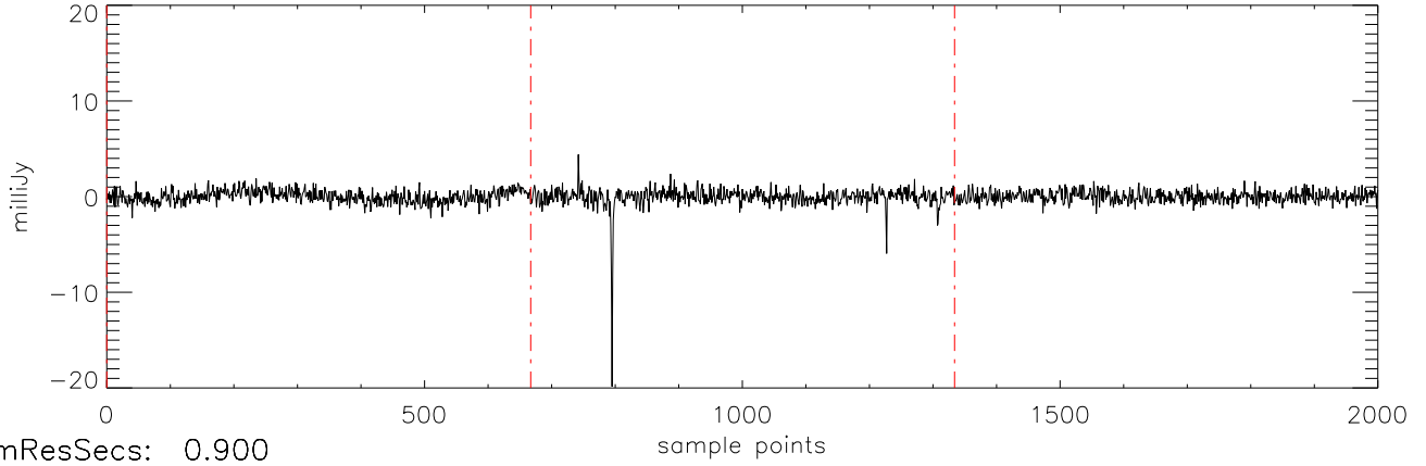
a2471 J0326137 19nov11 (AST) StokesV freq:4466.
