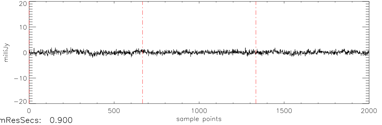
a2471 J0326137 19nov11 (AST) StokesV freq:5034.
