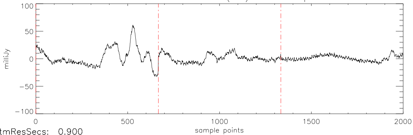
a2471 J0326137 19nov11 (AST) StokesI freq:5034.
