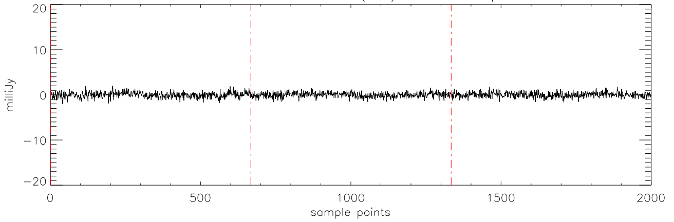
a2471 J0326137 19nov11 (AST) StokesV freq:4608.
