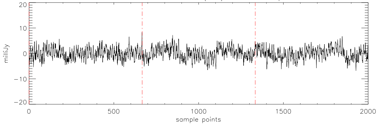
a2471 J0326137 19nov11 (AST) StokesQ freq:5176.
