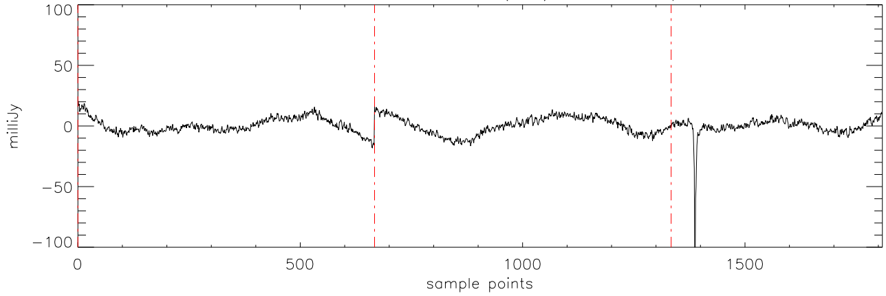
a2471 J01514155 18dec10 (AST) StokesI freq:5176.
