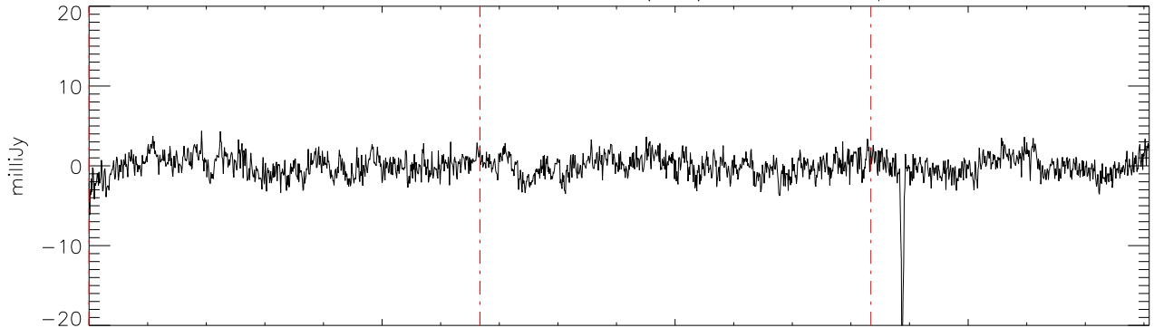
a2471 J01514155 18dec10 (AST) StokesQ freq:4608.
