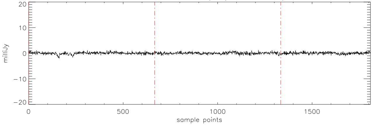
a2471 J01514155 18dec10 (AST) StokesV freq:4750.
