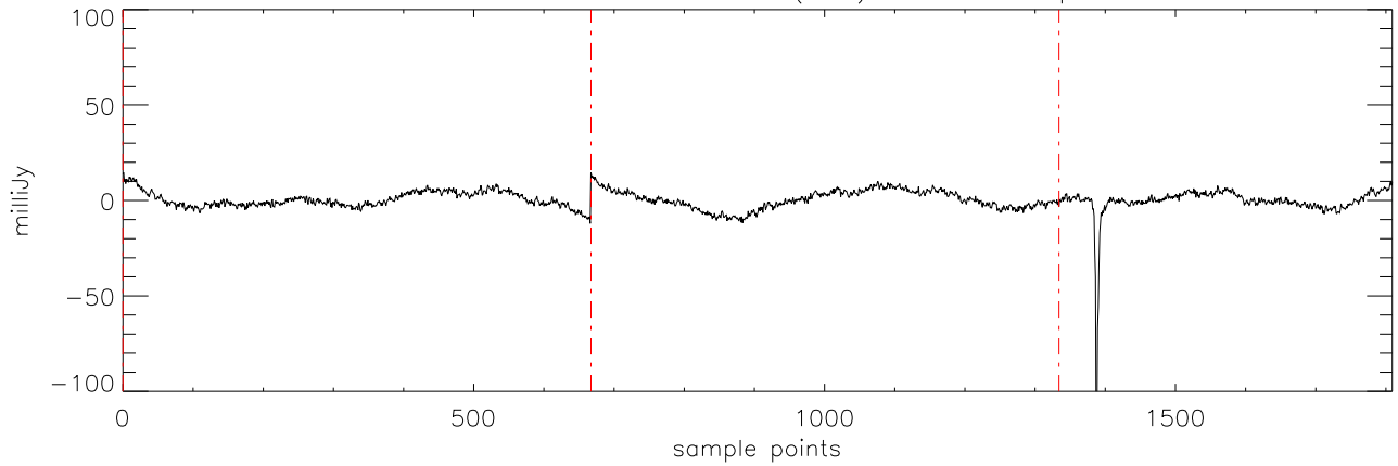
a2471 J01514155 18dec10 (AST) StokesI freq:4608.
