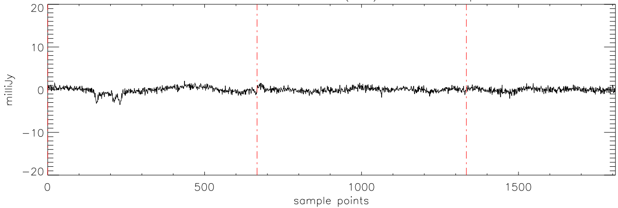
a2471 J01514155 18dec10 (AST) StokesU freq:4750.
