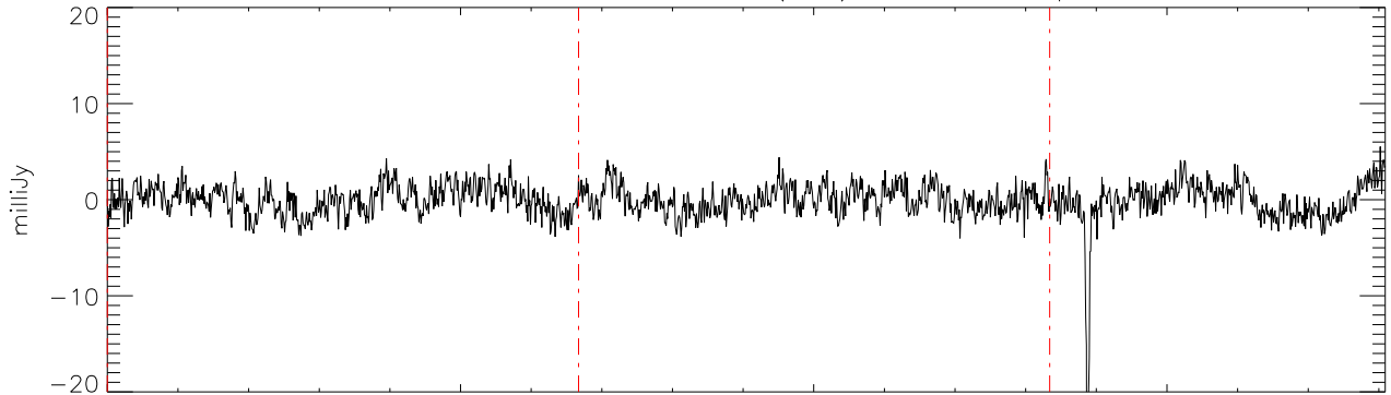
a2471 J01514155 18dec10 (AST) StokesQ freq:4750.
