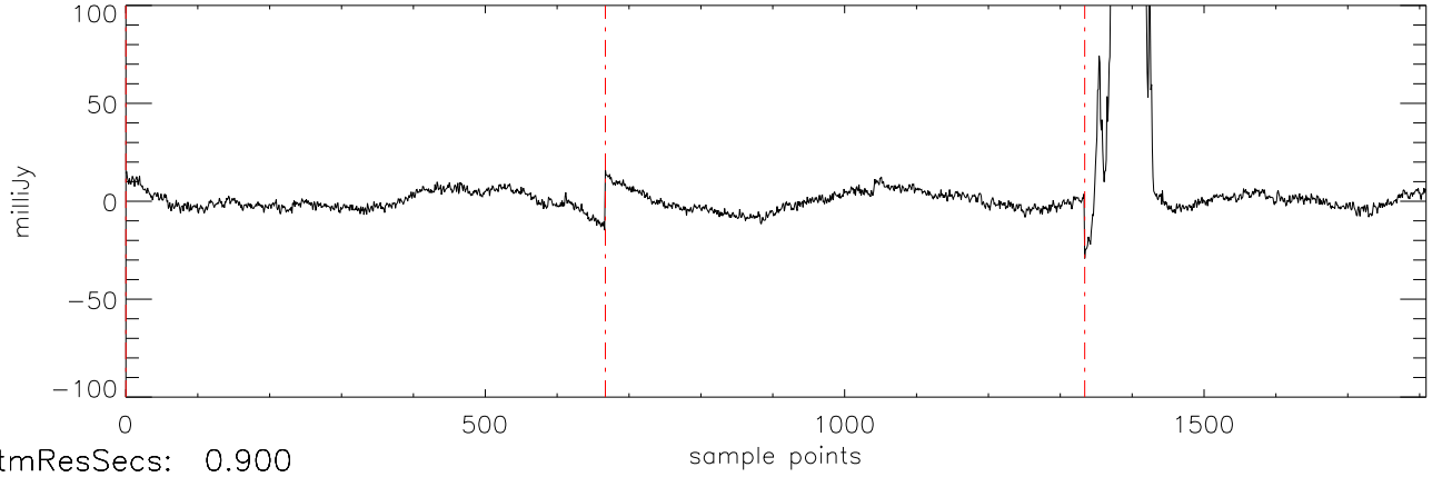
a2471 J01514155 18dec10 (AST) StokesI freq:4466.
