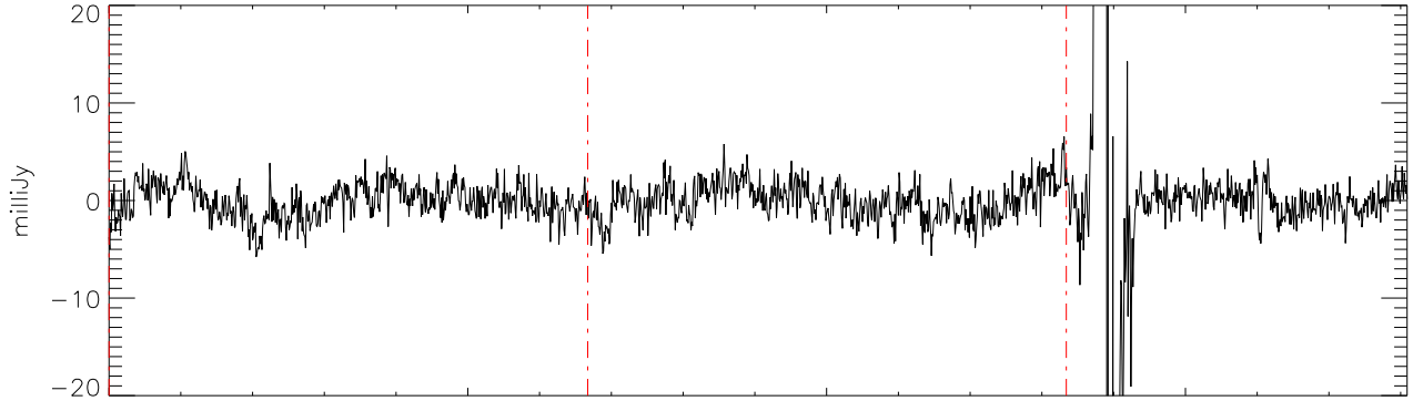
a2471 J01514155 18dec10 (AST) StokesQ freq:4325.
