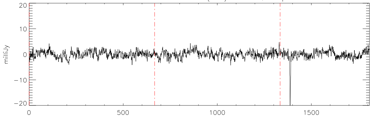
a2471 J01514155 18dec10 (AST) StokesQ freq:5034.
