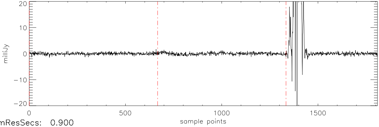
a2471 J01514155 18dec10 (AST) StokesV freq:4466.
