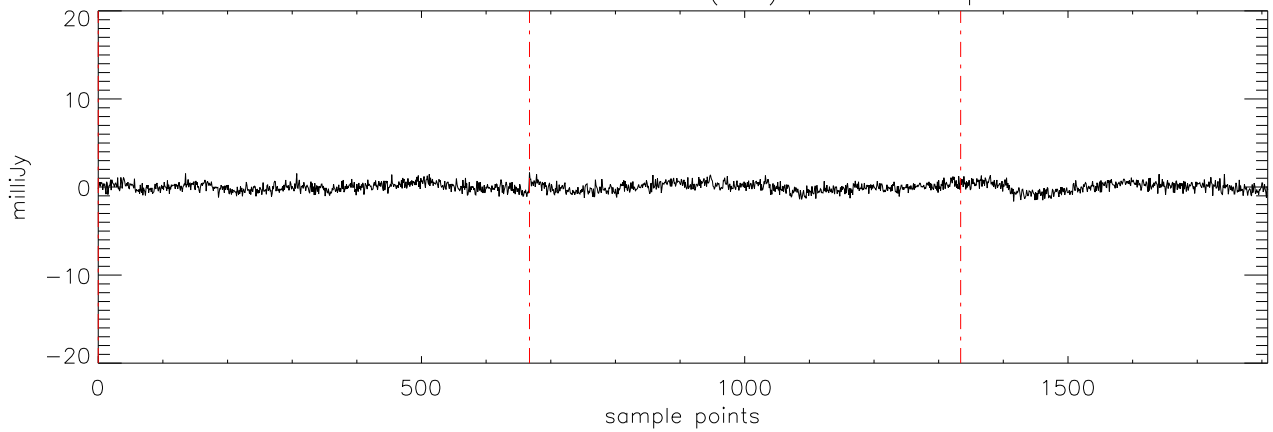
a2471 J01514155 18dec10 (AST) StokesU freq:4608.
