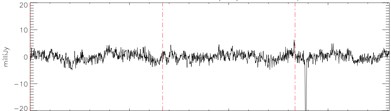
a2471 J01514155 18dec10 (AST) StokesQ freq:4466.
