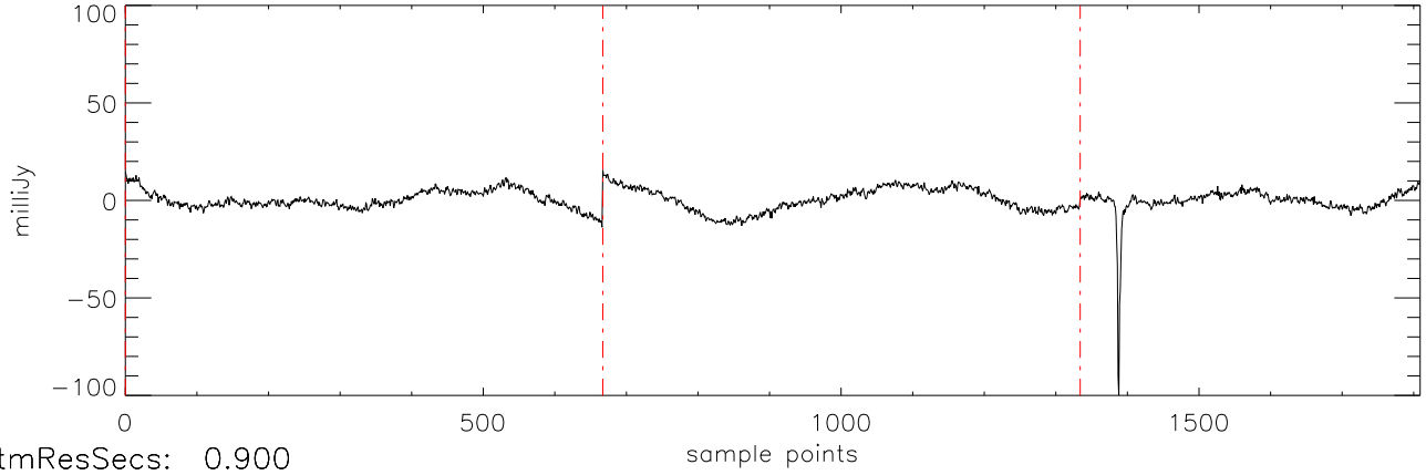
a2471 J01514155 18dec10 (AST) StokesI freq:5034.
