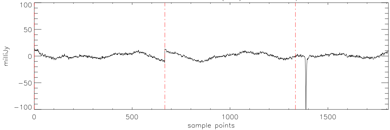
a2471 J01514155 18dec10 (AST) StokesI freq:4750.
