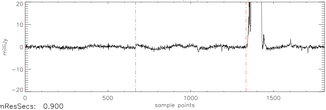
a2471 J01514155 18dec10 (AST) StokesU freq:4466.
