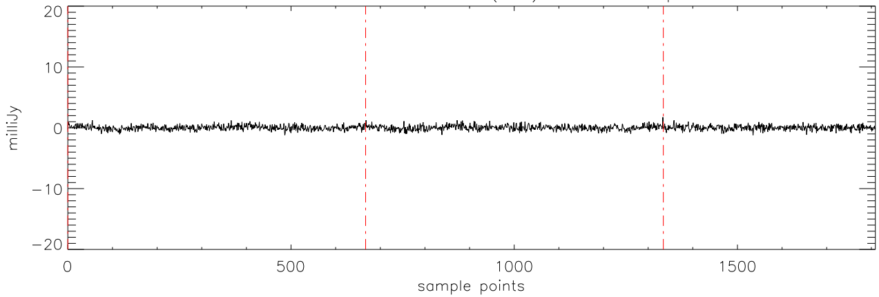
a2471 J01514155 18dec10 (AST) StokesV freq:4608.
