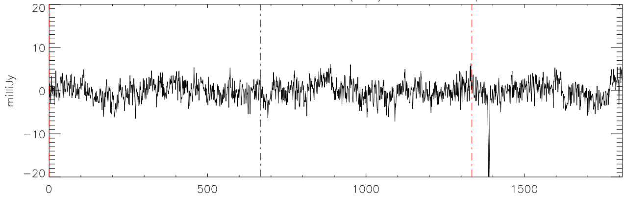
a2471 J01514155 18dec10 (AST) StokesQ freq:5176.
