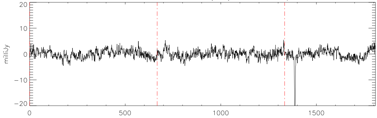
a2471 J01514155 18dec10 (AST) StokesQ freq:4892.
