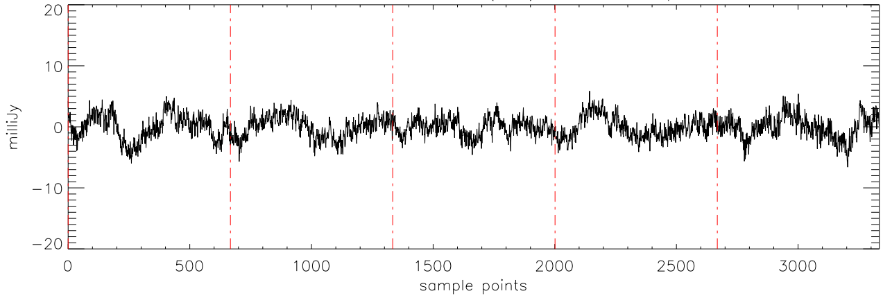
\alpha 2471 HD285968 18dec10 (AST) StokesQ freq:4750.
