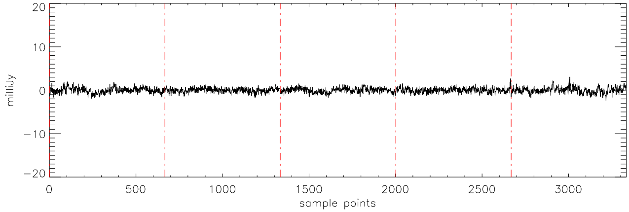
\alpha 2471 HD285968 18dec10 (AST) StokesU freq:5176.
