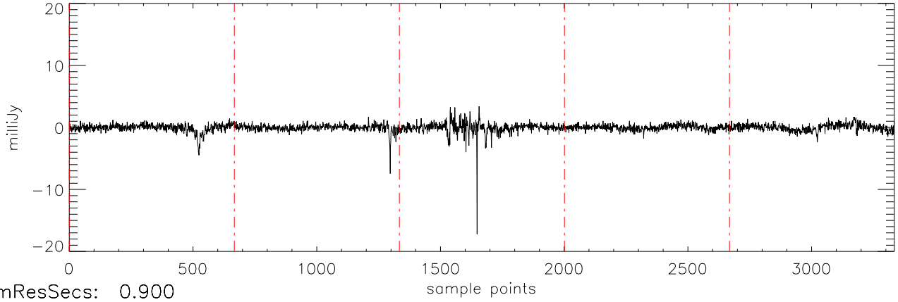
a2471 HD285968 18dec10 (AST) StokesV freq:4466.
