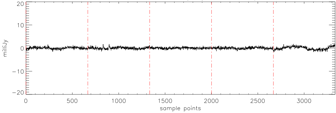
\alpha 2471 HD285968 18dec10 (AST) StokesU freq:4750.
