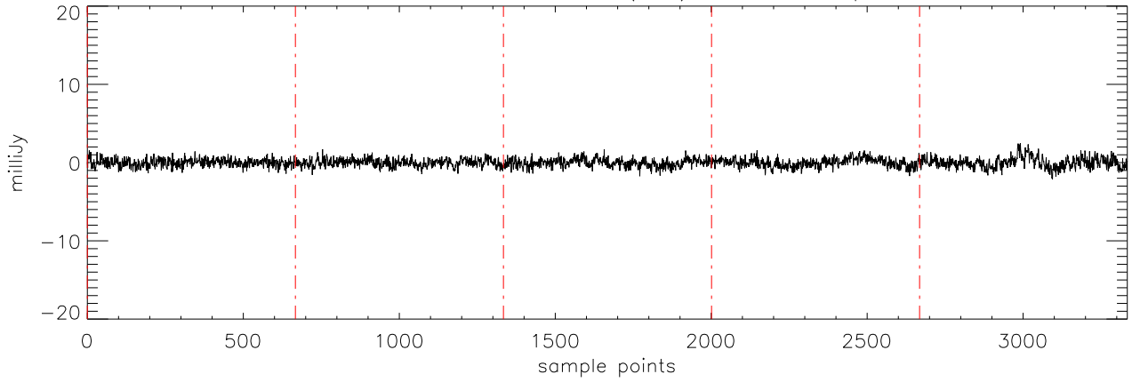
a2471 HD285968 18dec10 (AST) StokesV freq:5176.
