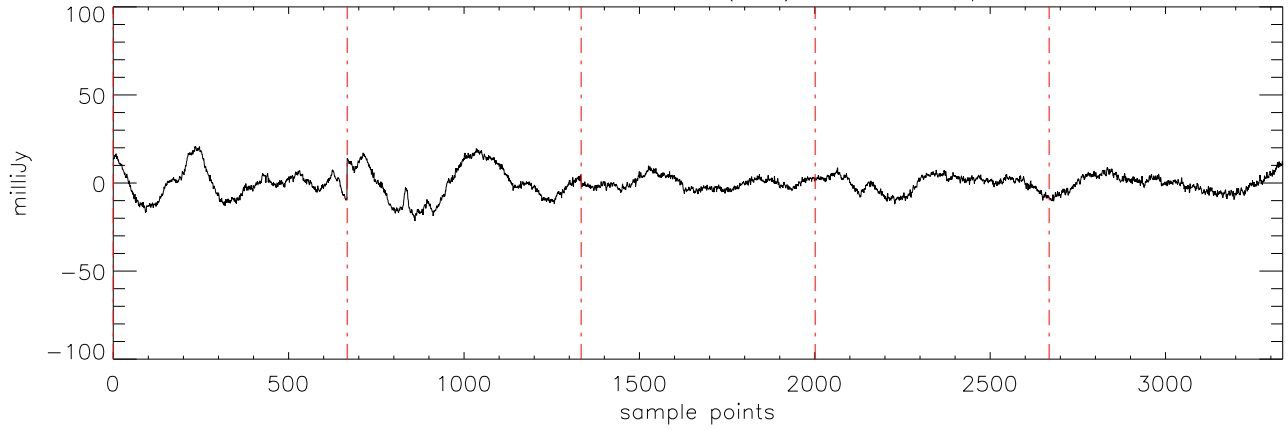
a2471 HD285968 18dec10 (AST) StokesI freq:4750.
