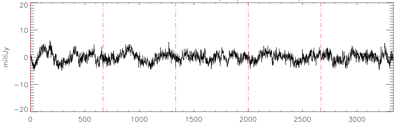
\alpha 2471 HD285968 18dec10 (AST) StokesQ freq:5034.
