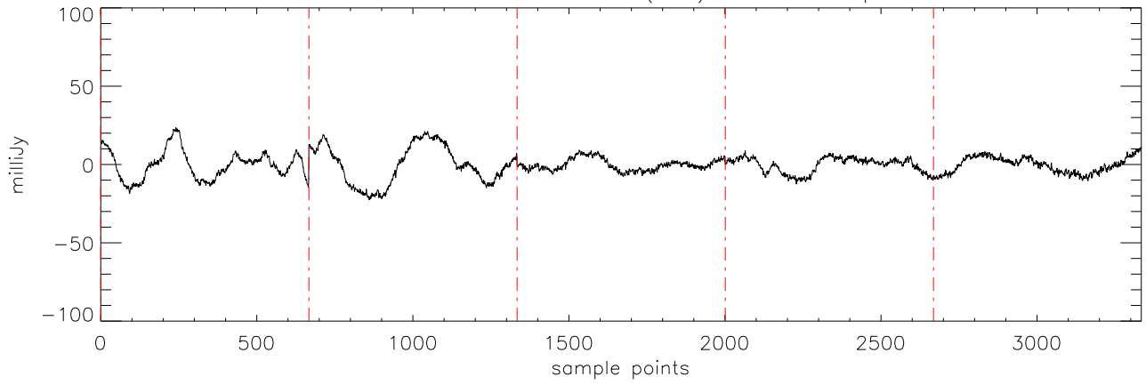
a2471 HD285968 18dec10 (AST) StokesI freq:5176.
