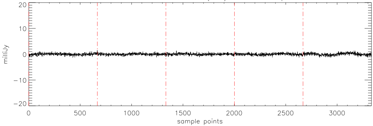
a2471 HD285968 18dec10 (AST) StokesV freq:4608.
