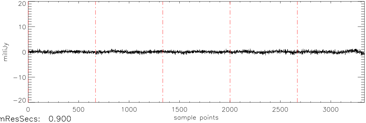
a2471 HD285968 18dec10 (AST) StokesV freq:5034.
