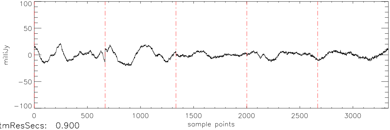
a2471 HD285968 18dec10 (AST) StokesI freq:5034.
