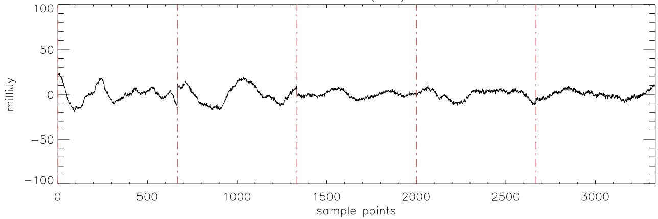
a2471 HD285968 18dec10 (AST) StokesI freq:4608.
