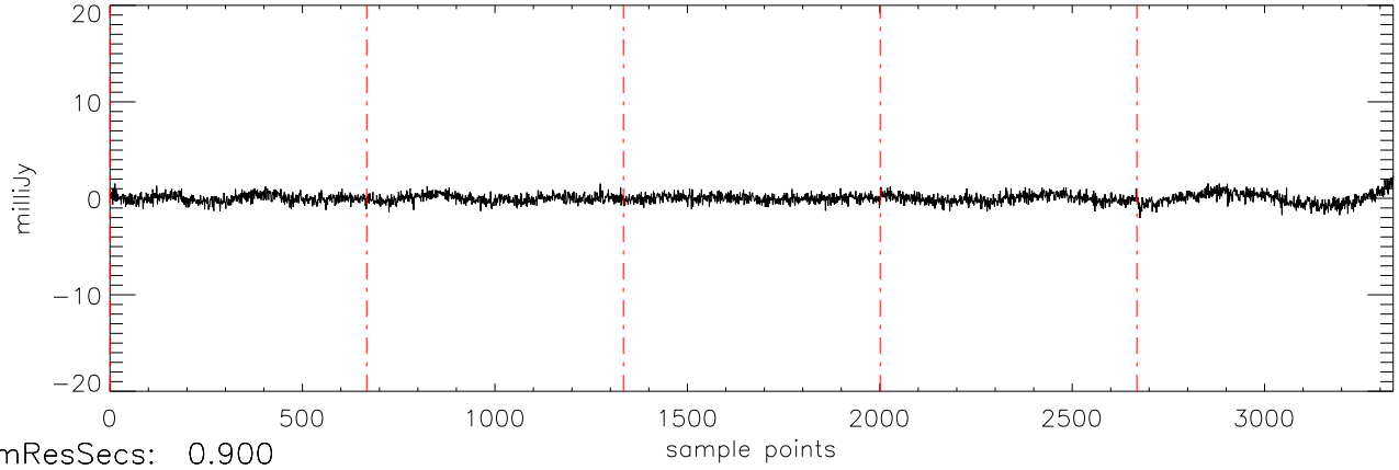
\alpha 2471 HD285968 18dec10 (AST) StokesU freq:5034.
