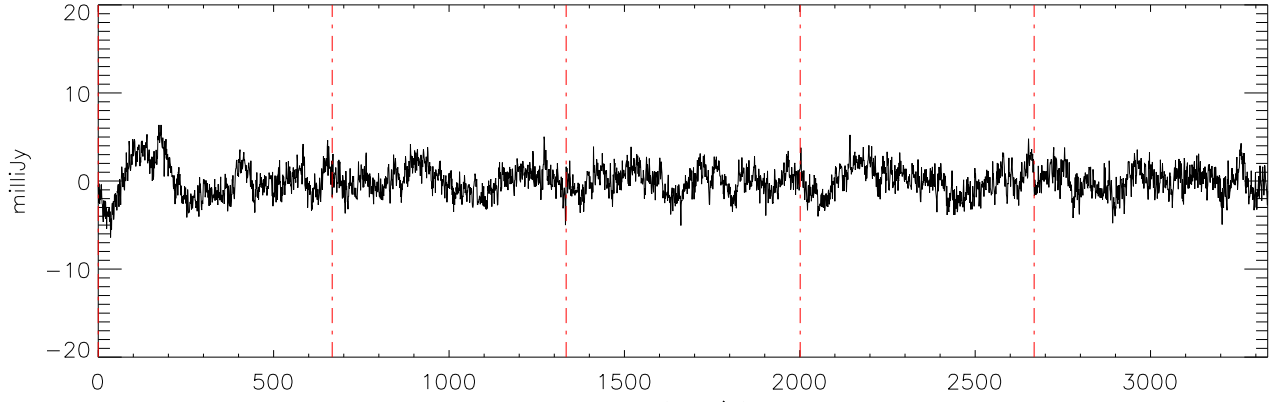
\alpha 2471 HD285968 18dec10 (AST) StokesQ freq:4892.
