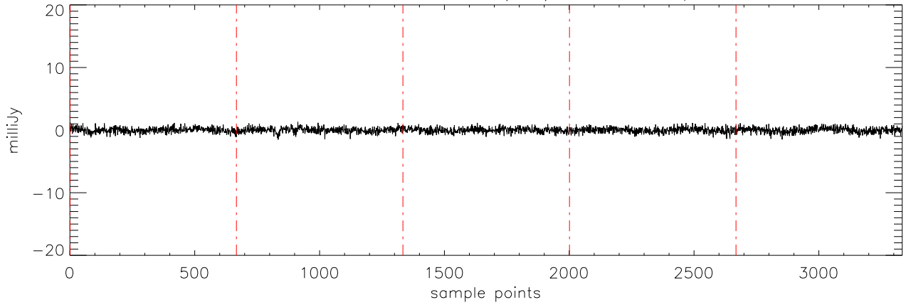
a2471 HD285968 18dec10 (AST) StokesV freq:4750.
