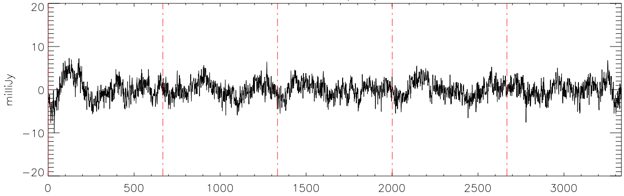
\alpha 2471 HD285968 18dec10 (AST) StokesQ freq:5176.
