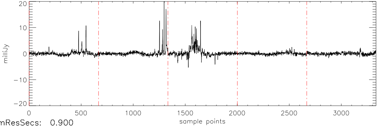
\alpha 2471 HD285968 18dec10 (AST) StokesU freq:4466.
