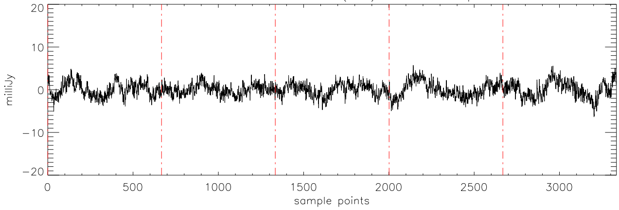
\alpha 2471 HD285968 18dec10 (AST) StokesQ freq:4608.
