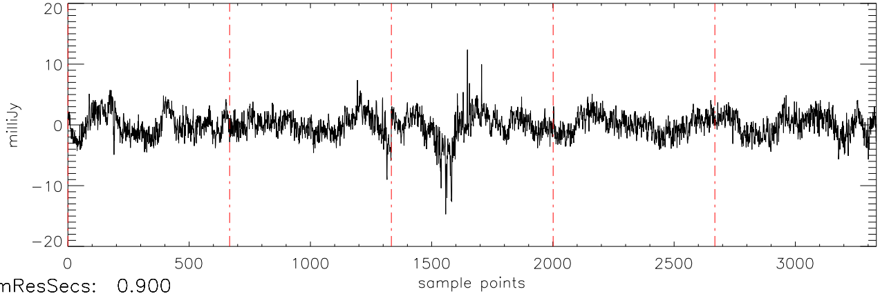
\alpha 2471 HD285968 18dec10 (AST) StokesQ freq:4466.
