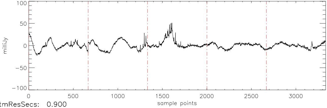
a2471 HD285968 18dec10 (AST) StokesI freq:4466.
