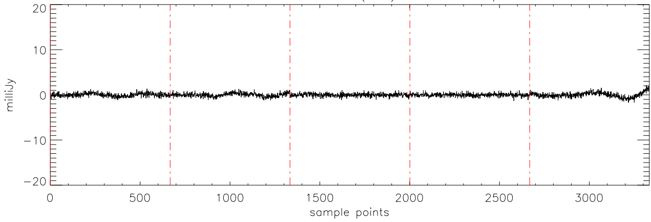
\alpha 2471 HD285968 18dec10 (AST) StokesU freq:4608.
