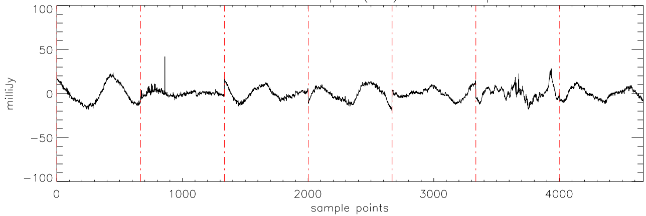
a2471 HD209458 06sep11 (AST) StokesI freq:4608.
