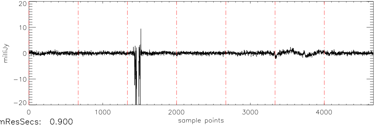
\alpha 2471 HD209458 06sep11 (AST) StokesV freq:4466.
