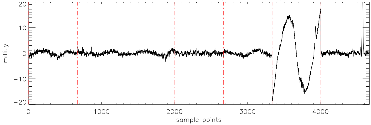
α2471 HD209458 06sep11 (AST) StokesU freq:4750.
