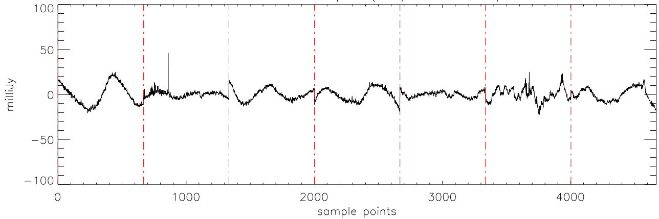
a2471 HD209458 06sep11 (AST) StokesI freq:4750.
