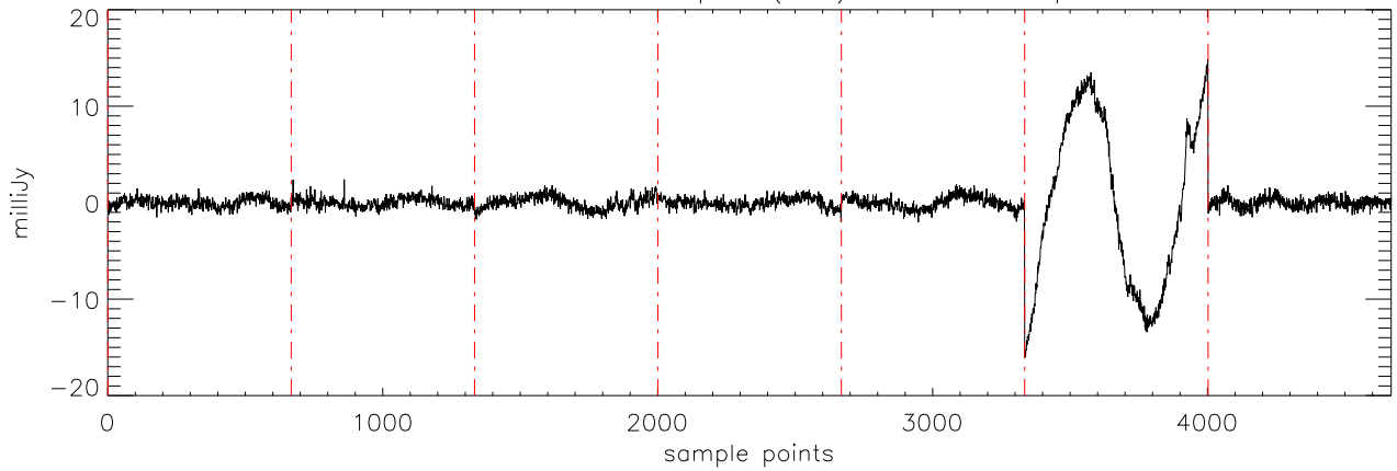
α2471 HD209458 06sep11 (AST) StokesU freq:4608.
