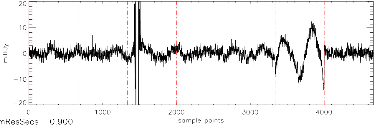
α2471 HD209458 06sep11 (AST) StokesQ freq:4466.
