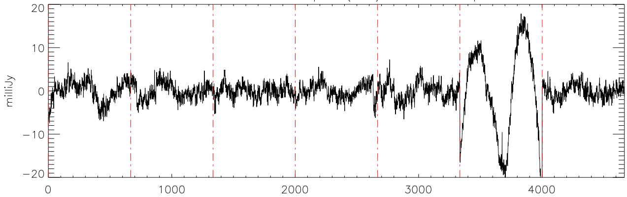
α2471 HD209458 06sep11 (AST) StokesQ freq:5034.
