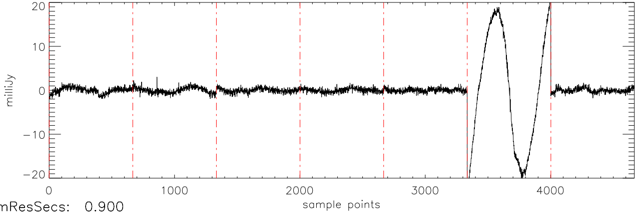
a2471 HD209458 06sep11 (AST) StokesU freq:5034.
