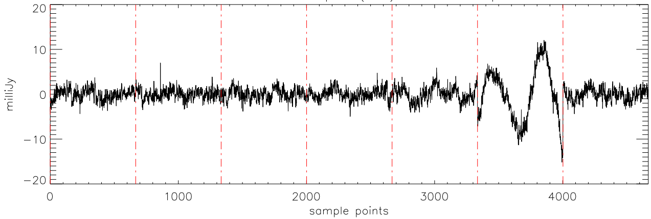
α2471 HD209458 06sep11 (AST) StokesQ freq:4608.
