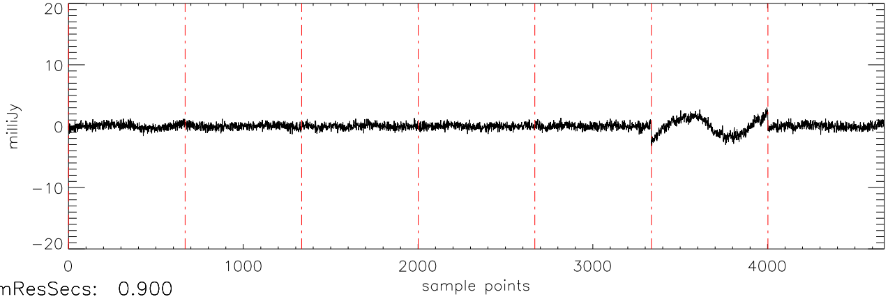
\alpha 2471 HD209458 06sep11 (AST) StokesV freq:5034.
