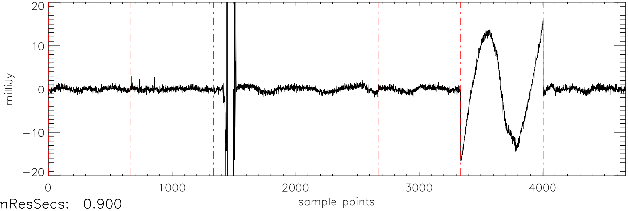
α2471 HD209458 06sep11 (AST) StokesU freq:4466.
