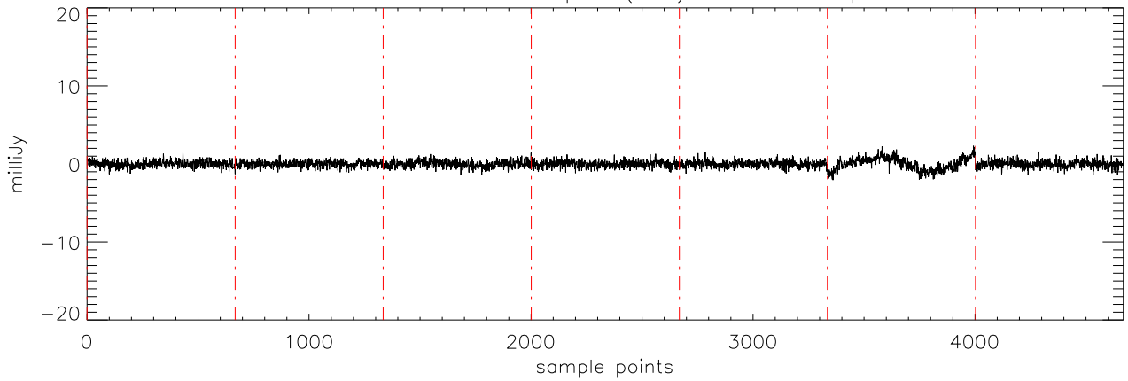
\alpha 2471 HD209458 06sep11 (AST) StokesV freq:4608.
