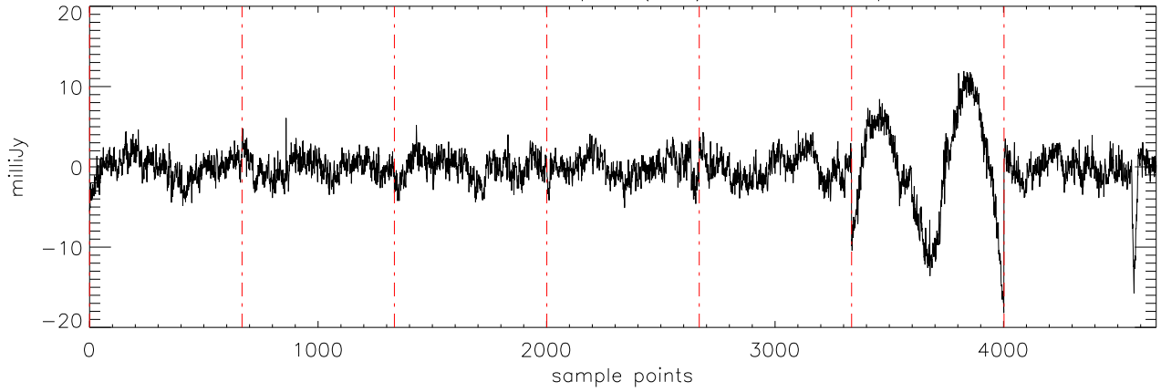
α2471 HD209458 06sep11 (AST) StokesQ freq:4750.
