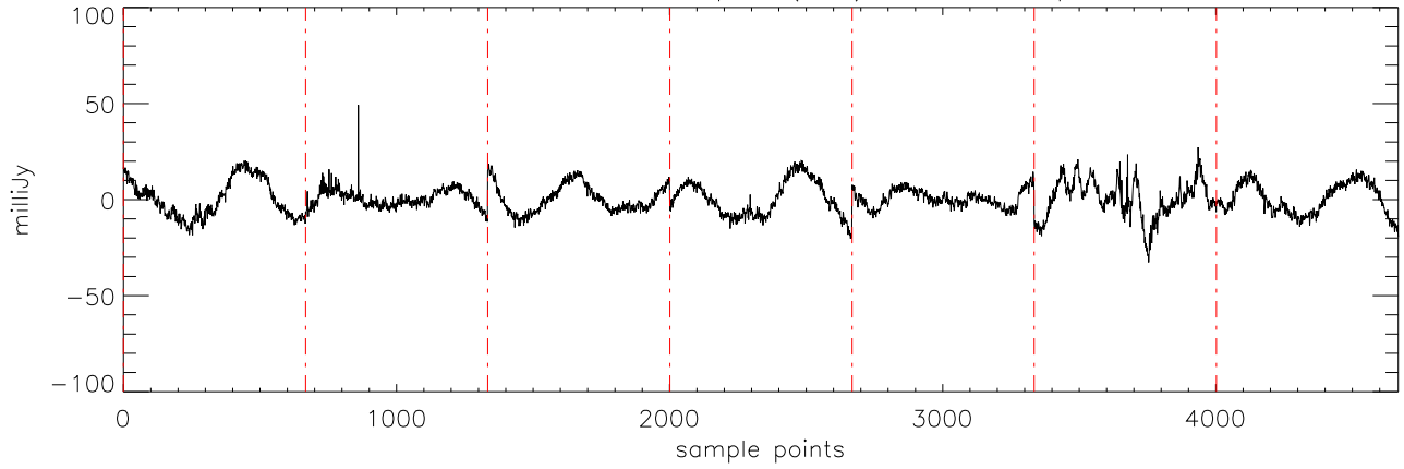
a2471 HD209458 06sep11 (AST) StokesI freq:5176.
