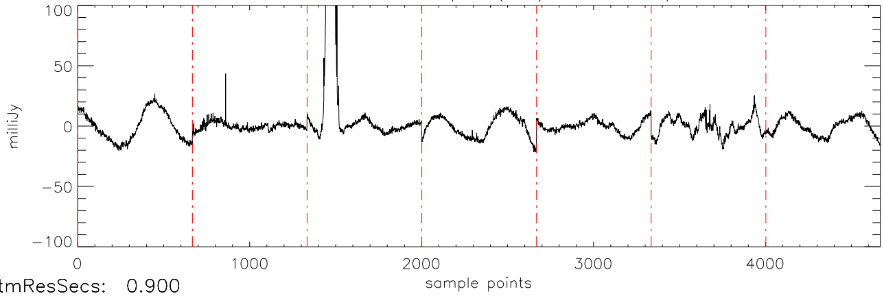
a2471 HD209458 06sep11 (AST) StokesI freq:4466.
