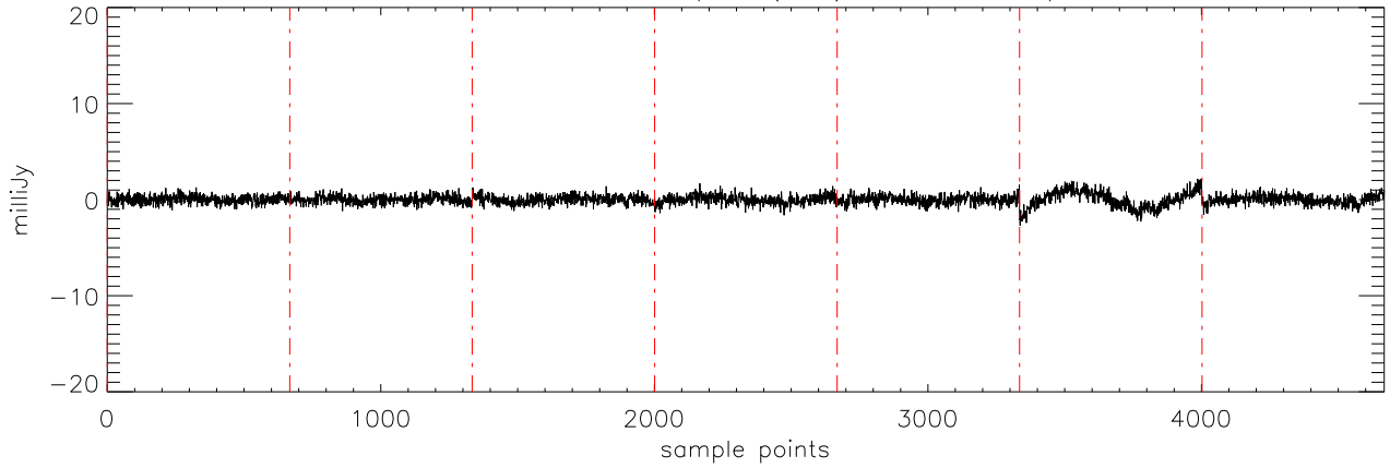
\alpha 2471 HD209458 06sep11 (AST) StokesV freq:4750.
