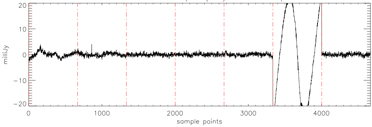
a2471 HD209458 06sep11 (AST) StokesU freq:5176.
