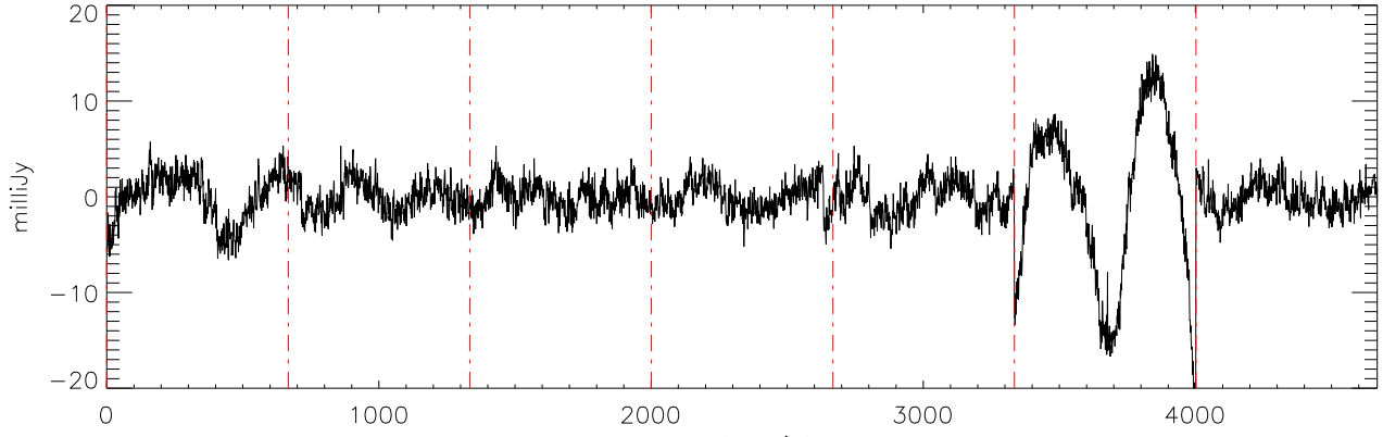
α2471 HD209458 06sep11 (AST) StokesQ freq:4892.
