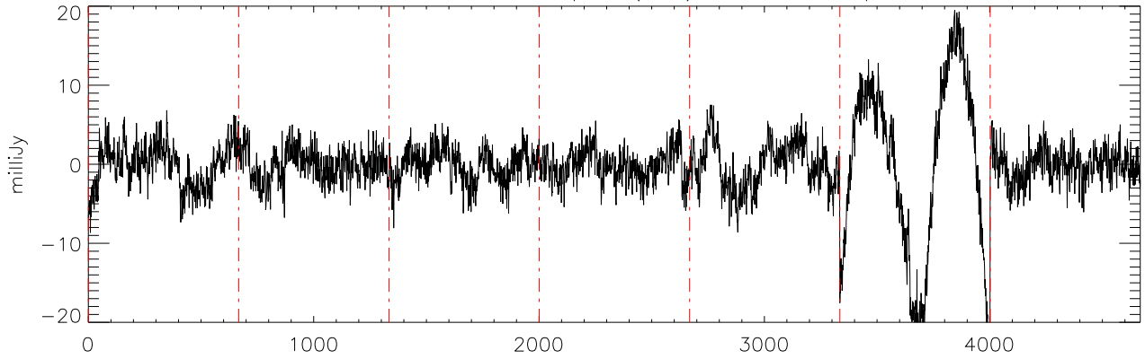
α2471 HD209458 06sep11 (AST) StokesQ freq:5176.
