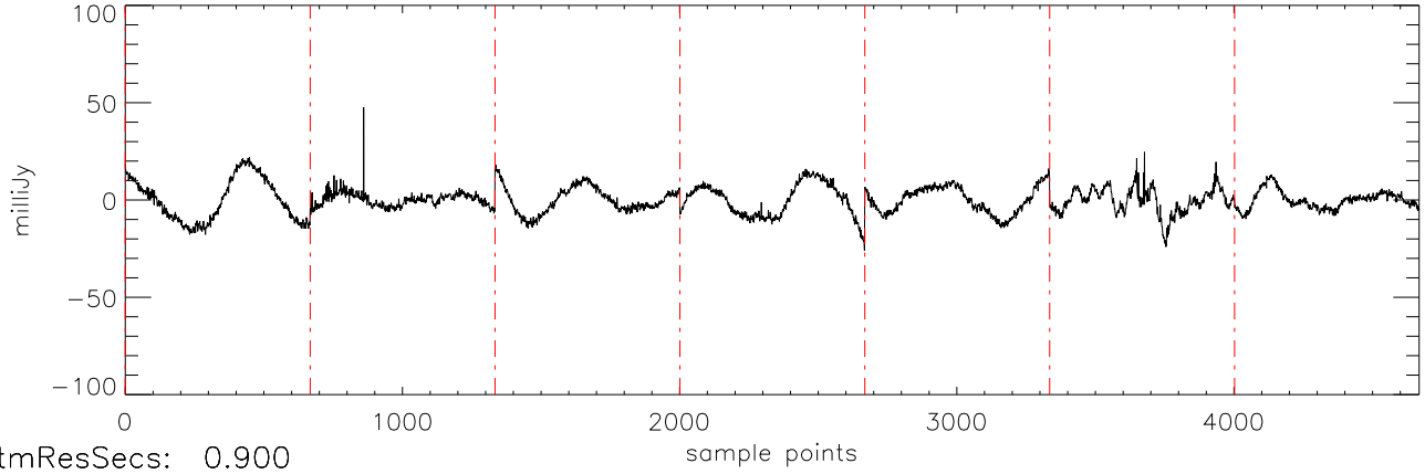
a2471 HD209458 06sep11 (AST) StokesI freq:5034.
