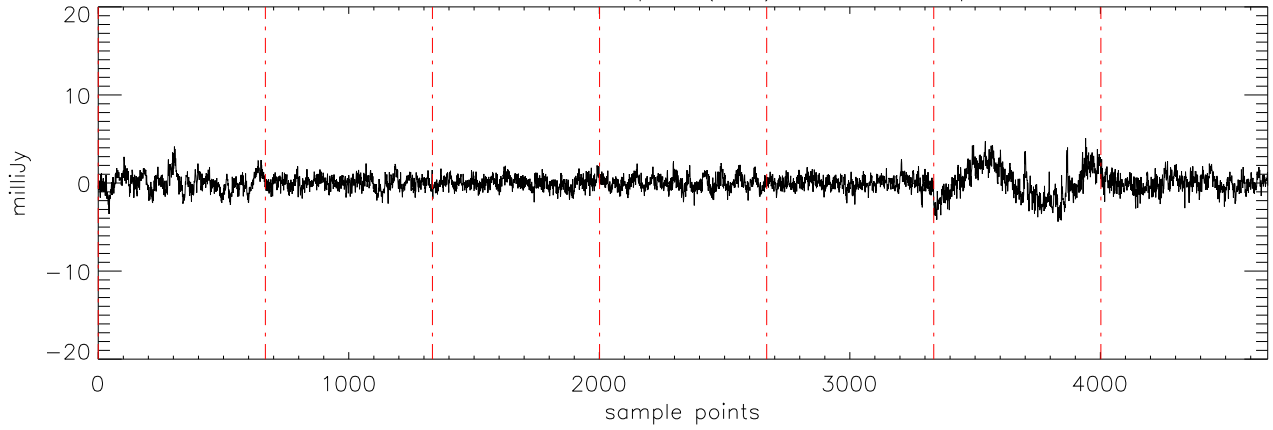
\alpha 2471 HD209458 06sep11 (AST) StokesV freq:5176.
