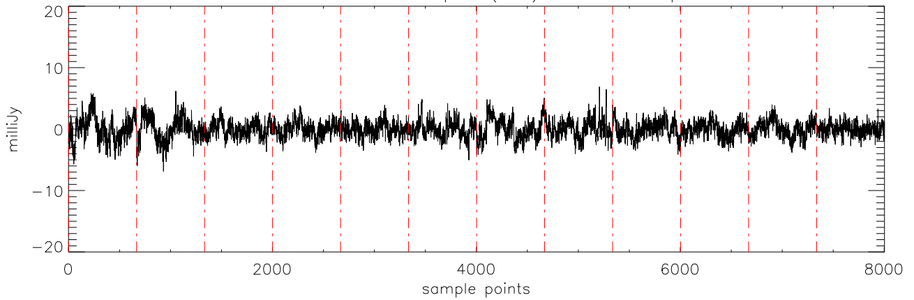
a2471 HD189733 06sep11 (AST) StokesQ freq:4608.
