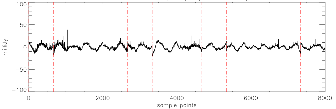
a2471 HD189733 06sep11 (AST) StokesI freq:4750.
