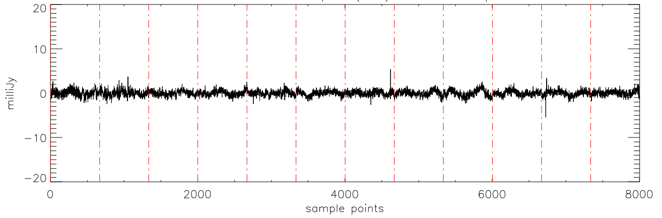
a2471 HD189733 06sep11 (AST) StokesU freq:5176.
