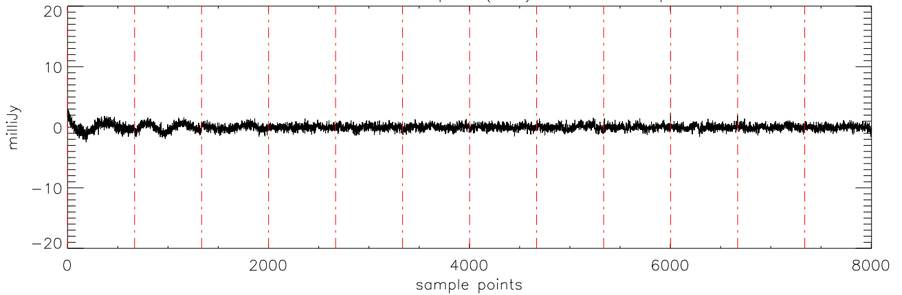
\alpha 2471 HD189733 06sep11 (AST) StokesV freq:4750.
