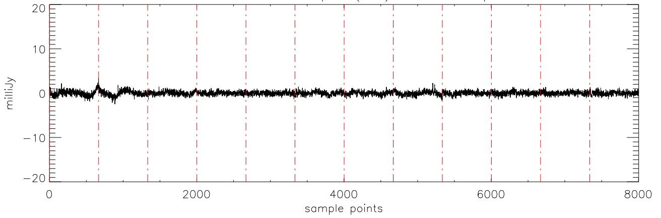
\alpha 2471 HD189733 06sep11 (AST) StokesV freq:4608.
