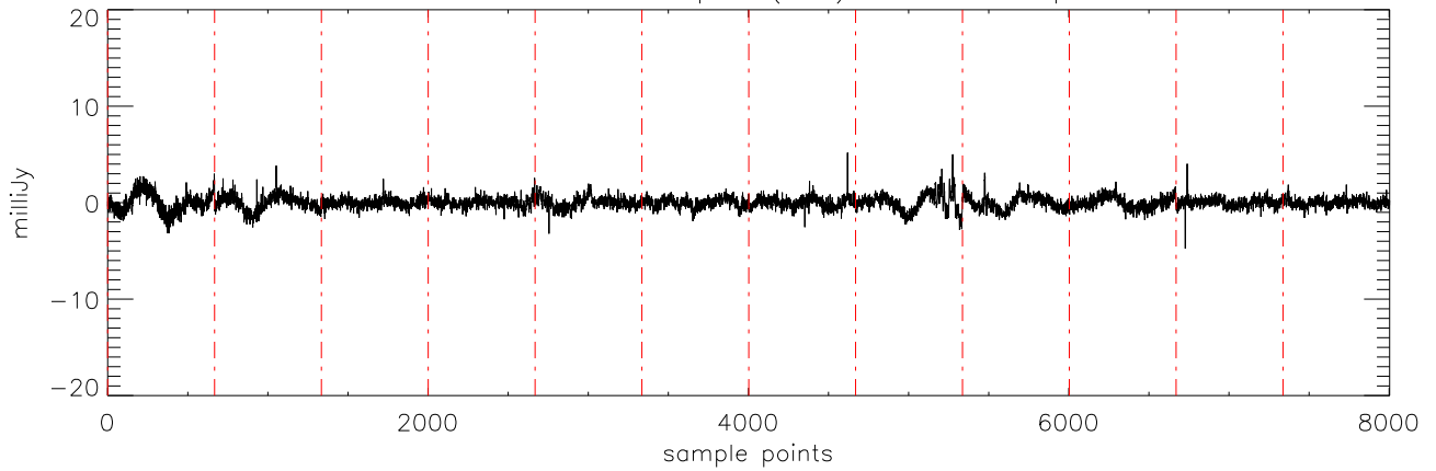
a2471 HD189733 06sep11 (AST) StokesU freq:4608.
