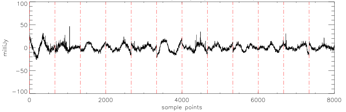
a2471 HD189733 06sep11 (AST) StokesI freq:5176.
