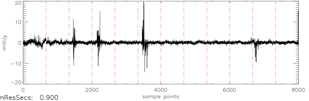
\alpha 2471 HD189733 06sep11 (AST) StokesV freq:4466.
