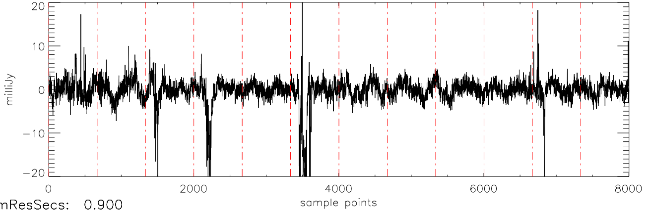
a2471 HD189733 06sep11 (AST) StokesQ freq:4466.
