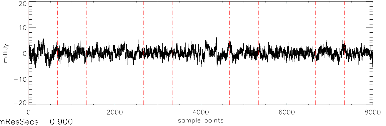
a2471 HD189733 06sep11 (AST) StokesQ freq:5034.
