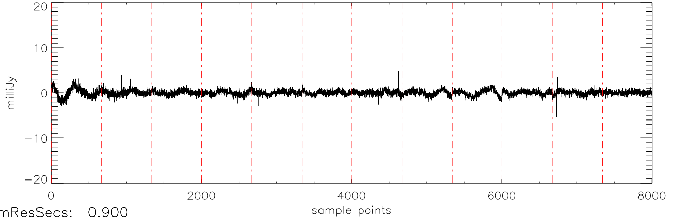
a2471 HD189733 06sep11 (AST) StokesU freq:5034.
