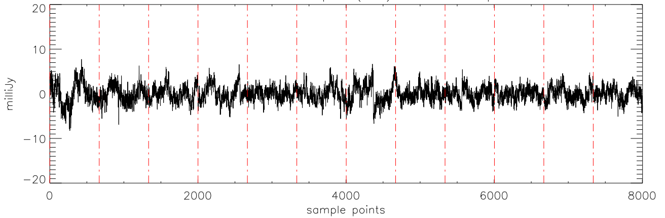
a2471 HD189733 06sep11 (AST) StokesQ freq:5176.
