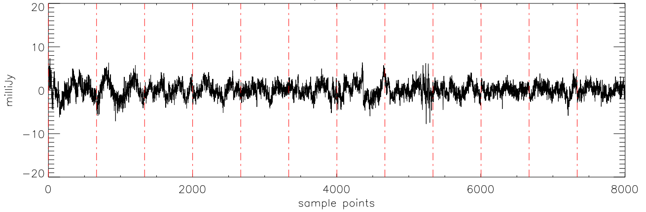
a2471 HD189733 06sep11 (AST) StokesQ freq:4750.
