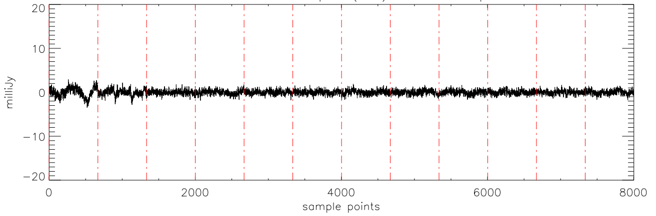
\alpha 2471 HD189733 06sep11 (AST) StokesV freq:5176.
