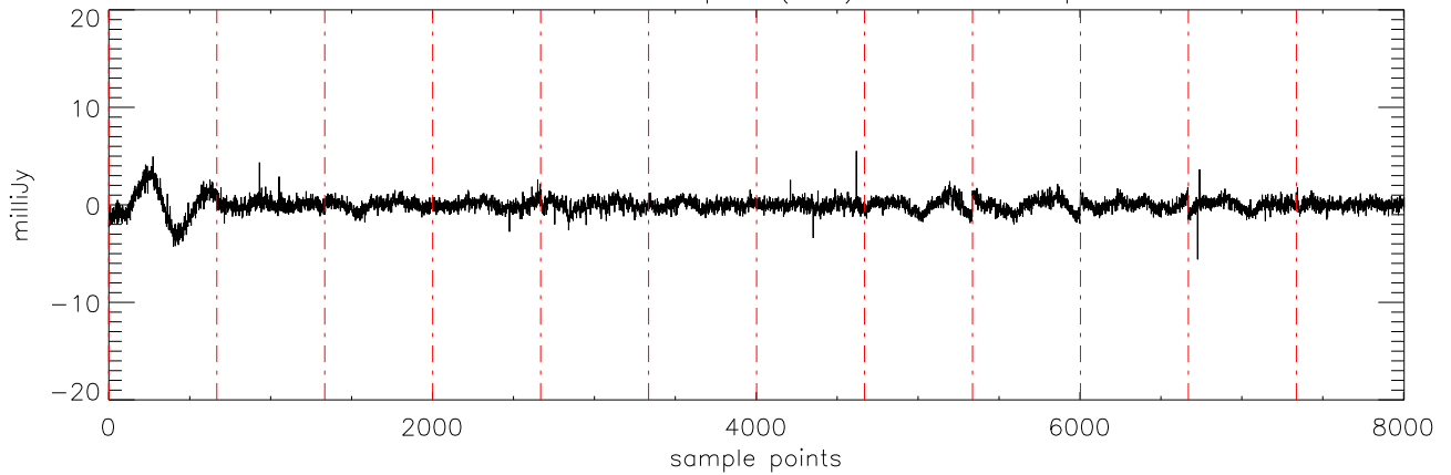
a2471 HD189733 06sep11 (AST) StokesU freq:4750.
