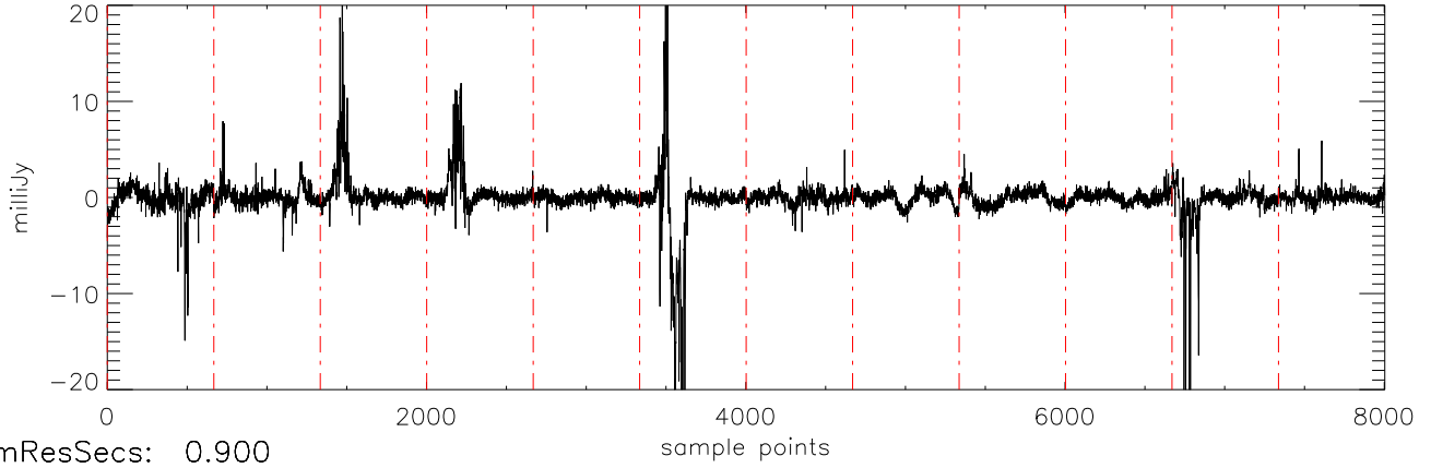
a2471 HD189733 06sep11 (AST) StokesU freq:4466.
