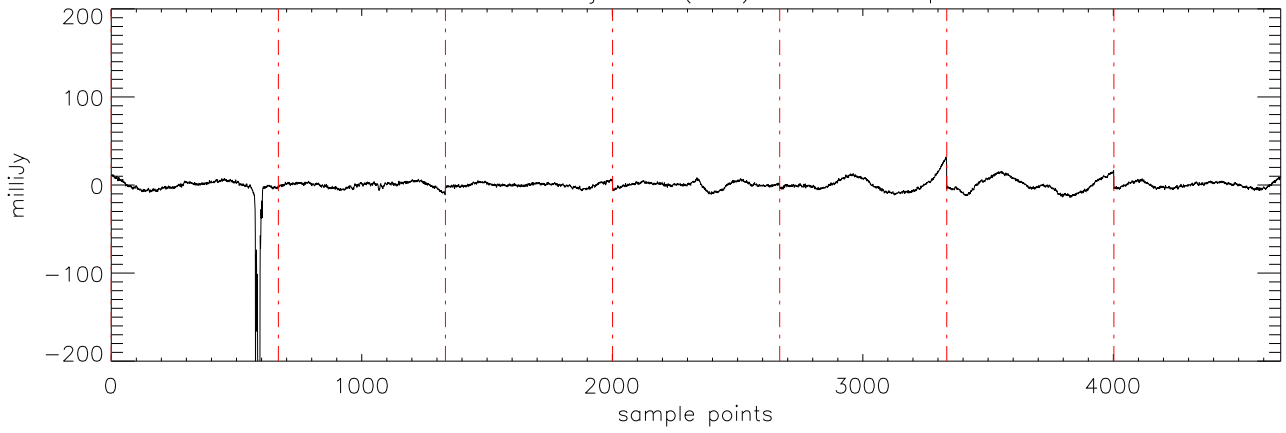
a2471 70Vir 06jan10 (AST) StokesI freq:4608.
