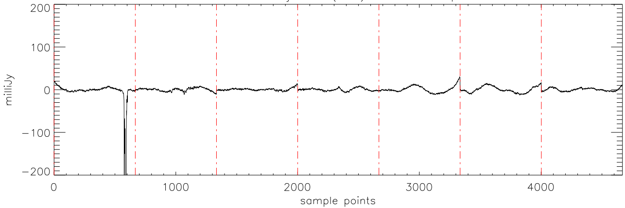
a2471 70Vir 06jan10 (AST) StokesI freq:4750.
