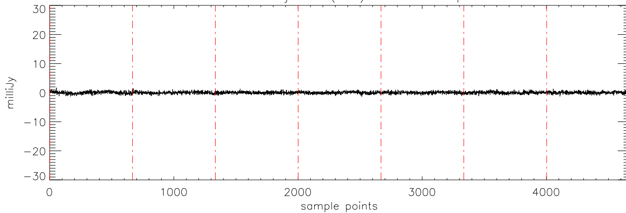
a2471 70Vir 06jan10 (AST) StokesV freq:4750.
