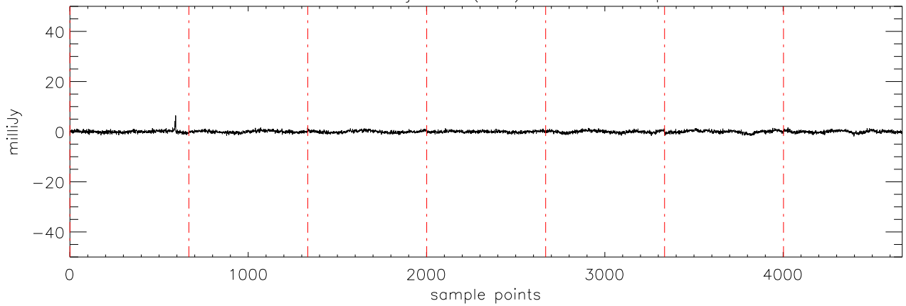
a2471 70Vir 06jan10 (AST) StokesU freq:4608.
