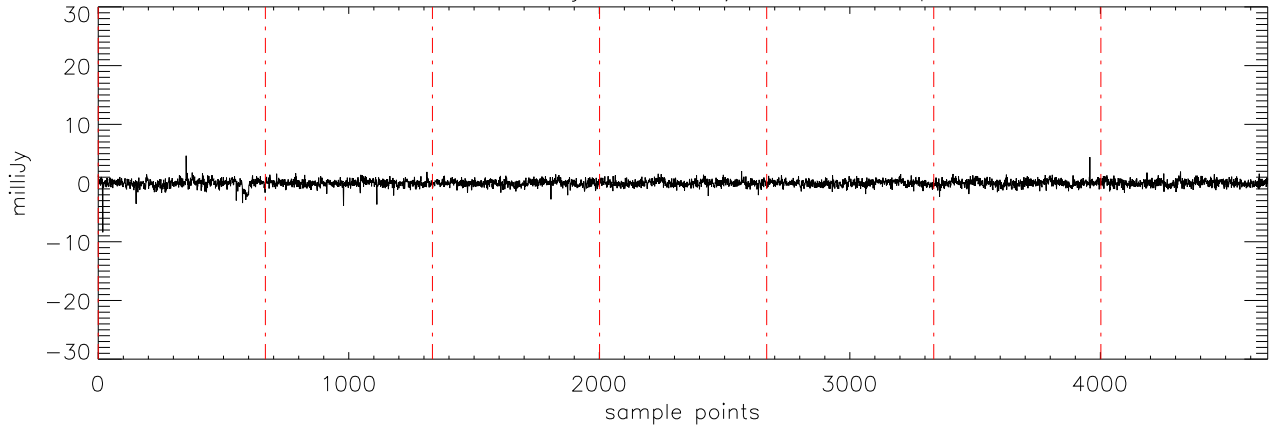
a2471 70Vir 06jan10 (AST) StokesV freq:5176.
