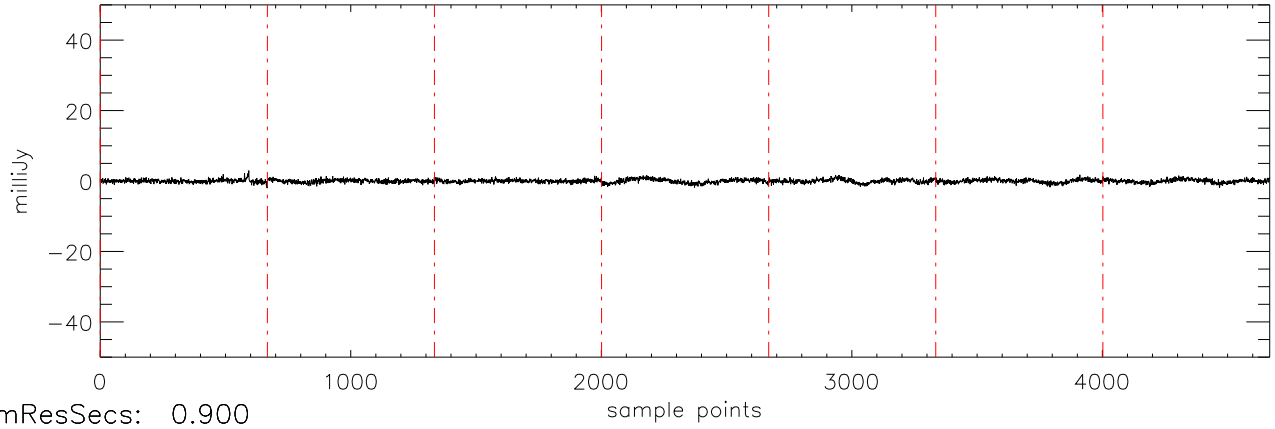
a2471 70Vir 06jan10 (AST) StokesU freq:5034.
