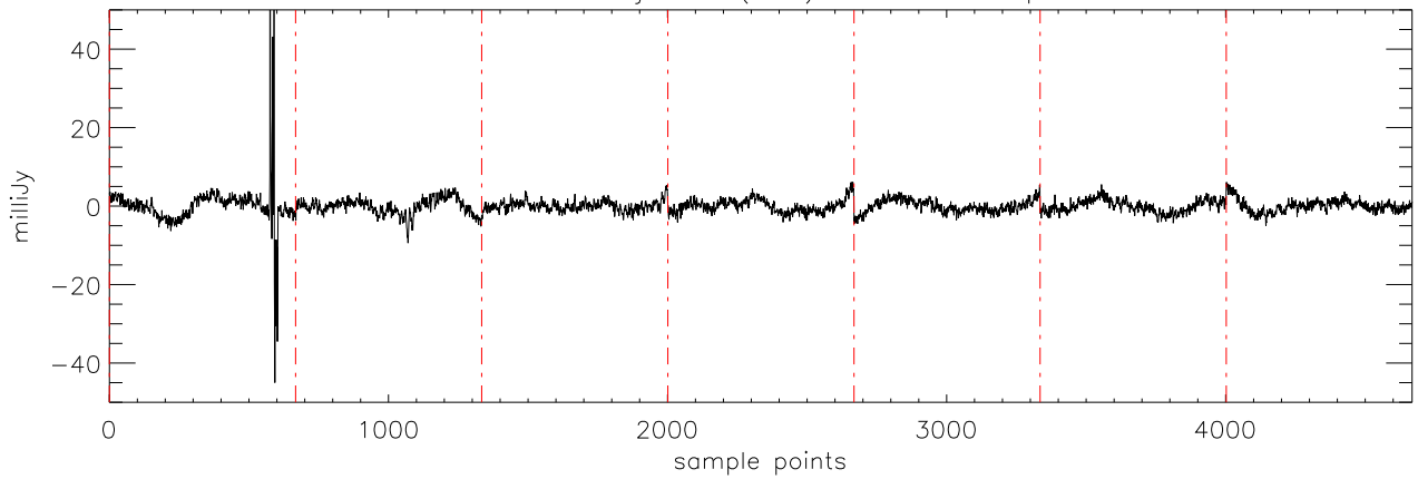
a2471 70Vir 06jan10 (AST) StokesQ freq:4608.
