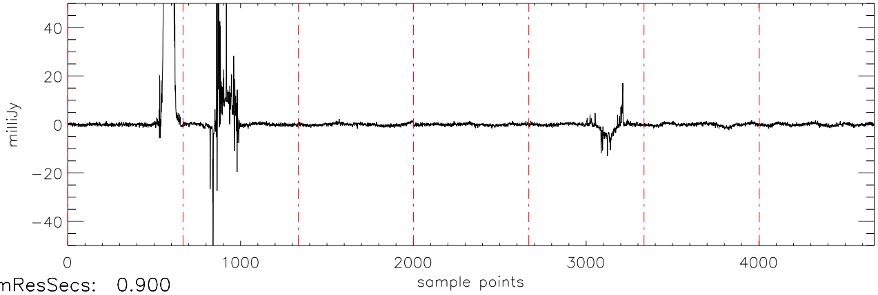
a2471 70Vir 06jan10 (AST) StokesU freq:4466.
