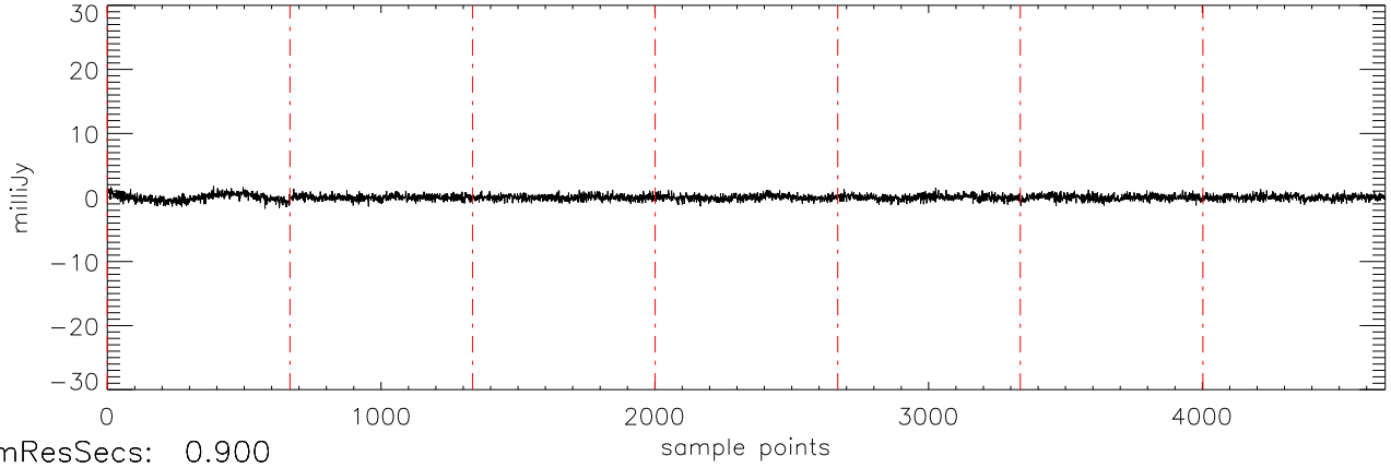
a2471 70Vir 06jan10 (AST) StokesV freq:5034.
