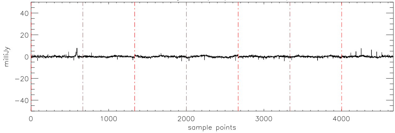
a2471 70Vir 06jan10 (AST) StokesU freq:5176.
