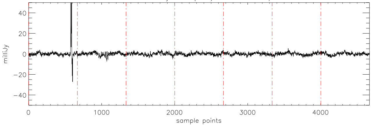
a2471 70Vir 06jan10 (AST) StokesQ freq:4750.
