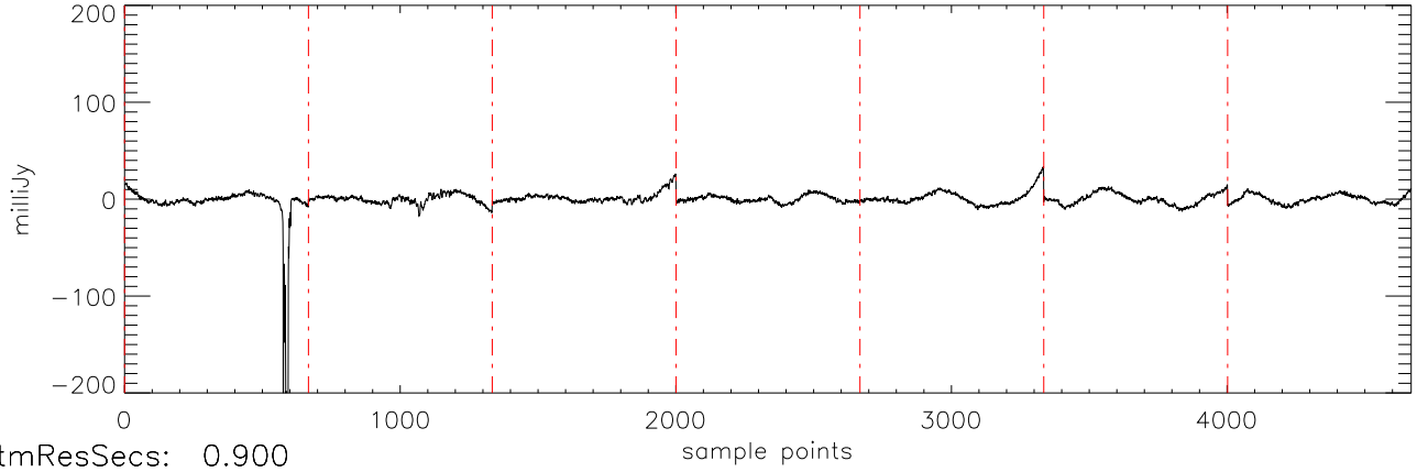
a2471 70Vir 06jan10 (AST) StokesI freq:5034.
