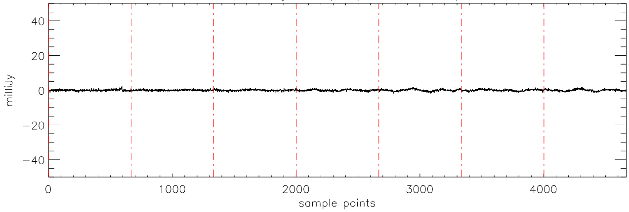
a2471 70Vir 06jan10 (AST) StokesU freq:4750.
