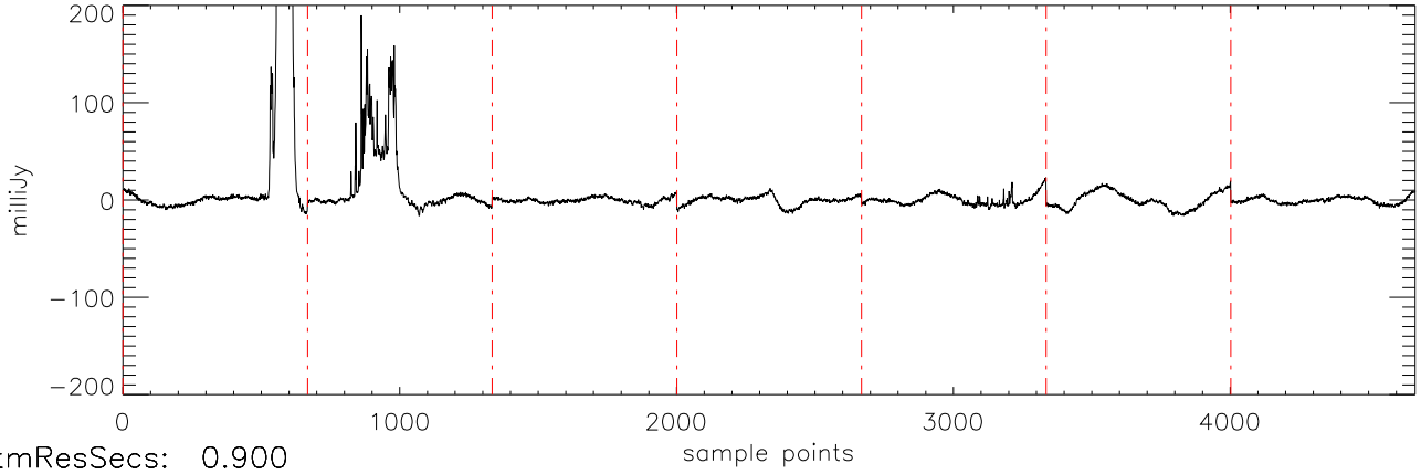
a2471 70Vir 06jan10 (AST) StokesI freq:4466.
