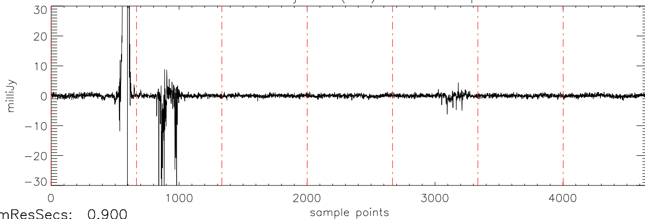
a2471 70Vir 06jan10 (AST) StokesV freq:4466.
