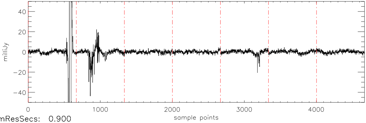
a2471 70Vir 06jan10 (AST) StokesQ freq:4466.
