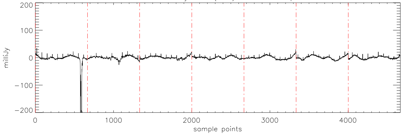
a2471 70Vir 06jan10 (AST) StokesI freq:5176.
