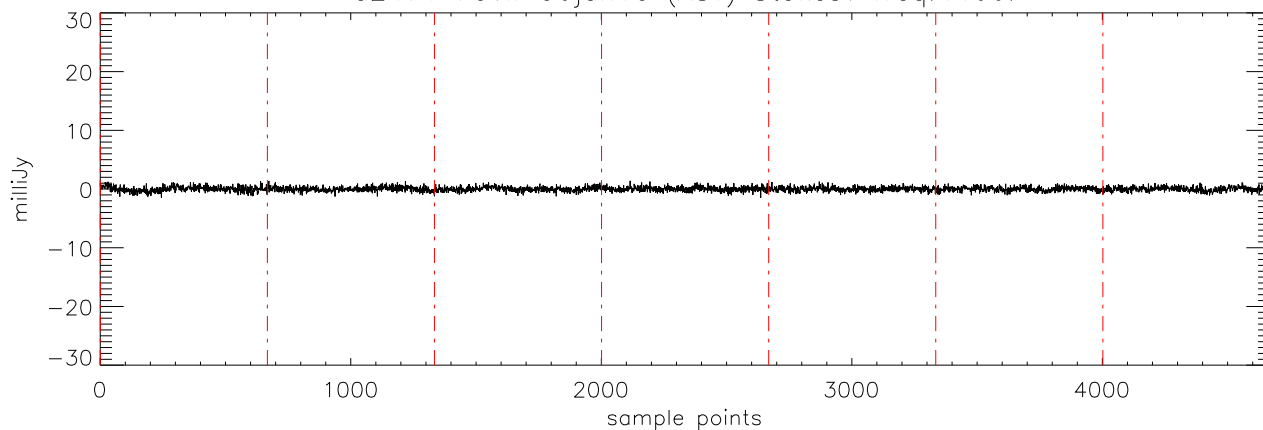
a2471 70Vir 06jan10 (AST) StokesV freq:4608.
