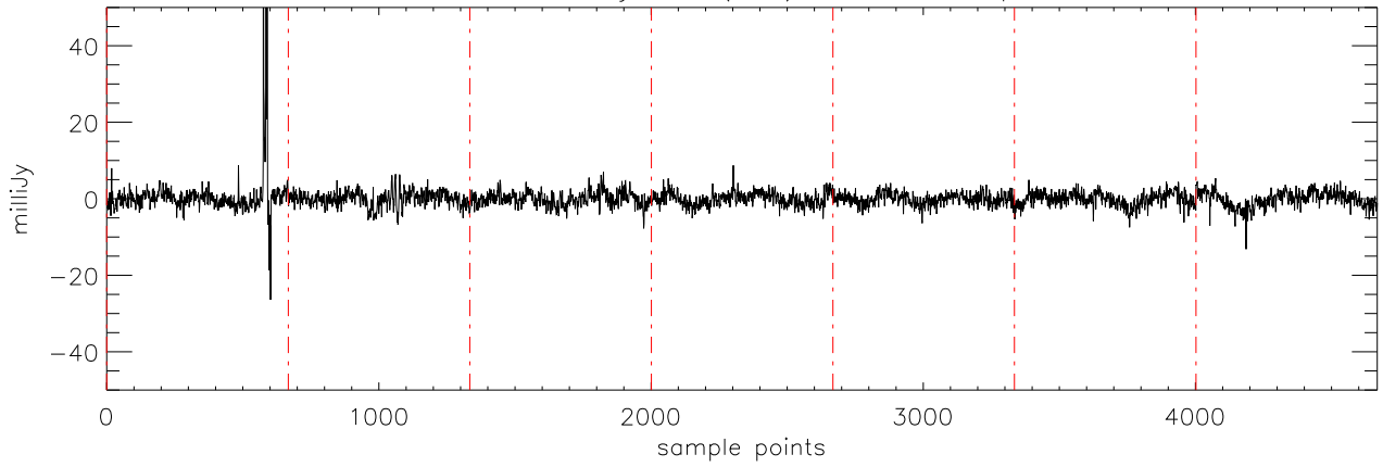
a2471 70Vir 06jan10 (AST) StokesQ freq:5176.
