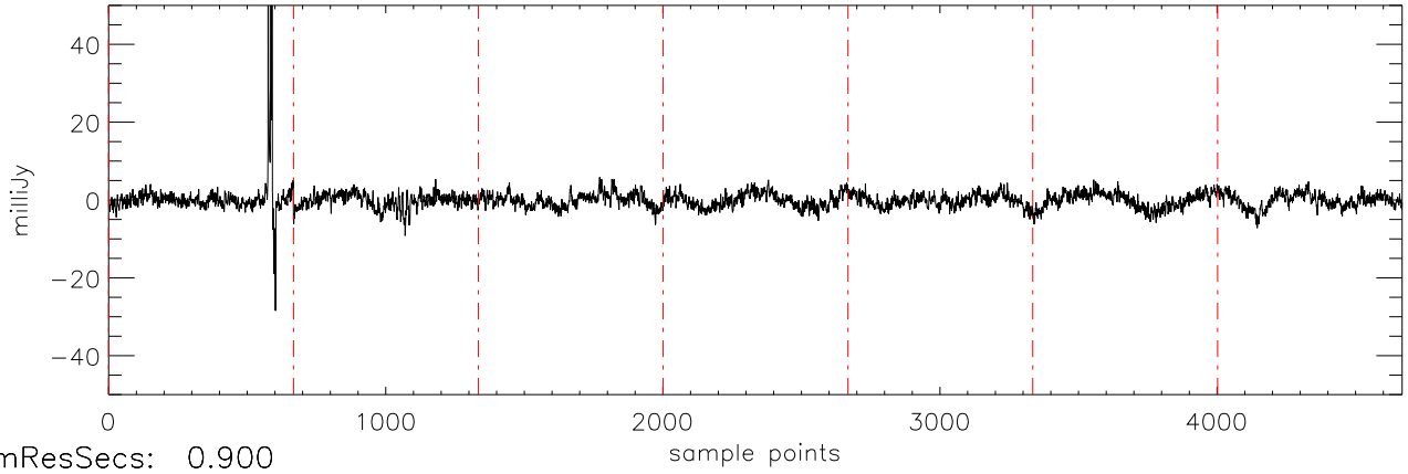
a2471 70Vir 06jan10 (AST) StokesQ freq:5034.
