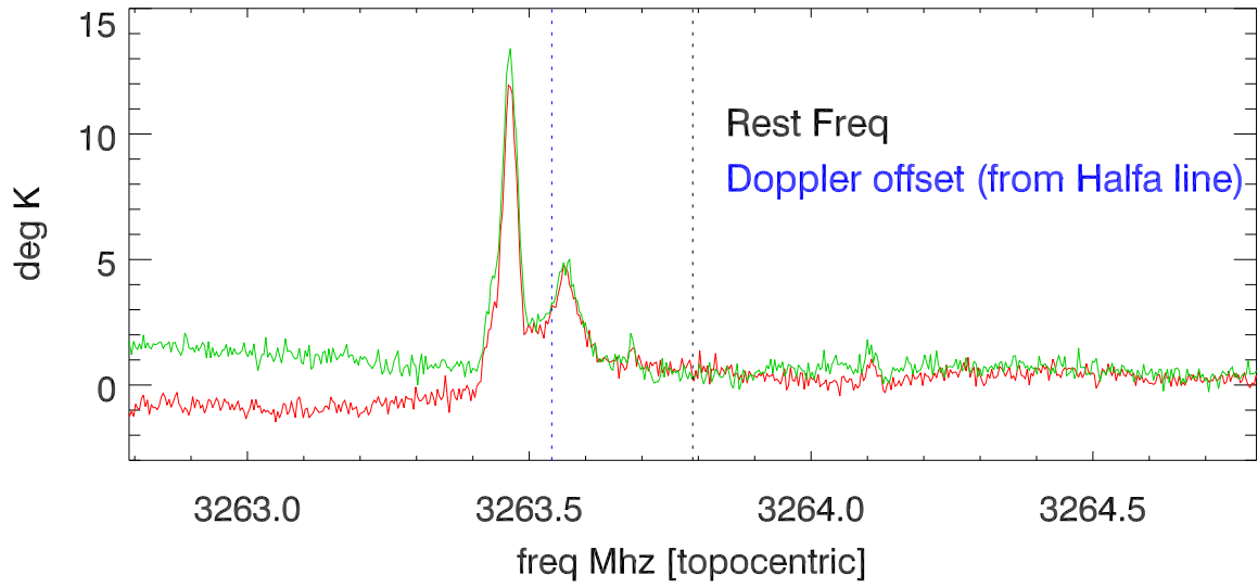
31may10 a2463 SBH CH lines: 3263.79 Mhz
