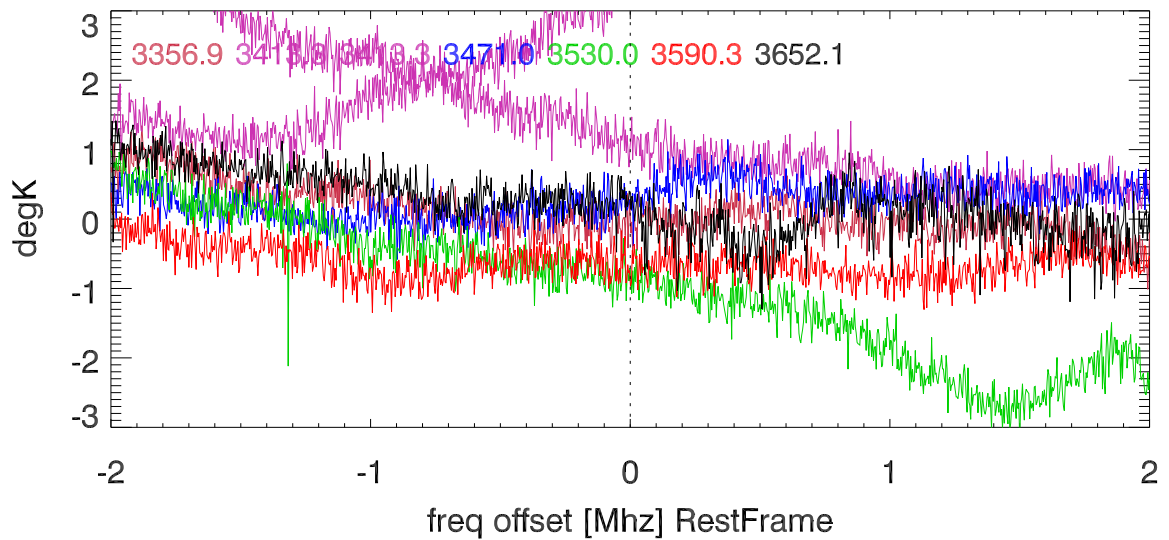
C_gamma 3335.7:3664.3 Mhz overplot lineNums
