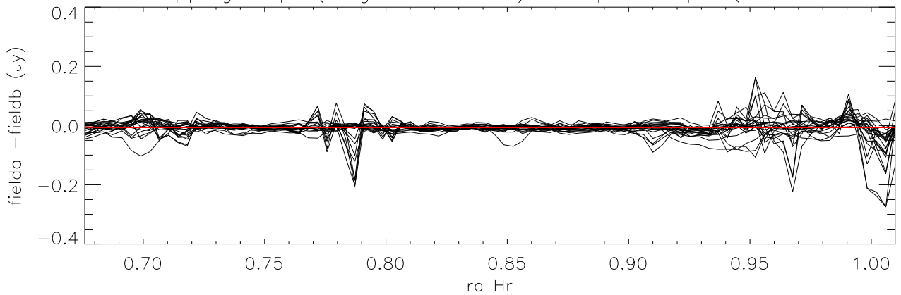
difference overlapping maps (long direction=ra) Cloop:5 Lloop:3 (Field1.05 - Field3.05)
