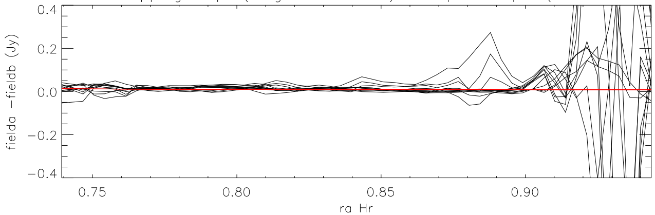
difference overlapping maps (long direction=ra) Cloop:5 Lloop:3 (Field6 - Field1.05)
