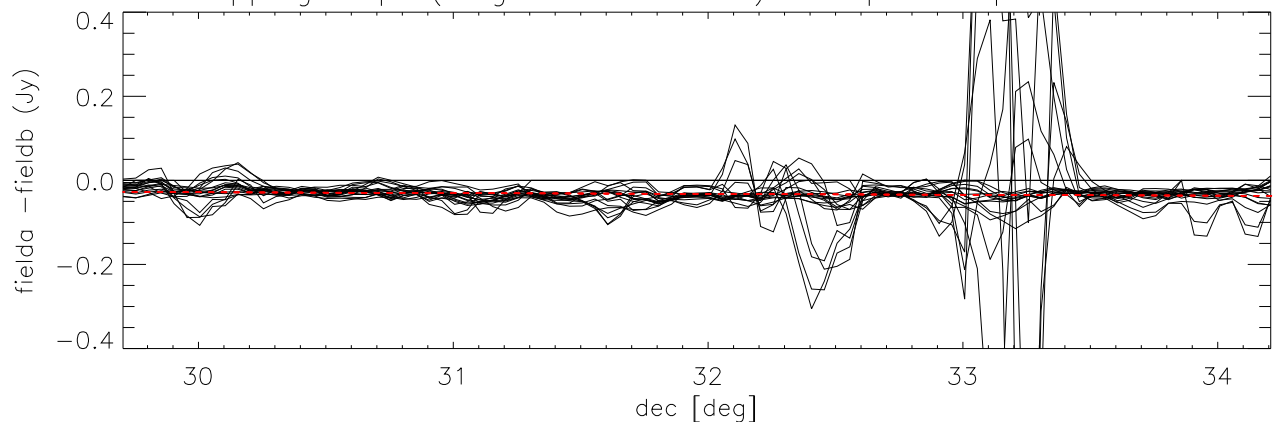
difference overlapping maps (long direction= dec) Cloop:5 Lloop:3 *Field4 - Field12)
