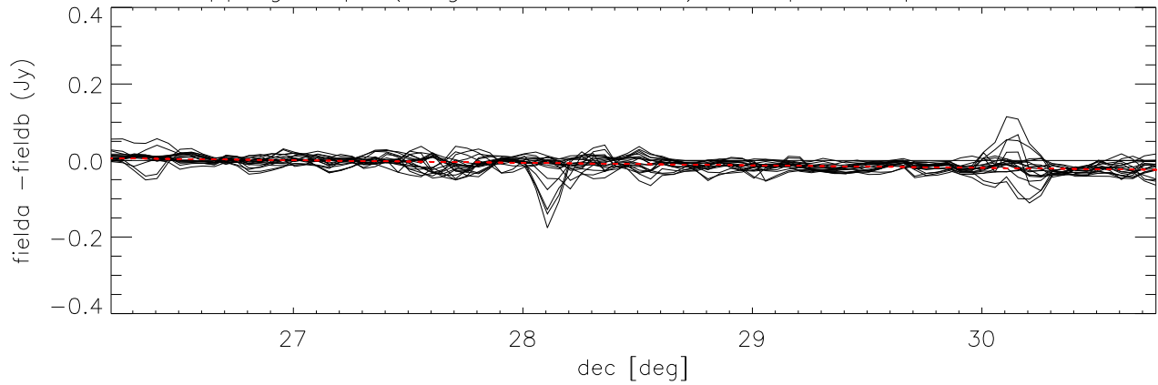
difference overlapping maps (long direction= dec) Cloop:5 Lloop:3 *Field5 - Field14)
