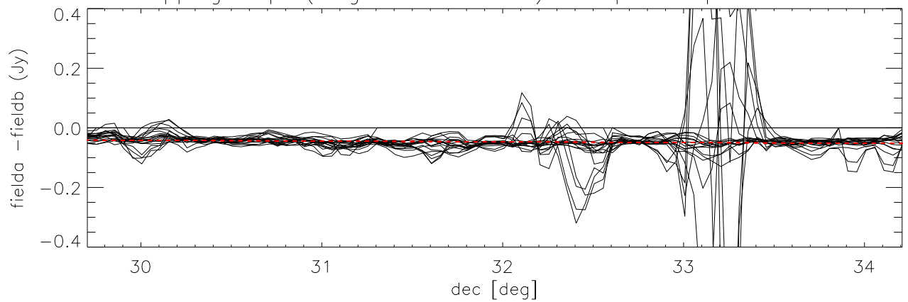
difference overlapping maps (long direction= dec) Cloop:4 Lloop:1 *Field4 - Field12)
