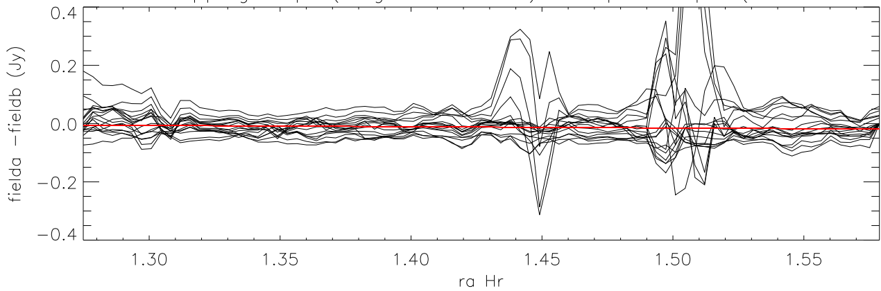
difference overlapping maps (long direction= dec) Cloop:4 Loop:1 *Field1 - Field2)
