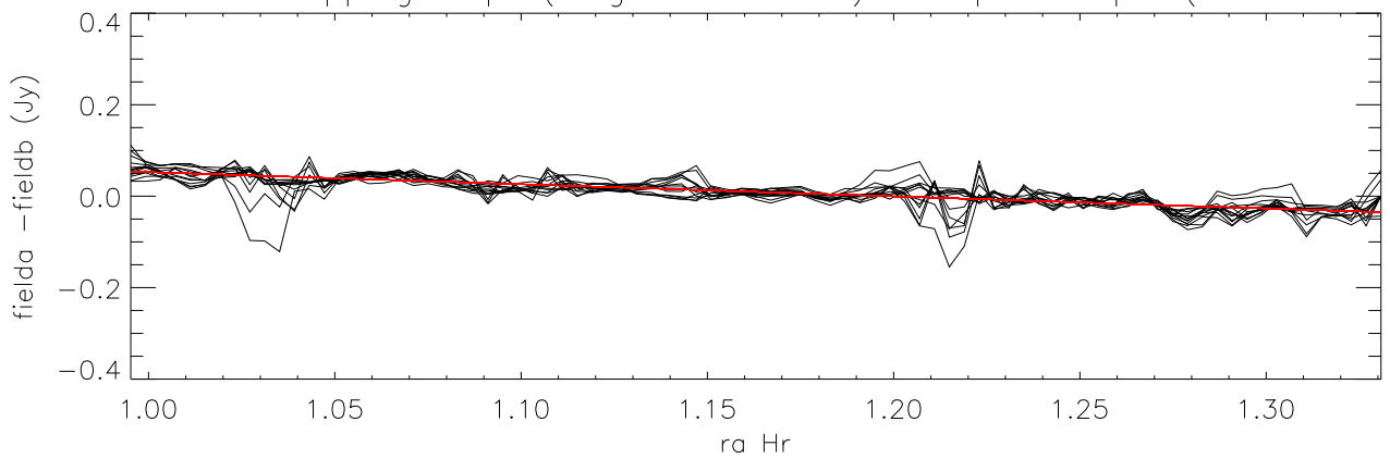
difference overlapping maps (long direction=ra) Cloop:4 Lloop:1 (Field2.05 - Field4.05)
