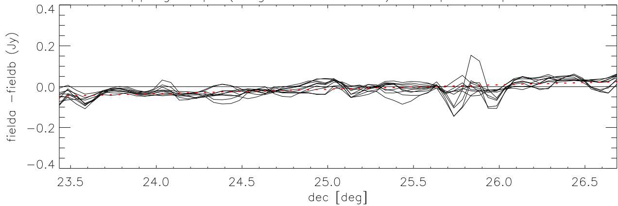
difference overlapping maps (long direction= dec) Cloop:4 Lloop:1 *Field6 – Field5)
