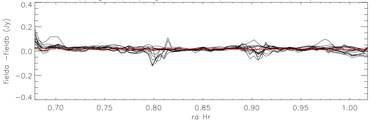
difference overlapping maps (long direction=ra) Cloop:4 Lloop:1 (Field3 - Field2)
