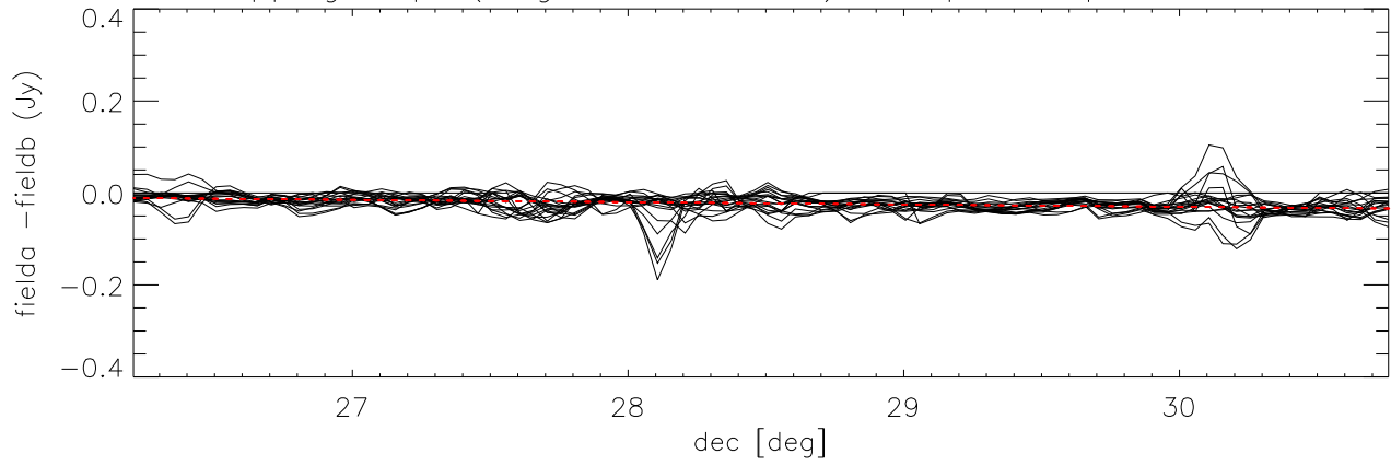
difference overlapping maps (long direction= dec) Cloop:4 Lloop:1 *Field5 – Field14)
