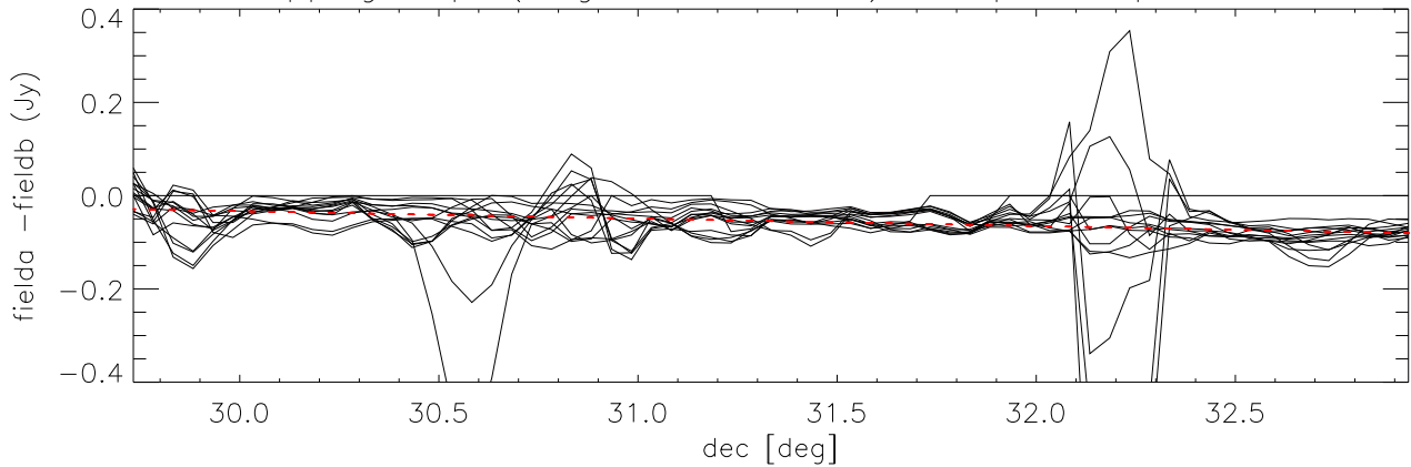
difference overlapping maps (long direction= dec) Cloop:4 Loop:1 *Field3 - Field11A)
