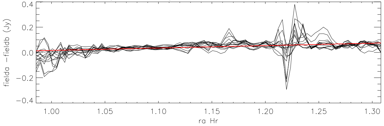
difference overlapping maps (long direction=ra) Cloop:4 Lloop:1 (Field12 - Field11A)
