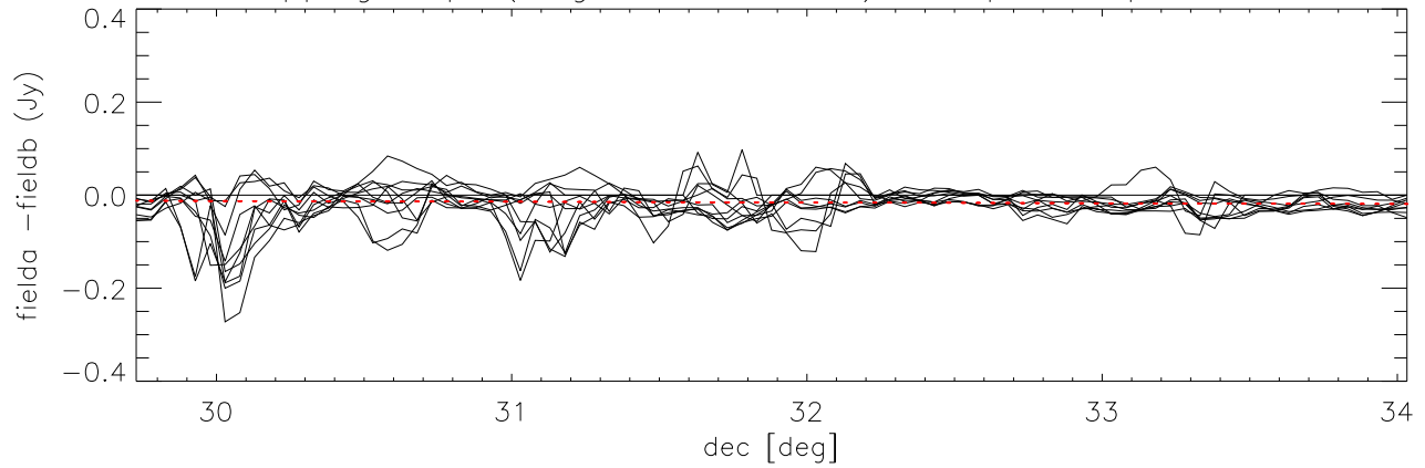
difference overlapping maps (long direction= dec) Cloop:4 Lloop:1 *Field4.05 - Field3.05)
