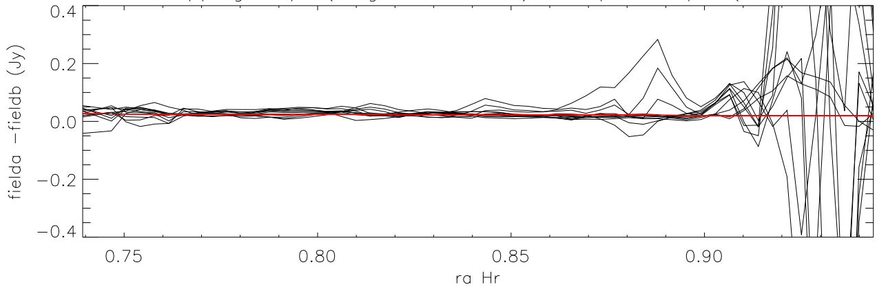
difference overlapping maps (long direction=ra) Cloop:4 Lloop:1 (Field6 - Field1.05)
