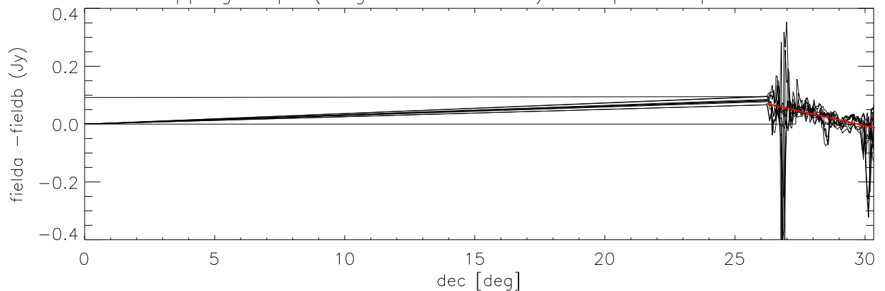
difference overlapping maps (long direction= dec) Cloop:4 Lloop:1 *Field1.05 - Field4)
