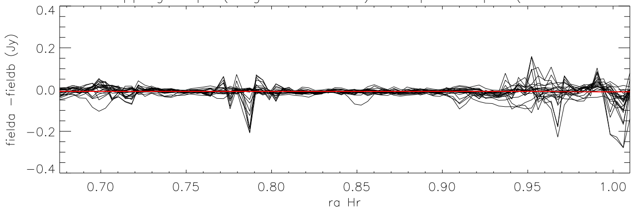
difference overlapping maps (long direction=ra) Cloop:4 Lloop:1 (Field1.05 - Field3.05)
