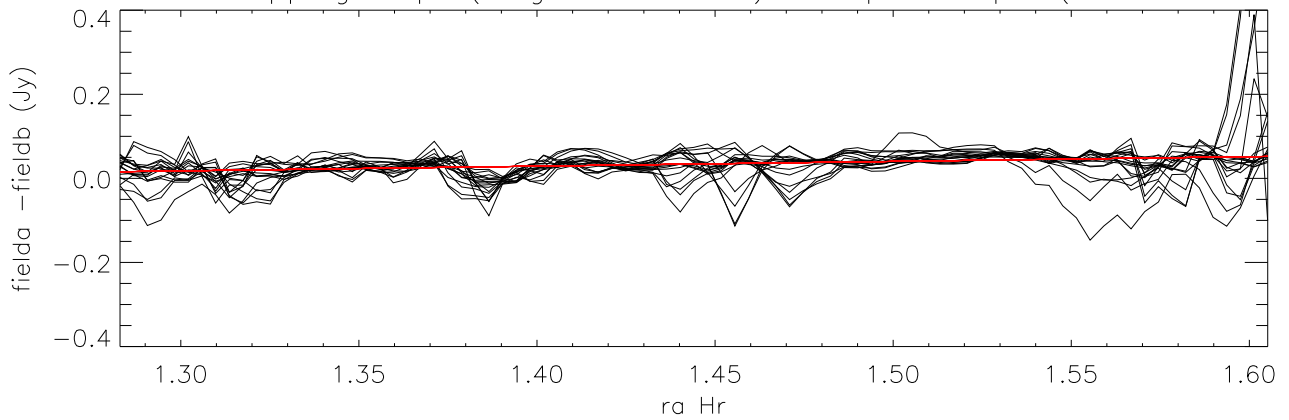
difference overlapping maps (long direction=ra) Cloop:4 Lloop:1 (Field7 - Field2.05)
