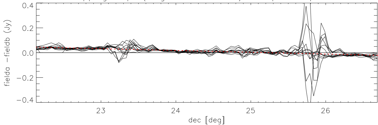
difference overlapping maps (long direction= dec) Cloop:4 Lloop:1 *Field7 – Field6)
