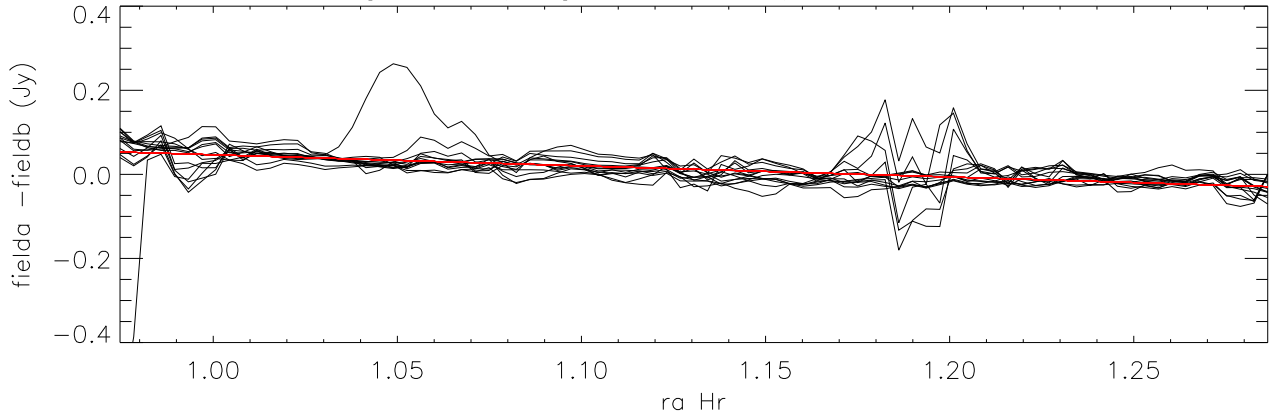
difference overlapping maps (long direction=ra) Cloop:4 Loop:1 (Field14 - Field12)
