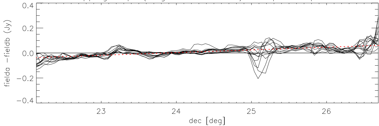
difference overlapping maps (long direction= dec) Cloop:3 Lloop:1 *Field7 - Field6)
