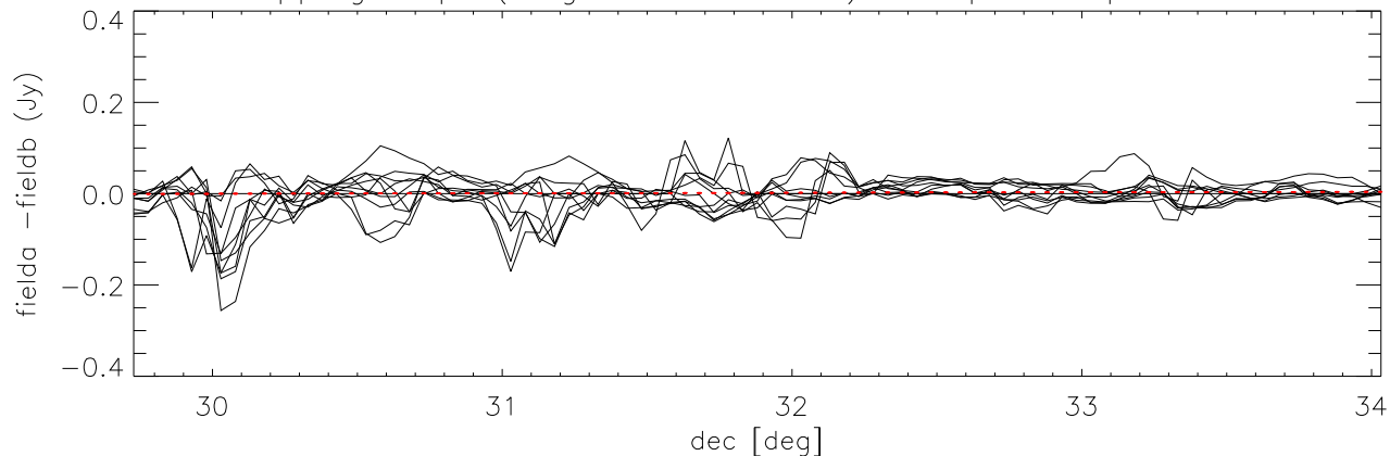
difference overlapping maps (long direction= dec) Cloop:3 Lloop:1 *Field4.05 - Field3.05)
