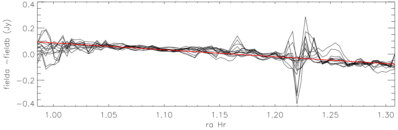
difference overlapping maps (long direction=ra) Cloop:3 Lloop:1 (Field12 - Field11A)
