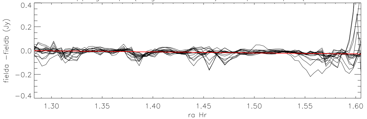
difference overlapping maps (long direction=ra) Cloop:3 Lloop:1 (Field7 - Field2.05)
