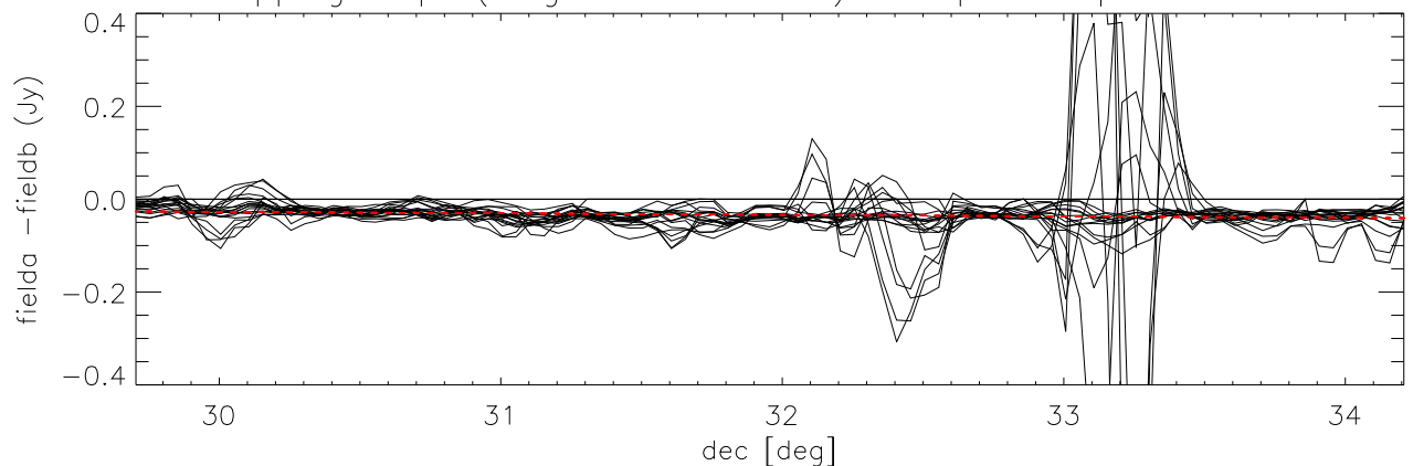
difference overlapping maps (long direction= dec) Cloop:3 Lloop:1 *Field4 - Field12)
