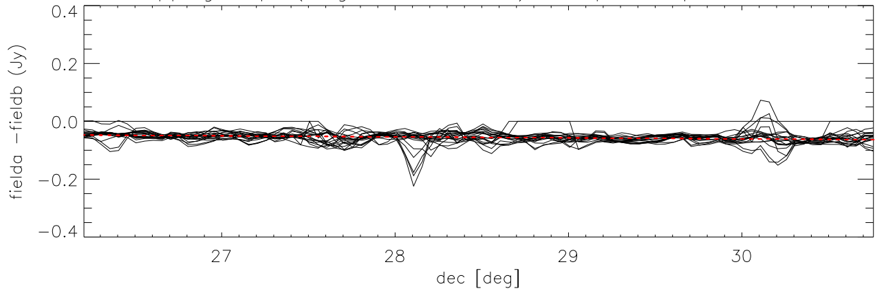
difference overlapping maps (long direction= dec) Cloop:3 Lloop:1 *Field5 - Field14)
