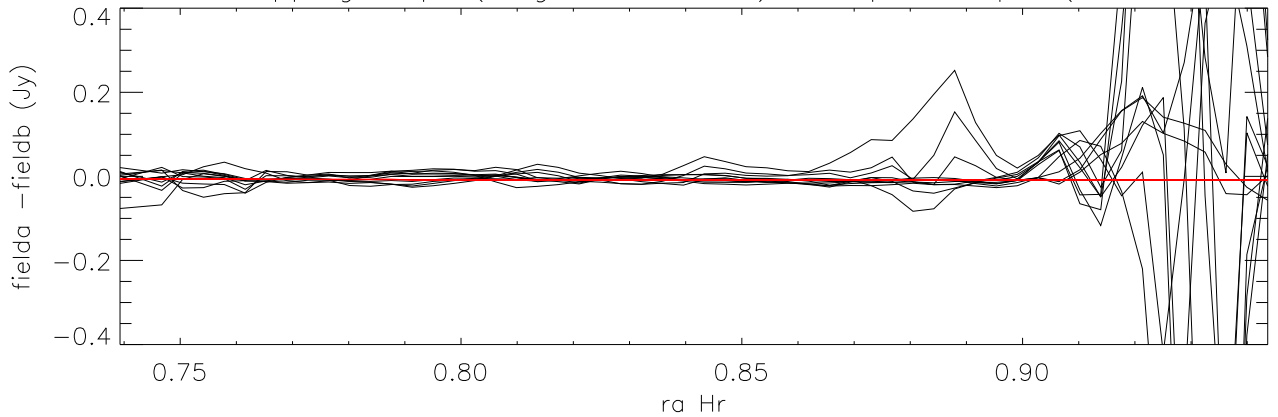
difference overlapping maps (long direction=ra) Cloop:3 Lloop:1 (Field6 - Field1.05)
