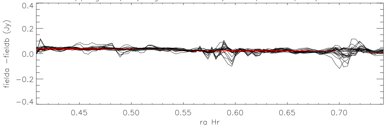
difference overlapping maps (long direction=ra) Cloop:3 Lloop:1 (Field1.05 - Field3.05)
