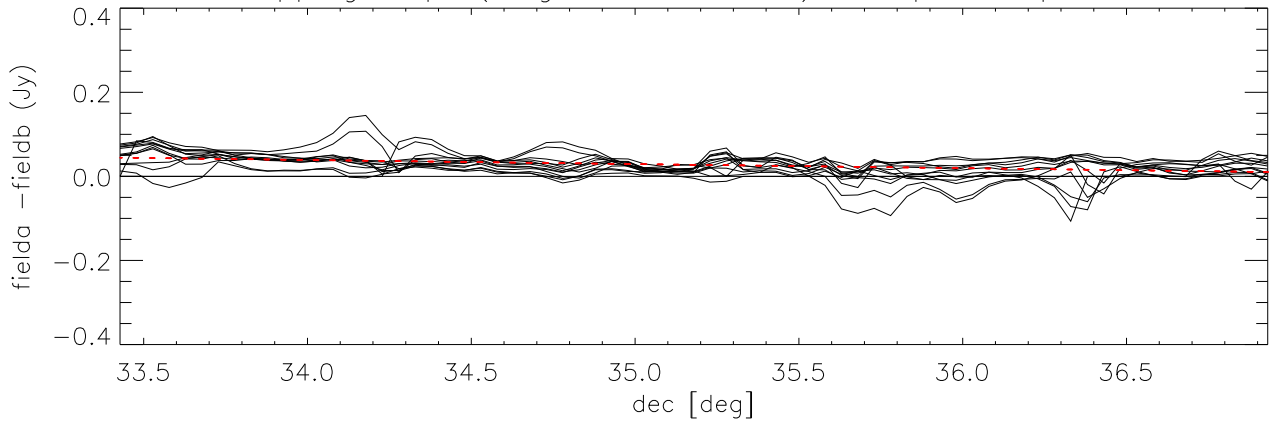
difference overlapping maps (long direction= dec) Cloop:3 Loop:1 *Field3 - Field11A)
