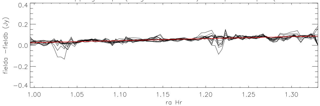
difference overlapping maps (long direction=ra) Cloop:3 Lloop:1 (Field2.05 - Field4.05)
