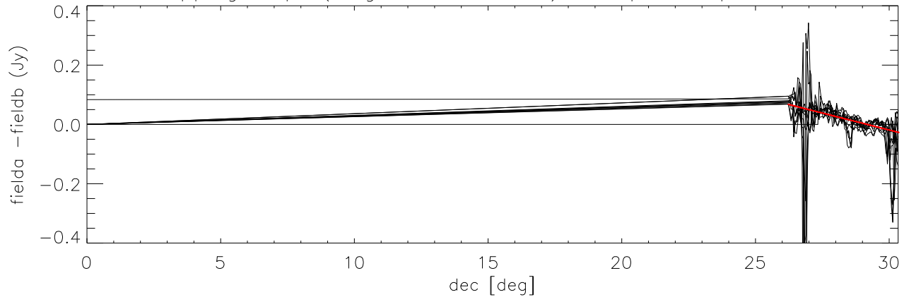
difference overlapping maps (long direction= dec) Cloop:3 Lloop:1 *Field1.05 - Field4)
