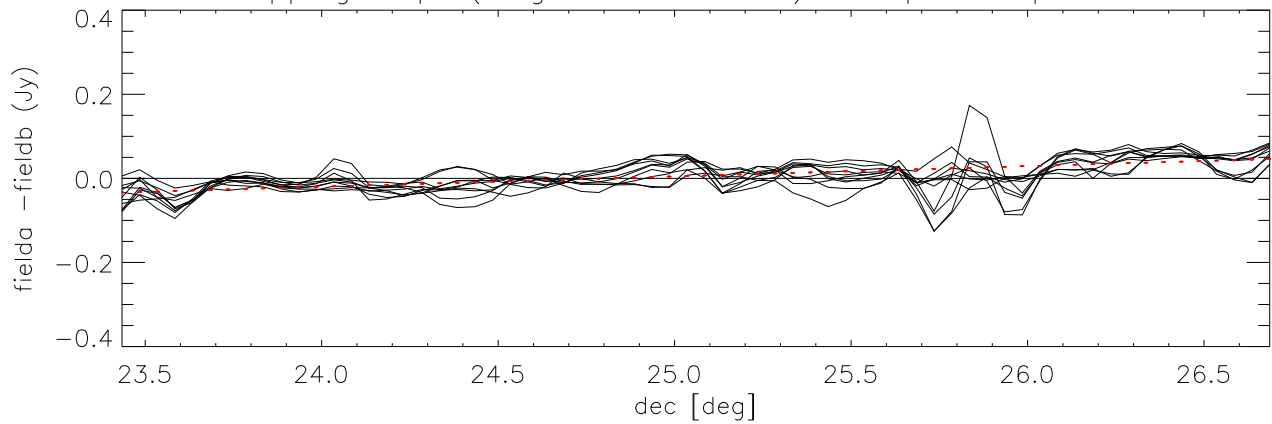
difference overlapping maps (long direction= dec) Cloop:3 Lloop:1 *Field6 - Field5)
