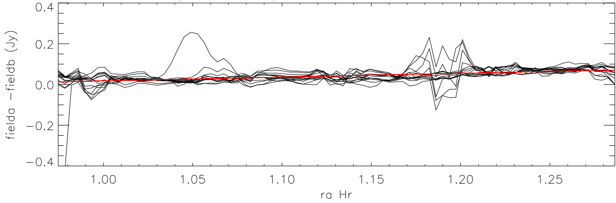
difference overlapping maps (long direction=ra) Cloop:3 Loop:1 (Field14 - Field12)
