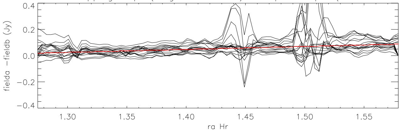
difference overlapping maps (long direction= dec) Cloop:3 Loop:1 *Field1 - Field2)
