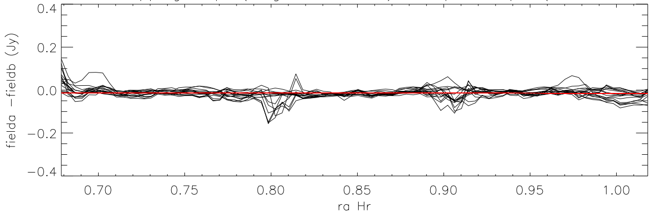
difference overlapping maps (long direction=ra) Cloop:3 Lloop:1 (Field3 - Field2)
