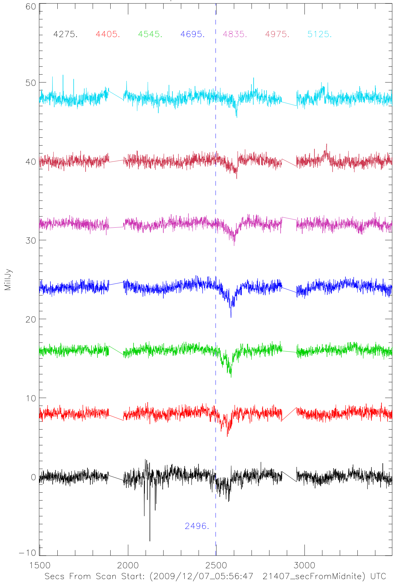
06dec09 cband blowup stokes V TP vs time for 2MASS0746
