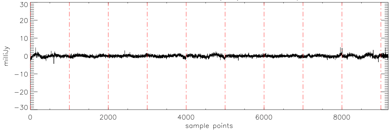
a2430 2MASS0746 05dec09 (AST) StokesV freq:5125.
