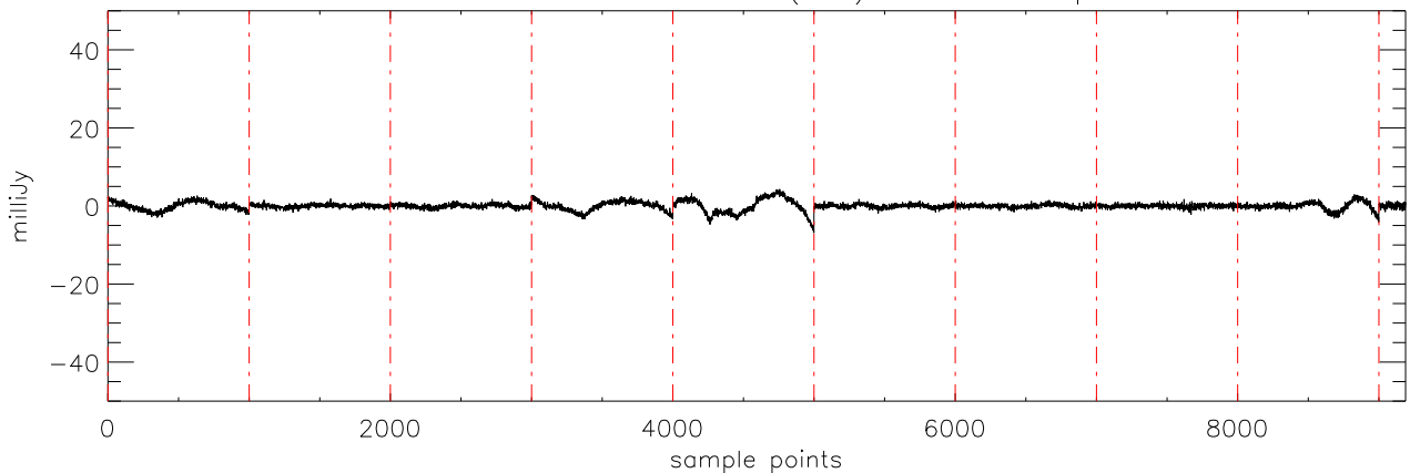
a2430 2MASS0746 05dec09 (AST) StokesU freq:4695.
