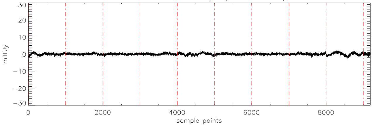
a2430 2MASS0746 05dec09 (AST) StokesV freq:4695.
