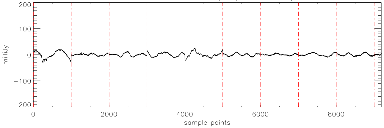
a2430 2MASS0746 05dec09 (AST) StokesI freq:4545.
