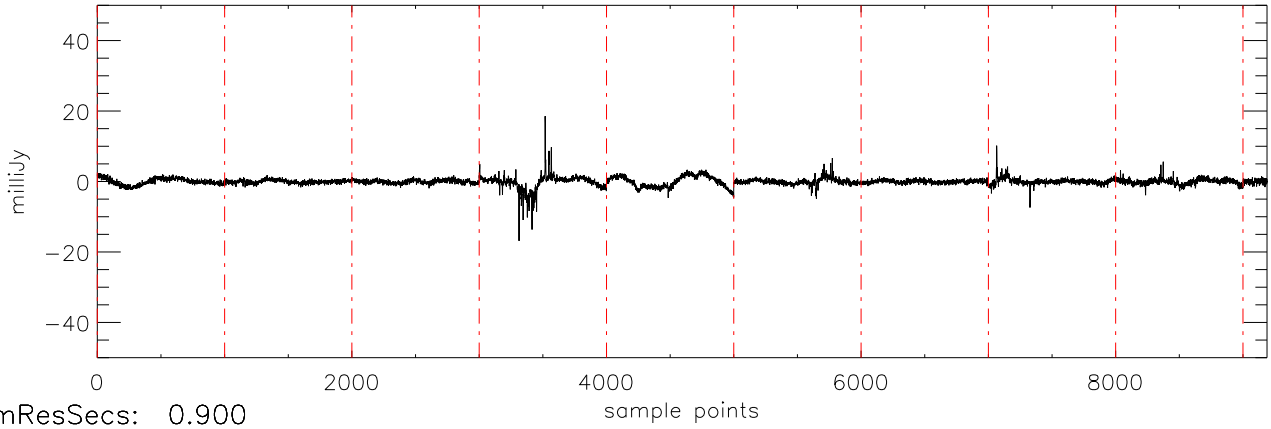
a2430 2MASS0746 05dec09 (AST) StokesU freq:4405.
