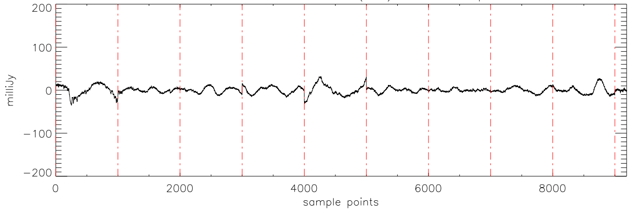
a2430 2MASS0746 05dec09 (AST) StokesI freq:5125.
