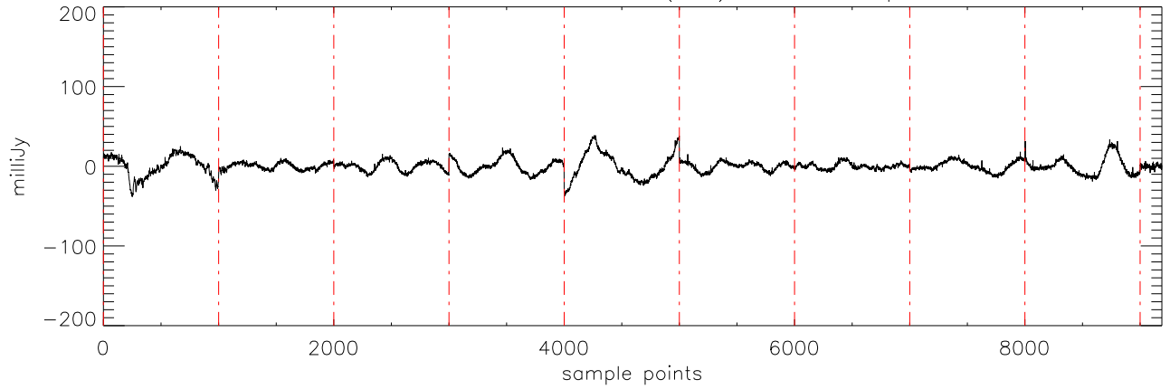
a2430 2MASS0746 05dec09 (AST) StokesI freq:5125.
