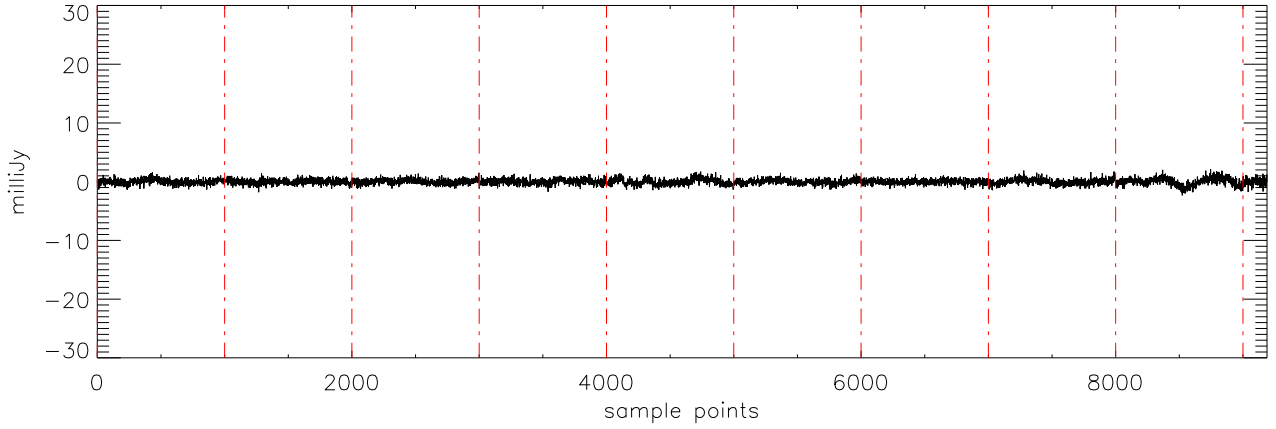
a2430 2MASS0746 05dec09 (AST) StokesV freq:4545.
