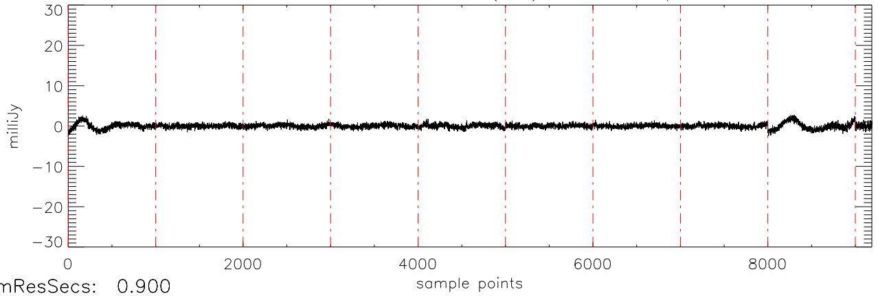
a2430 2MASS0746 05dec09 (AST) StokesV freq:4975.
