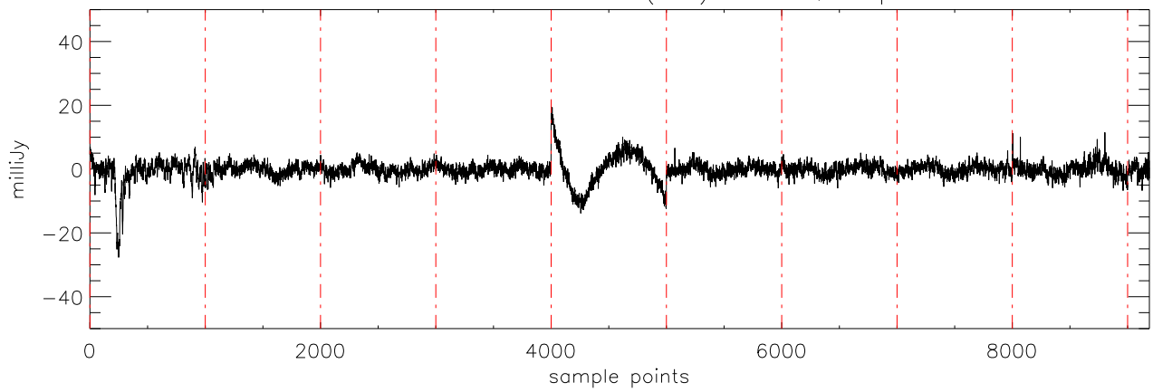
a2430 2MASS0746 05dec09 (AST) StokesQ freq:5125.
