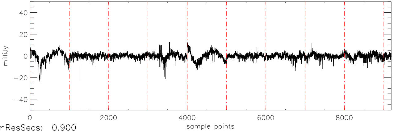
a2430 2MASS0746 05dec09 (AST) StokesQ freq:4405.
