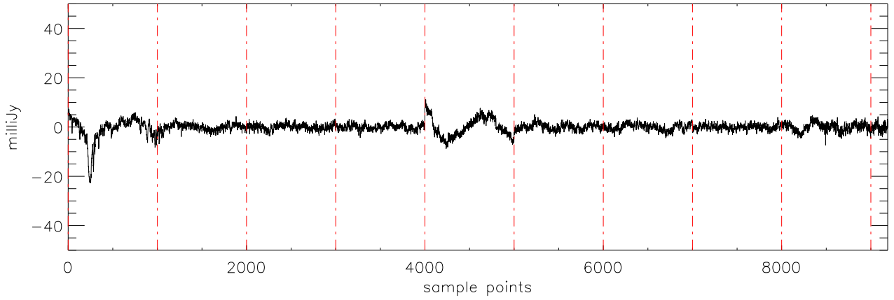
a2430 2MASS0746 05dec09 (AST) StokesQ freq:4545.
