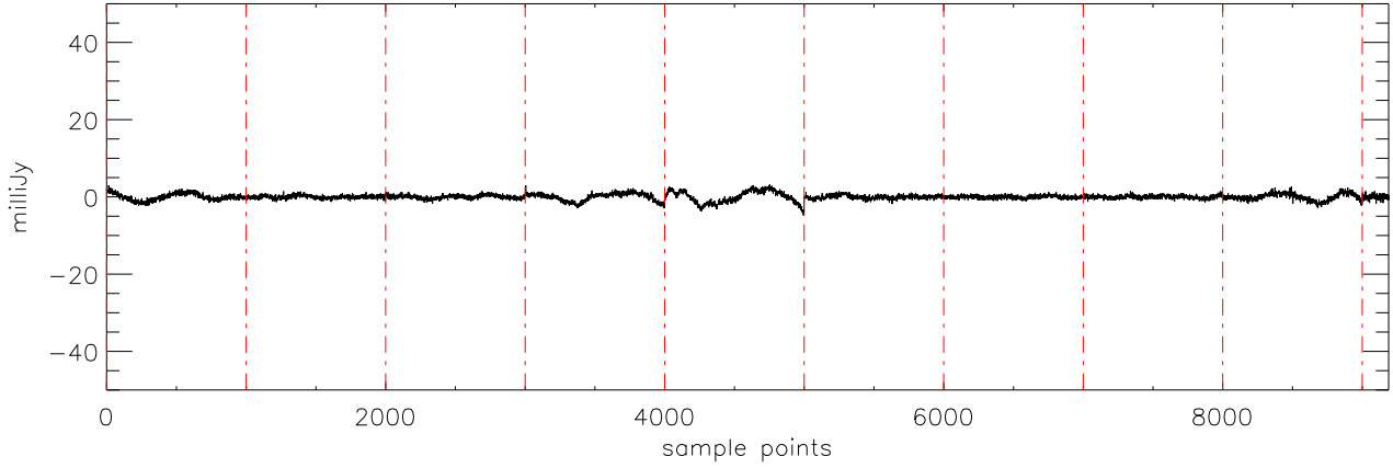
a2430 2MASS0746 05dec09 (AST) StokesU freq:4545.
