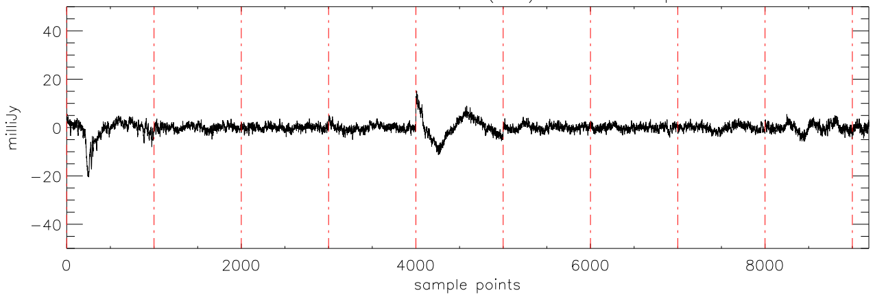
a2430 2MASS0746 05dec09 (AST) StokesQ freq:4695.
