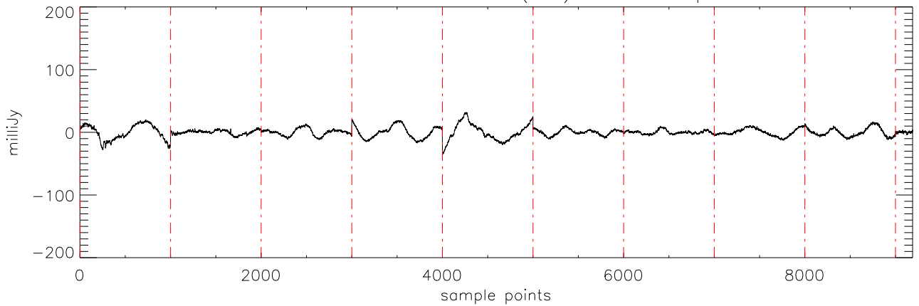
a2430 2MASS0746 05dec09 (AST) StokesI freq:4695.
