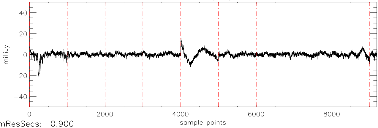
a2430 2MASS0746 05dec09 (AST) StokesQ freq:4975.
