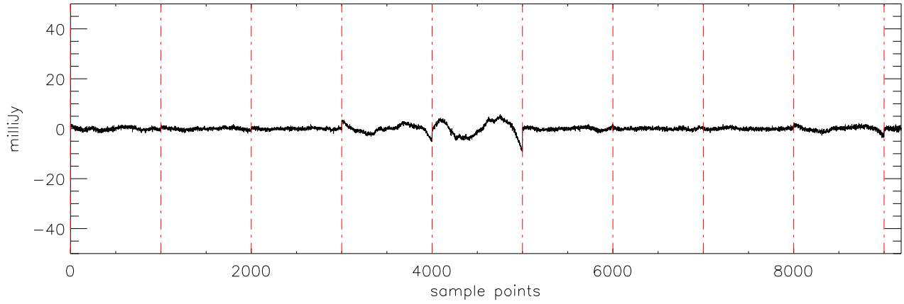
a2430 2MASS0746 05dec09 (AST) StokesU freq:5125.
