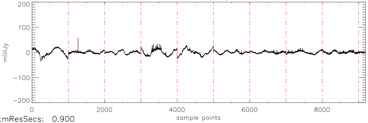
a2430 2MASS0746 05dec09 (AST) StokesI freq:4405.
