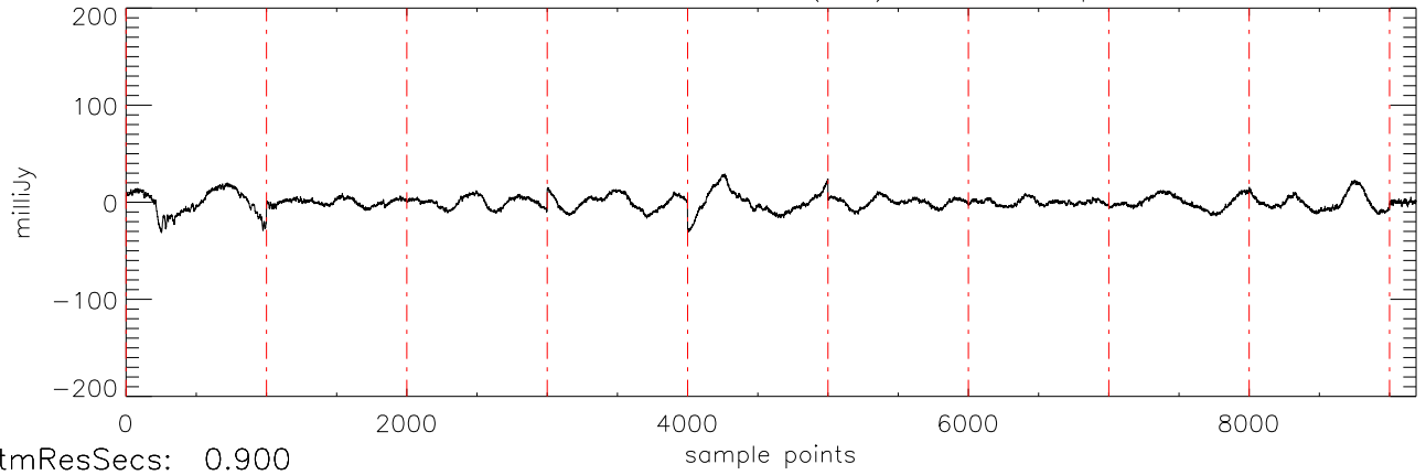
a2430 2MASS0746 05dec09 (AST) StokesI freq:4975.
