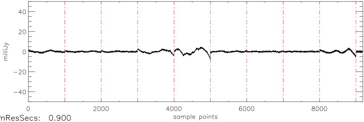
a2430 2MASS0746 05dec09 (AST) StokesU freq:4975.
