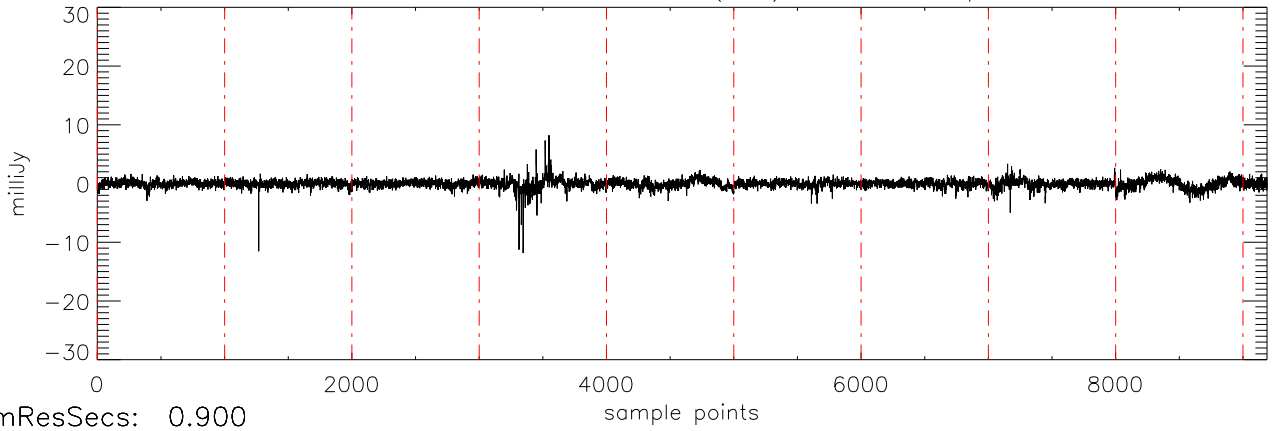
a2430 2MASS0746 05dec09 (AST) StokesV freq:4405.
