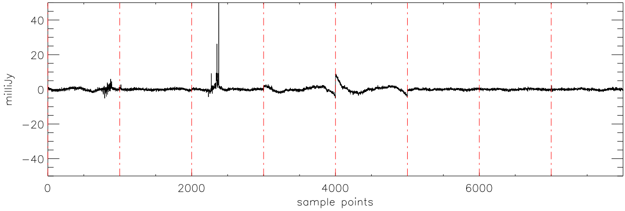
a2430 2MASS0746 03dec09 (AST) StokesU freq:4545.
