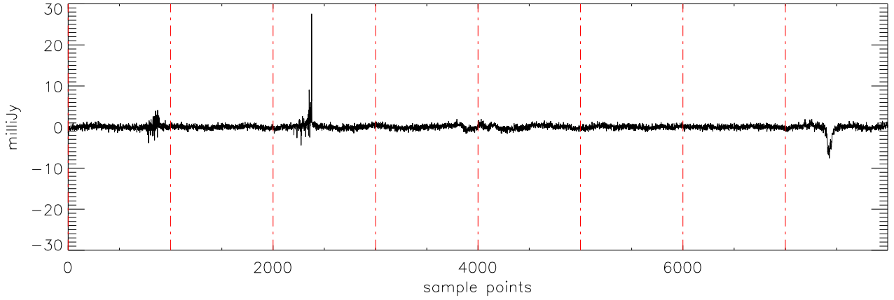
a2430 2MASS0746 03dec09 (AST) StokesV freq:4545.
