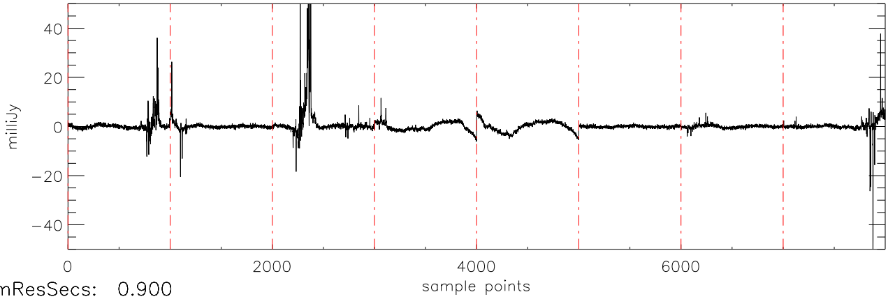
a2430 2MASS0746 03dec09 (AST) StokesU freq:4405.
