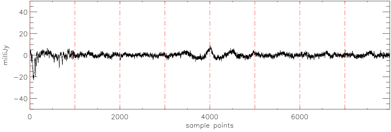
a2430 2MASS0746 03dec09 (AST) StokesQ freq:5125.
