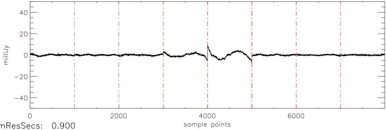
a2430 2MASS0746 03dec09 (AST) StokesU freq:4975.
