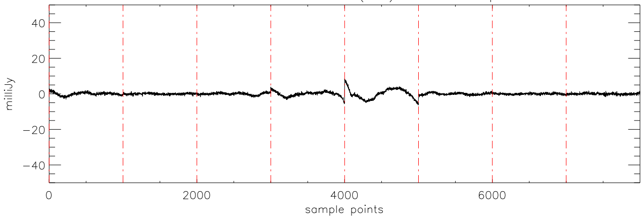
a2430 2MASS0746 03dec09 (AST) StokesU freq:4695.
