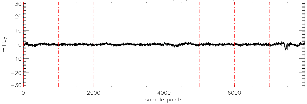
a2430 2MASS0746 03dec09 (AST) StokesV freq:5125.
