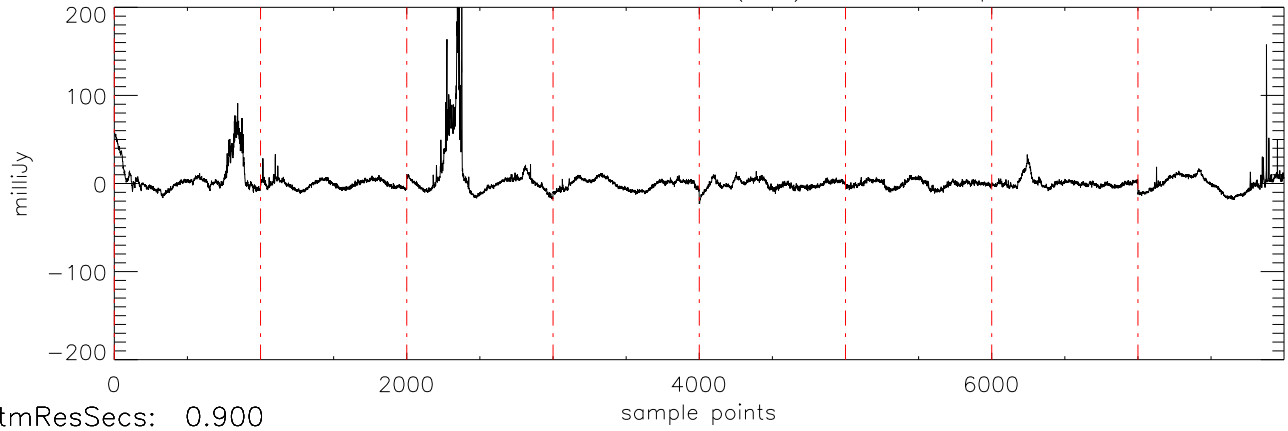
a2430 2MASS0746 03dec09 (AST) StokesI freq:4405.
