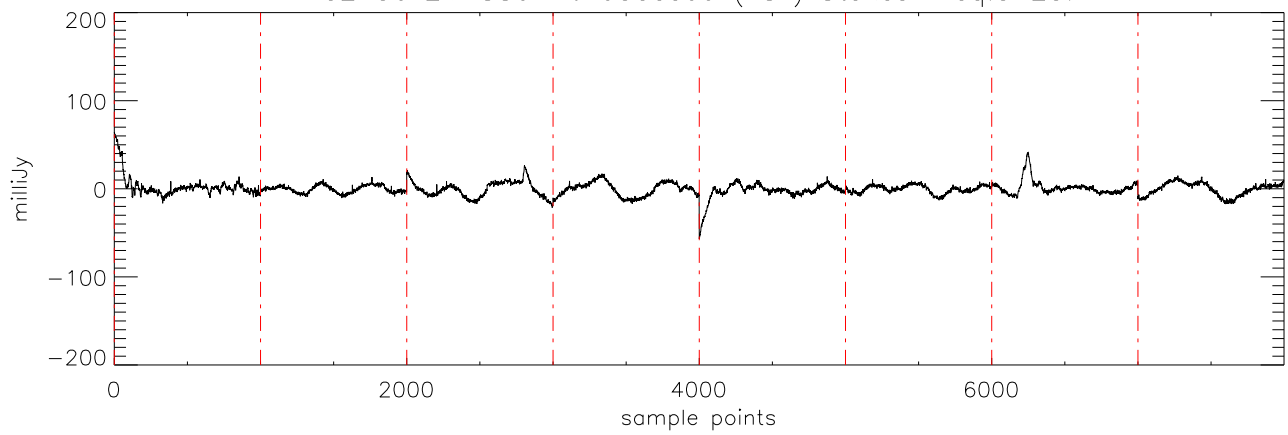
a2430 2MASS0746 03dec09 (AST) StokesI freq:5125.
