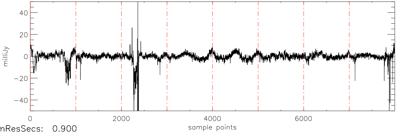
a2430 2MASS0746 03dec09 (AST) StokesQ freq:4405.
