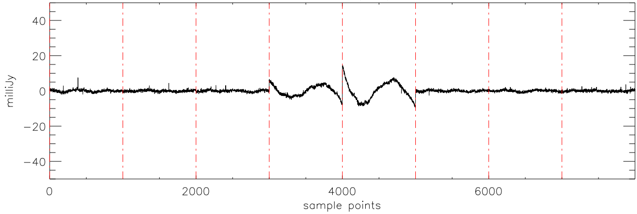
a2430 2MASS0746 03dec09 (AST) StokesU freq:5125.
