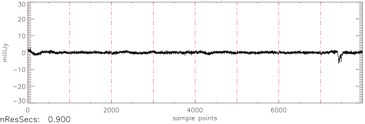
a2430 2MASS0746 03dec09 (AST) StokesV freq:4975.
