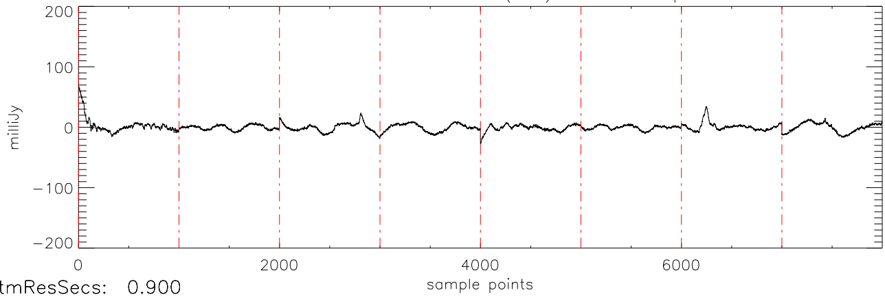
a2430 2MASS0746 03dec09 (AST) StokesI freq:4975.
