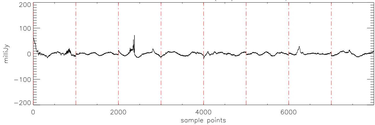
a2430 2MASS0746 03dec09 (AST) StokesI freq:4545.
