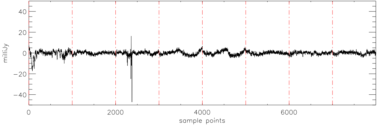
a2430 2MASS0746 03dec09 (AST) StokesQ freq:4545.
