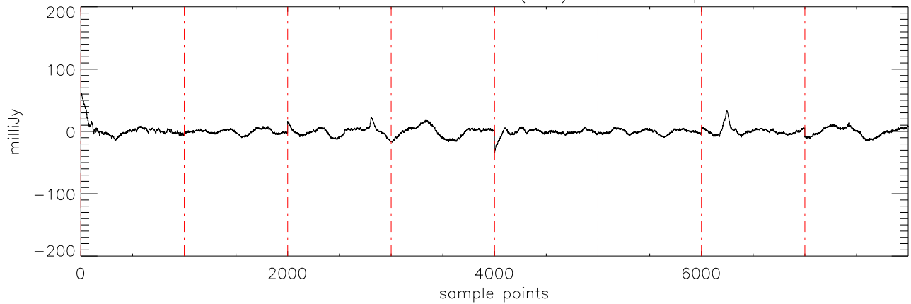
a2430 2MASS0746 03dec09 (AST) StokesI freq:4695.
