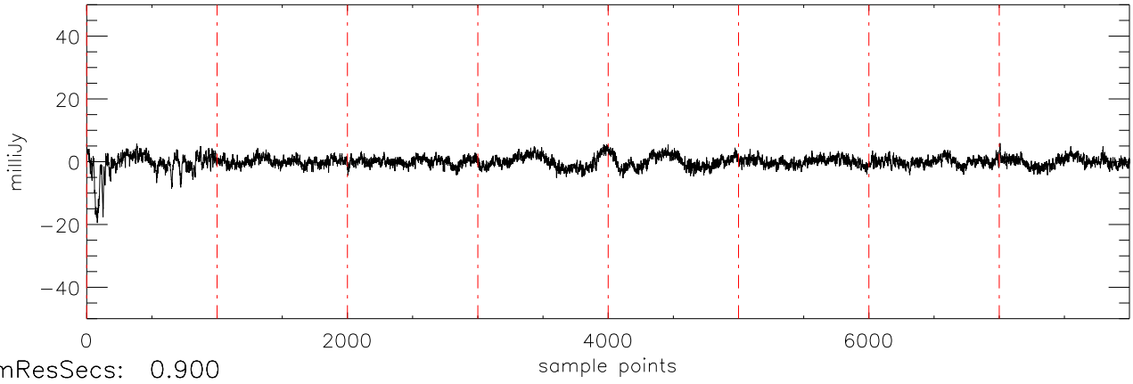
a2430 2MASS0746 03dec09 (AST) StokesQ freq:4975.
