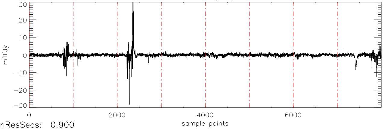
a2430 2MASS0746 03dec09 (AST) StokesV freq:4405.
