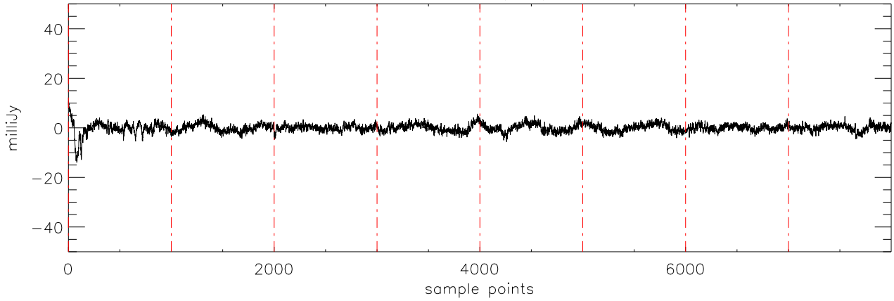
a2430 2MASS0746 03dec09 (AST) StokesQ freq:4695.
