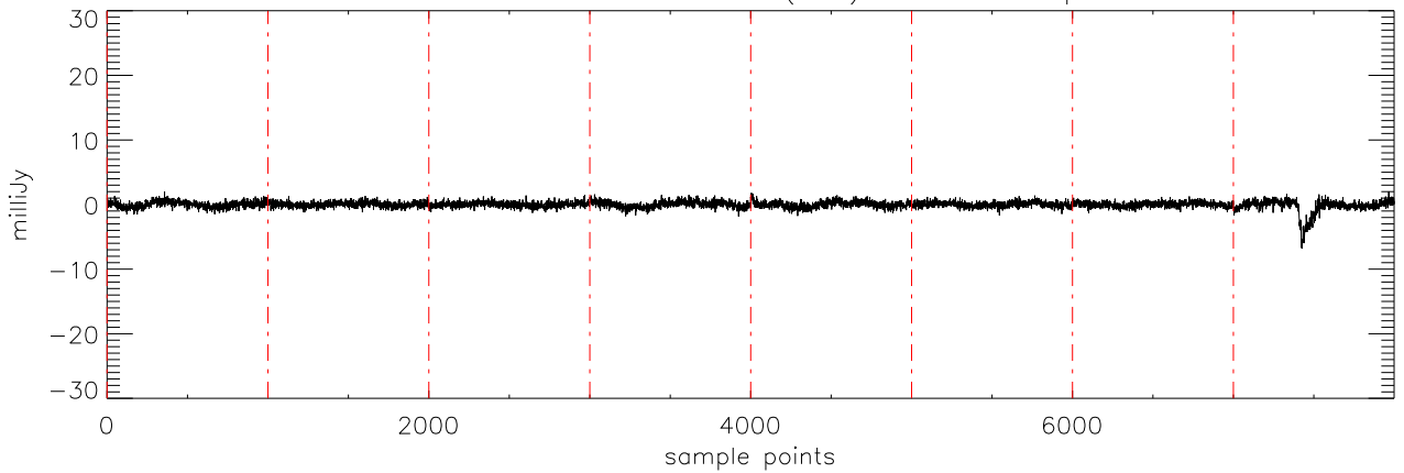
a2430 2MASS0746 03dec09 (AST) StokesV freq:4695.
