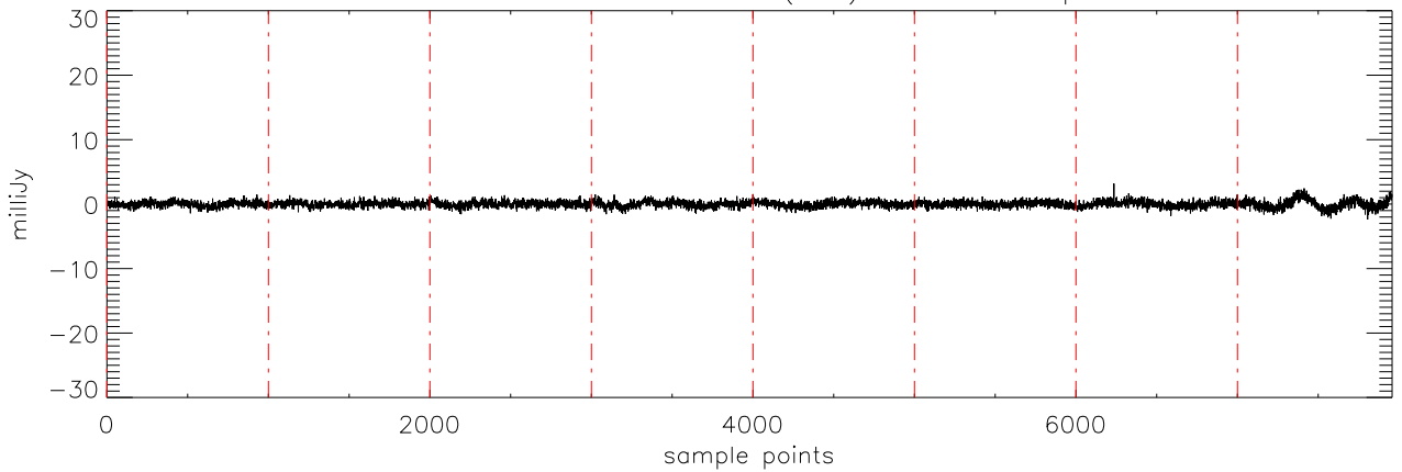
a2430 2MASS0746 02dec09 (AST) StokesV freq:4695.
