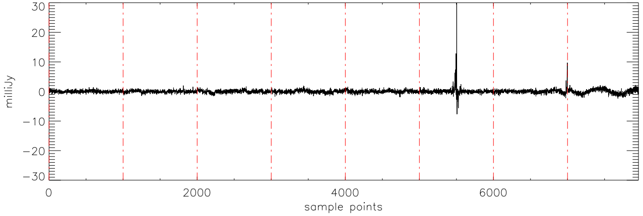
a2430 2MASS0746 02dec09 (AST) StokesV freq:4545.
