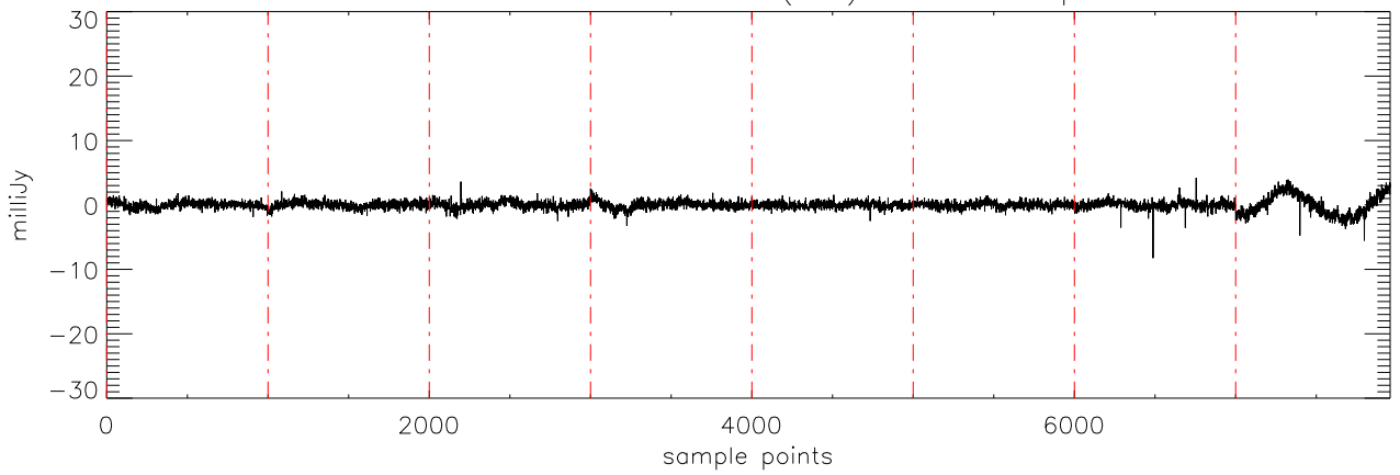
a2430 2MASS0746 02dec09 (AST) StokesV freq:5125.
