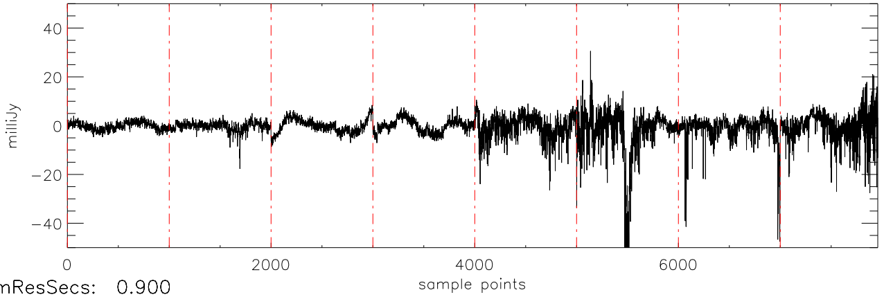
a2430 2MASS0746 02dec09 (AST) StokesQ freq:4405.
