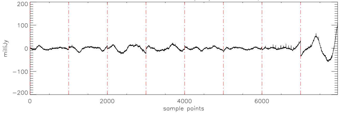
a2430 2MASS0746 02dec09 (AST) StokesI freq:5125.
