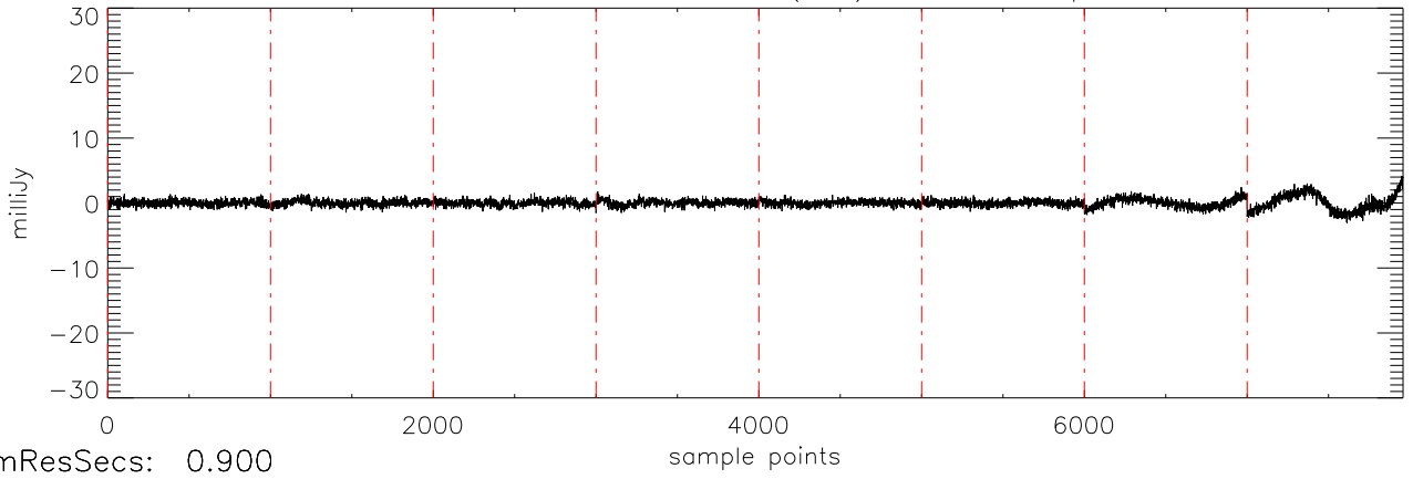
a2430 2MASS0746 02dec09 (AST) StokesV freq:4975.
