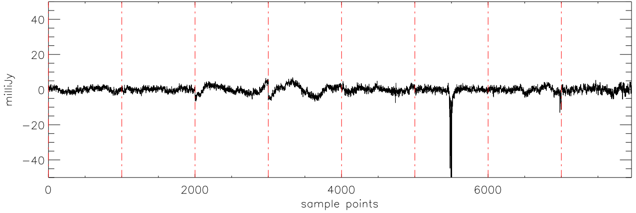
a2430 2MASS0746 02dec09 (AST) StokesQ freq:4545.
