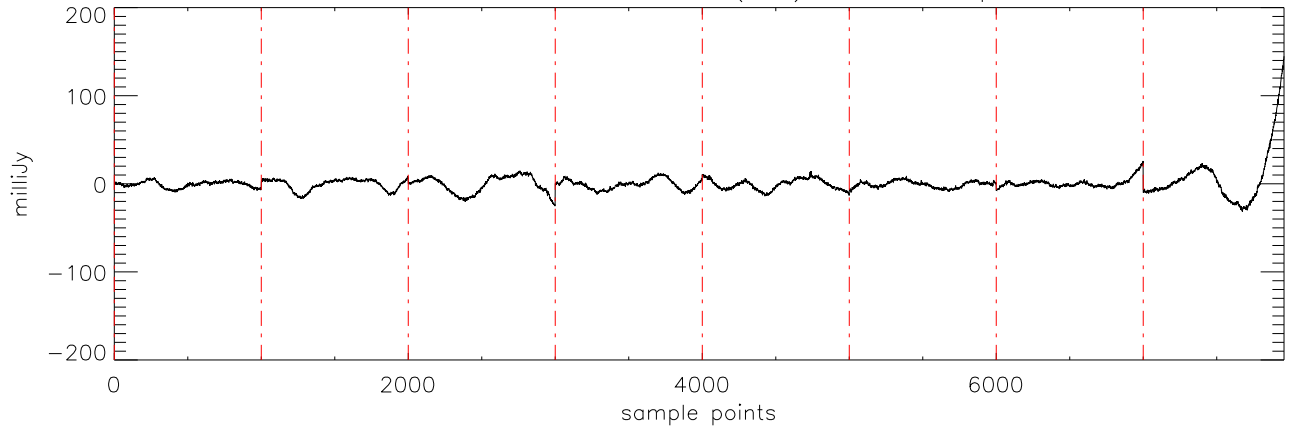
a2430 2MASS0746 02dec09 (AST) StokesI freq:4695.
