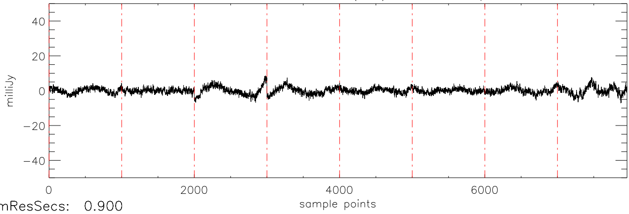
a2430 2MASS0746 02dec09 (AST) StokesQ freq:4975.
