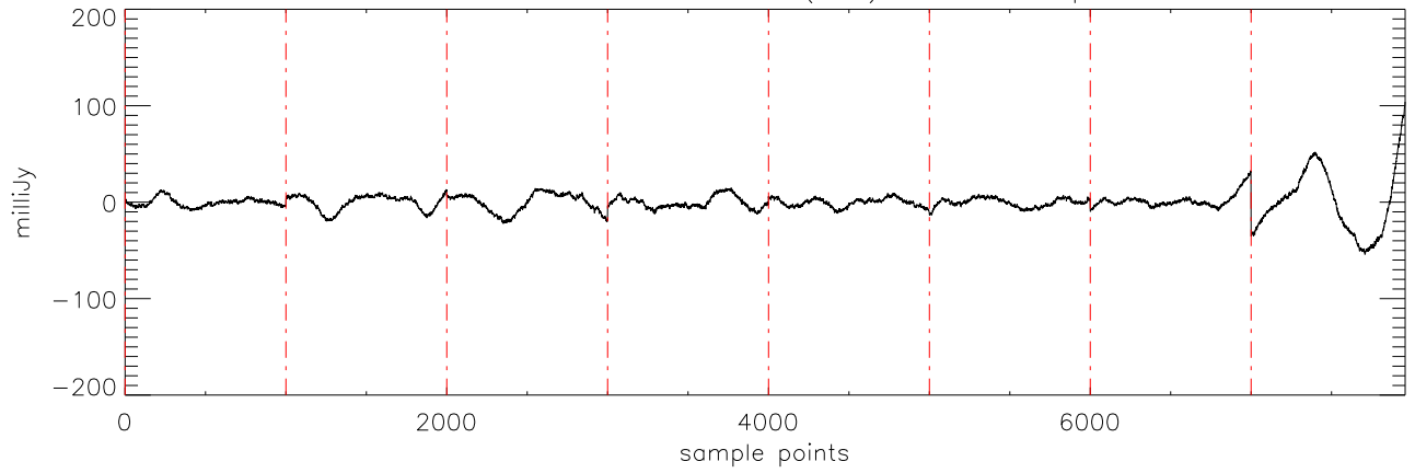
a2430 2MASS0746 02dec09 (AST) StokesI freq:5125.
