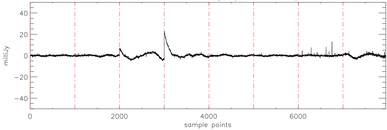
a2430 2MASS0746 02dec09 (AST) StokesU freq:5125.
