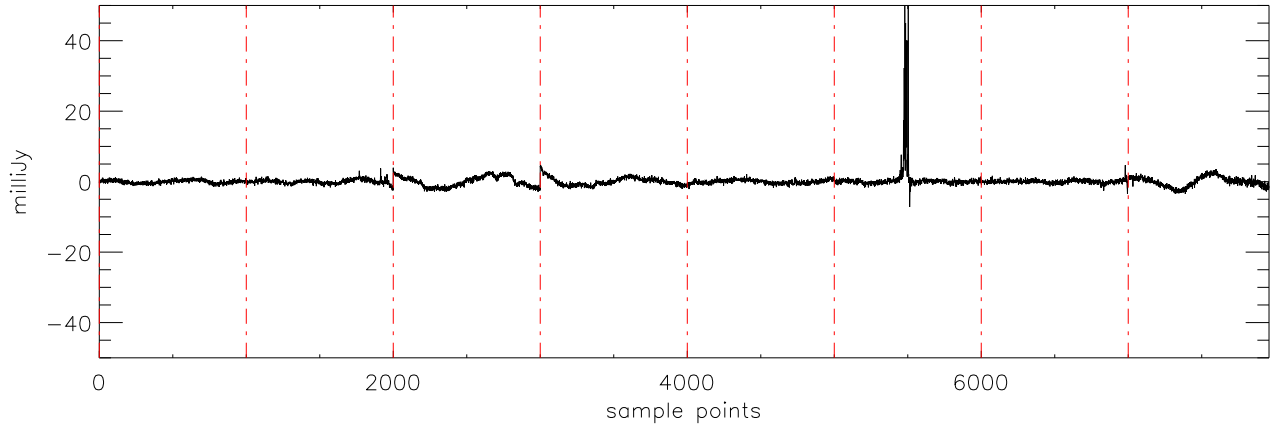
a2430 2MASS0746 02dec09 (AST) StokesU freq:4545.
