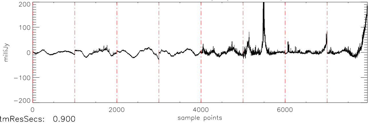
a2430 2MASS0746 02dec09 (AST) StokesI freq:4405.
