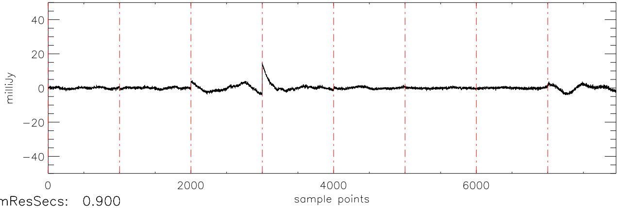
a2430 2MASS0746 02dec09 (AST) StokesU freq:4975.
