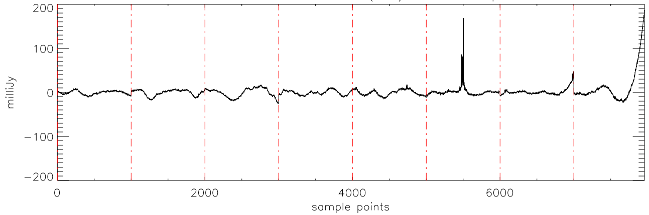
a2430 2MASS0746 02dec09 (AST) StokesI freq:4545.
