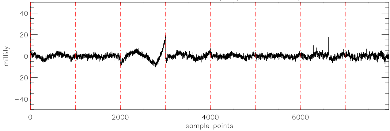
a2430 2MASS0746 02dec09 (AST) StokesQ freq:5125.
