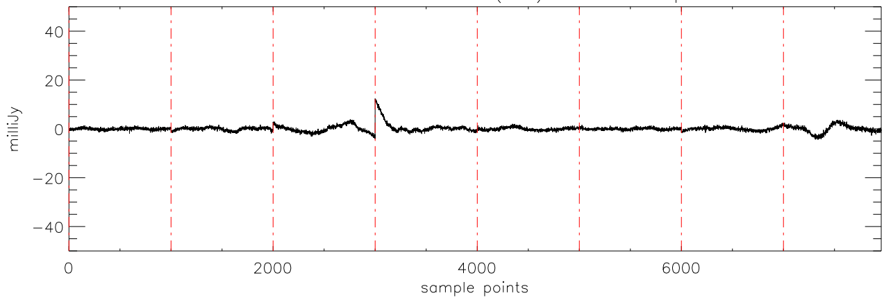
a2430 2MASS0746 02dec09 (AST) StokesU freq:4695.
