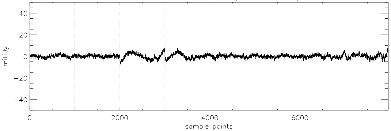
a2430 2MASS0746 02dec09 (AST) StokesQ freq:4695.
