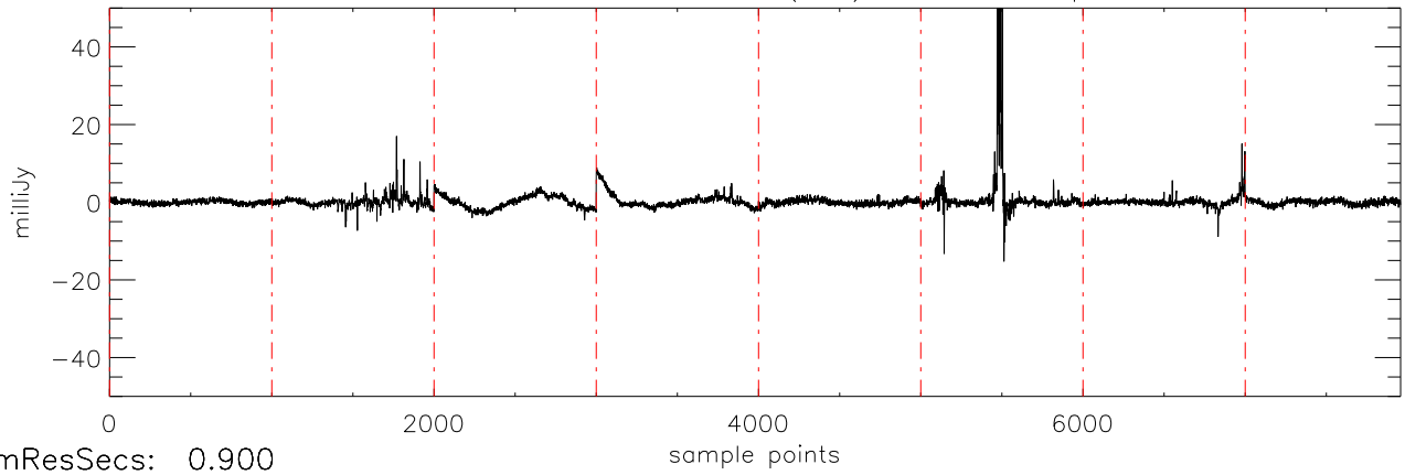
a2430 2MASS0746 02dec09 (AST) StokesU freq:4405.
