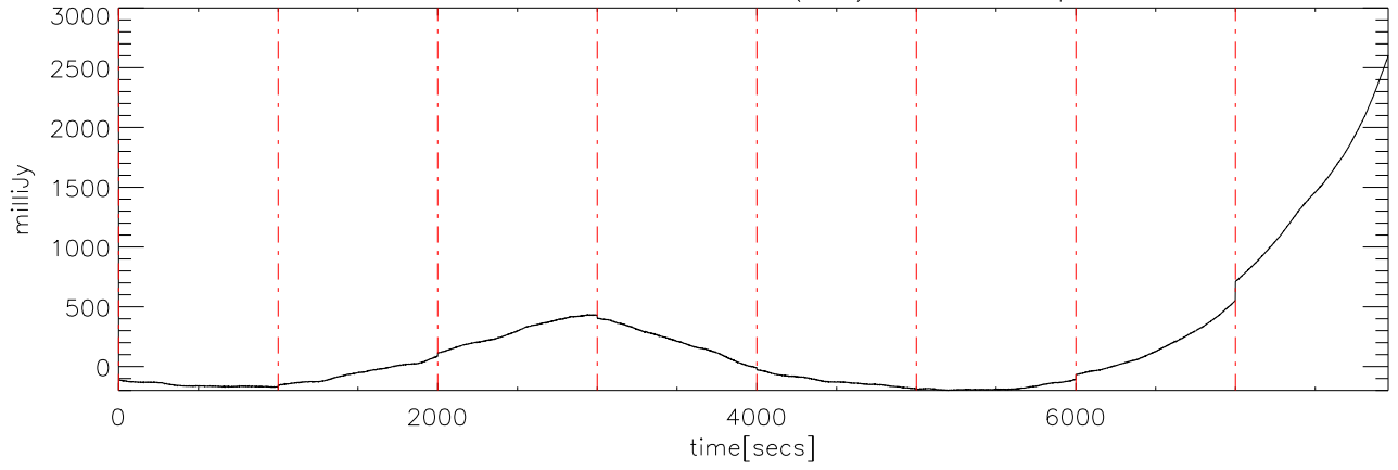
a2430 2MASS0746 02dec09 (AST) StokesI freq:4975.
