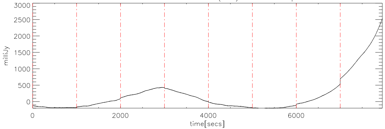
α2430 2MASS0746 02dec09 (AST) StokesI freq:4695.
