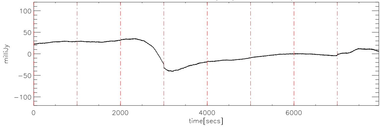
a2430 2MASS0746 02dec09 (AST) StokesU freq:4975.
