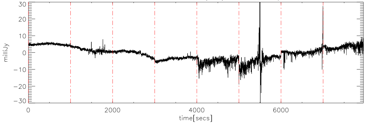
a2430 2MASS0746 02dec09 (AST) StokesV freq:4405.
