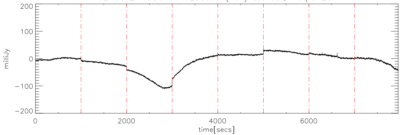
a2430 2MASS0746 02dec09 (AST) StokesQ freq:5125.
