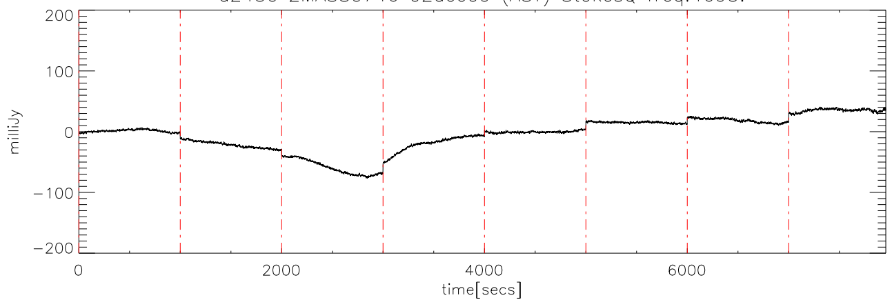
a2430 2MASS0746 02dec09 (AST) StokesQ freq:4695.
