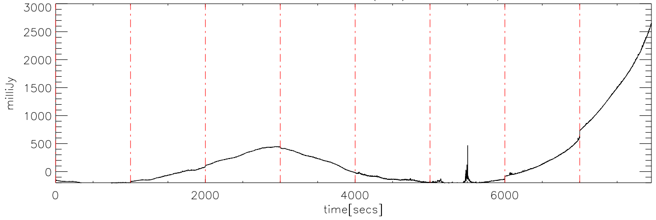
α2430 2MASS0746 02dec09 (AST) StokesI freq:4405.
