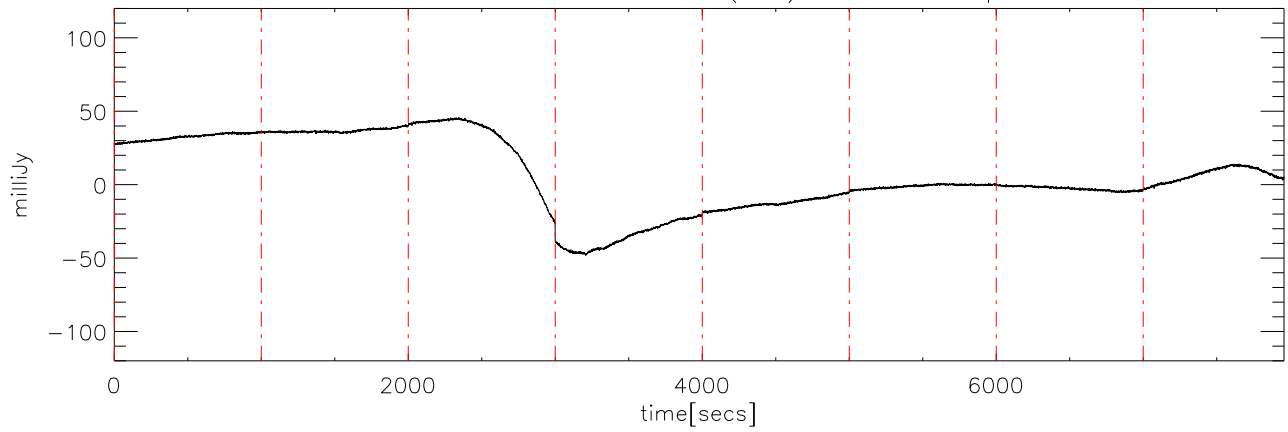
a2430 2MASS0746 02dec09 (AST) StokesU freq:5125.
