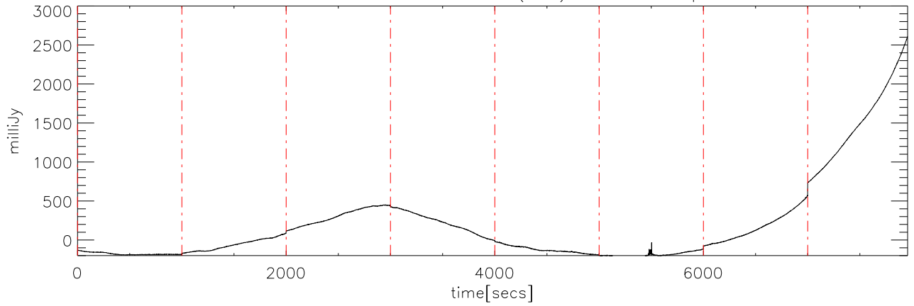
α2430 2MASS0746 02dec09 (AST) StokesI freq:4545.
