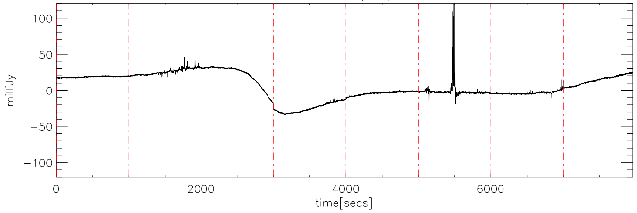
a2430 2MASS0746 02dec09 (AST) StokesU freq:4405.
