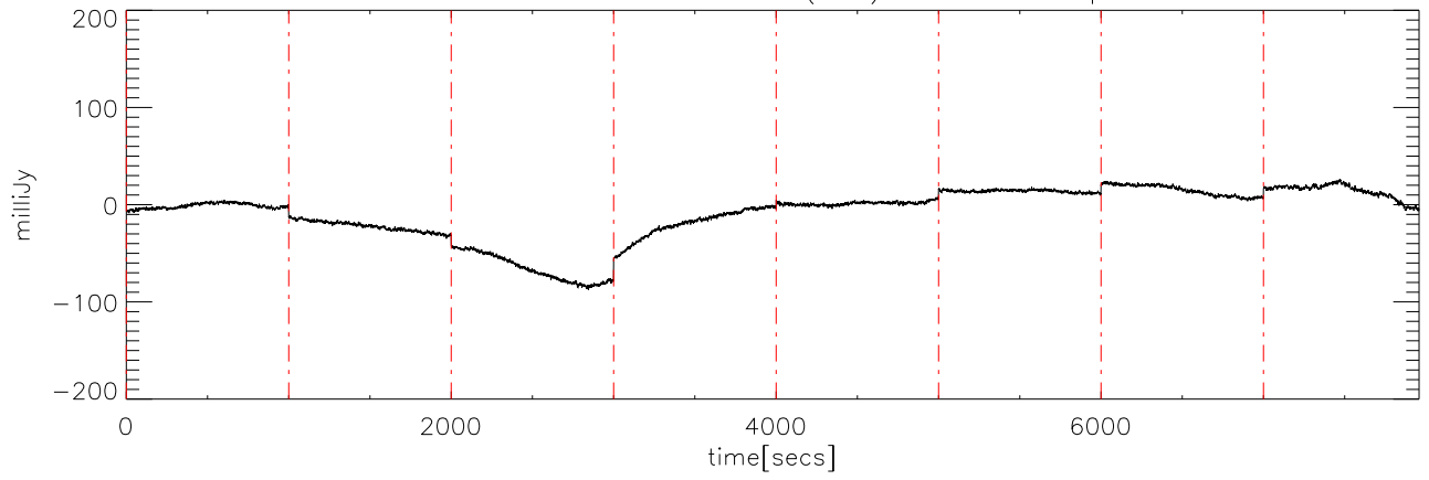
a2430 2MASS0746 02dec09 (AST) StokesQ freq:4975.
