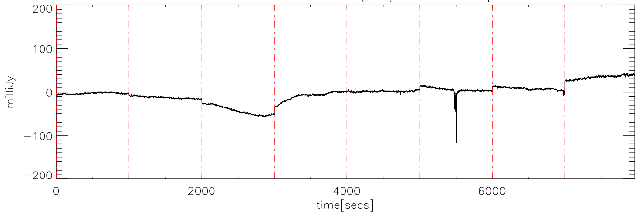
a2430 2MASS0746 02dec09 (AST) StokesQ freq:4545.
