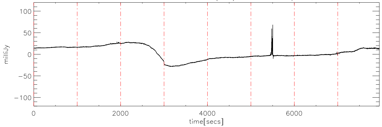
a2430 2MASS0746 02dec09 (AST) StokesU freq:4545.
