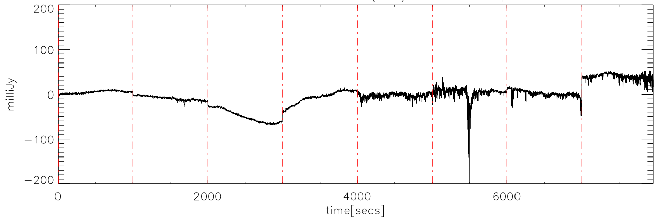
a2430 2MASS0746 02dec09 (AST) StokesQ freq:4405.
