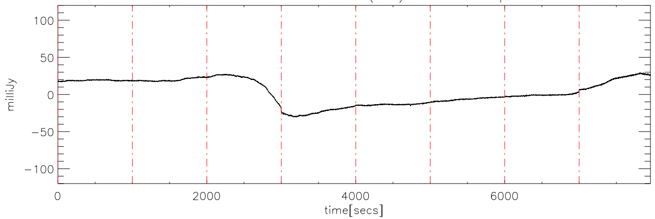
a2430 2MASS0746 02dec09 (AST) StokesU freq:4695.
