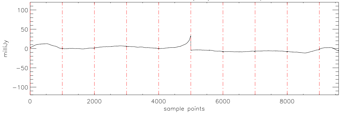
a2430 2MASS0036 04dec09 (AST) StokesU freq:5125.
