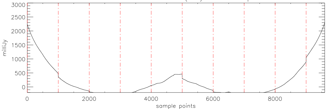
a2430 2MASS0036 04dec09 (AST) StokesI freq:4695.
