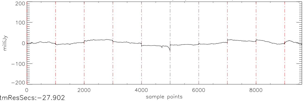
a2430 2MASS0036 04dec09 (AST) StokesQ freq:4975.
