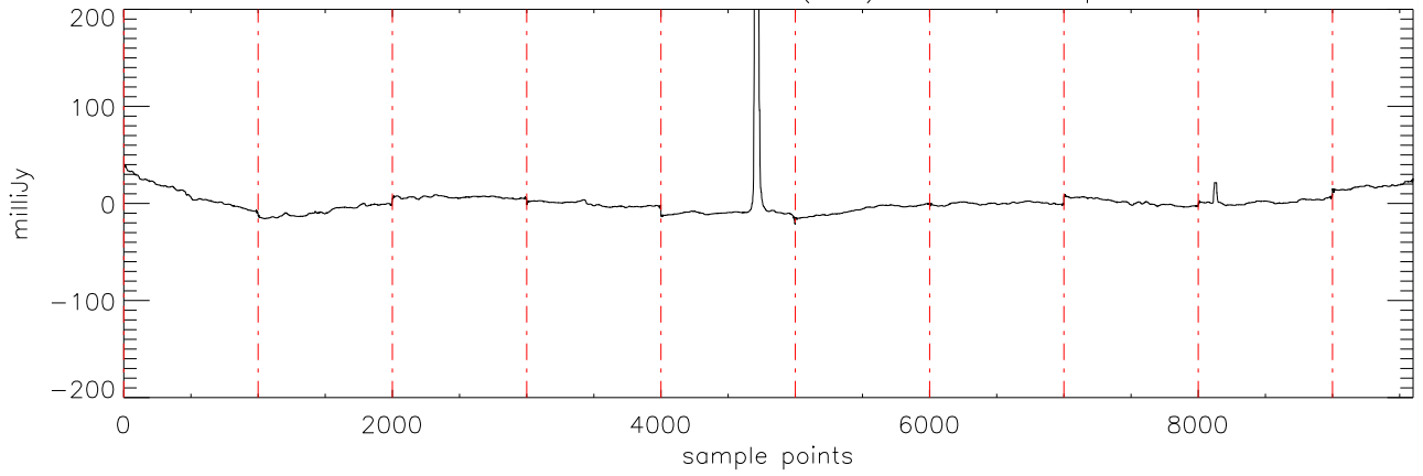
a2430 2MASS0036 04dec09 (AST) StokesQ freq:4545.
