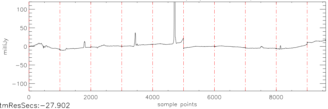
a2430 2MASS0036 04dec09 (AST) StokesU freq:4405.
