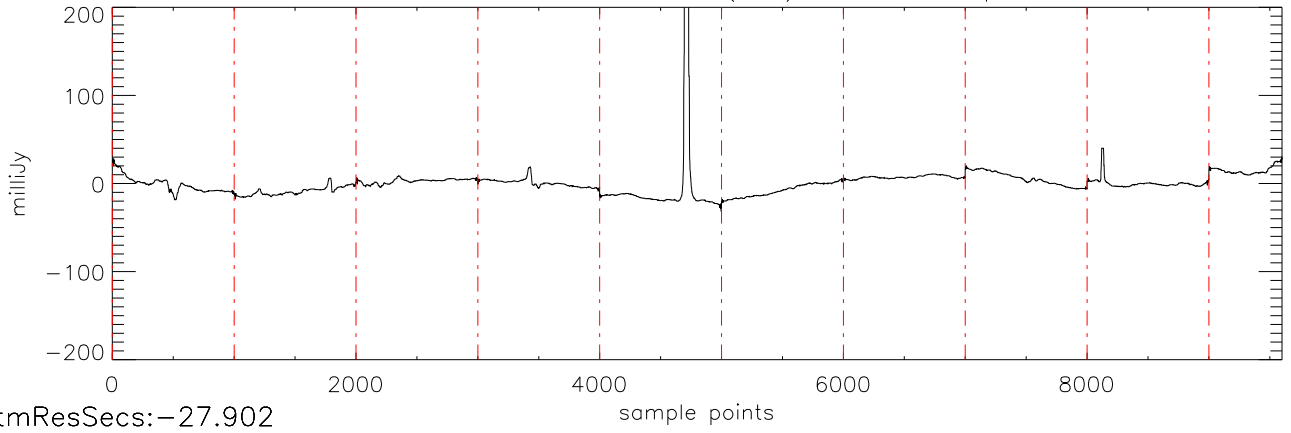
a2430 2MASS0036 04dec09 (AST) StokesQ freq:4405.
