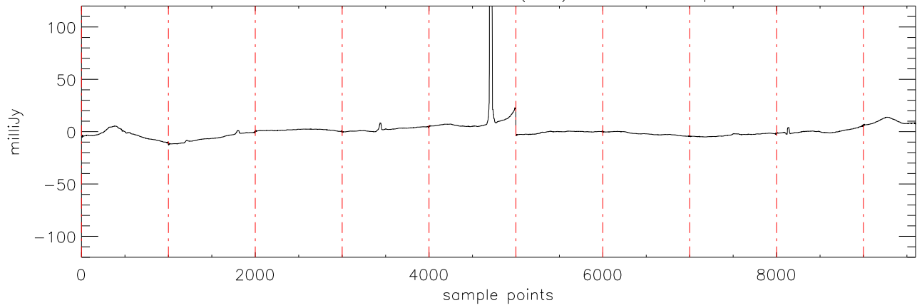
a2430 2MASS0036 04dec09 (AST) StokesU freq:4545.
