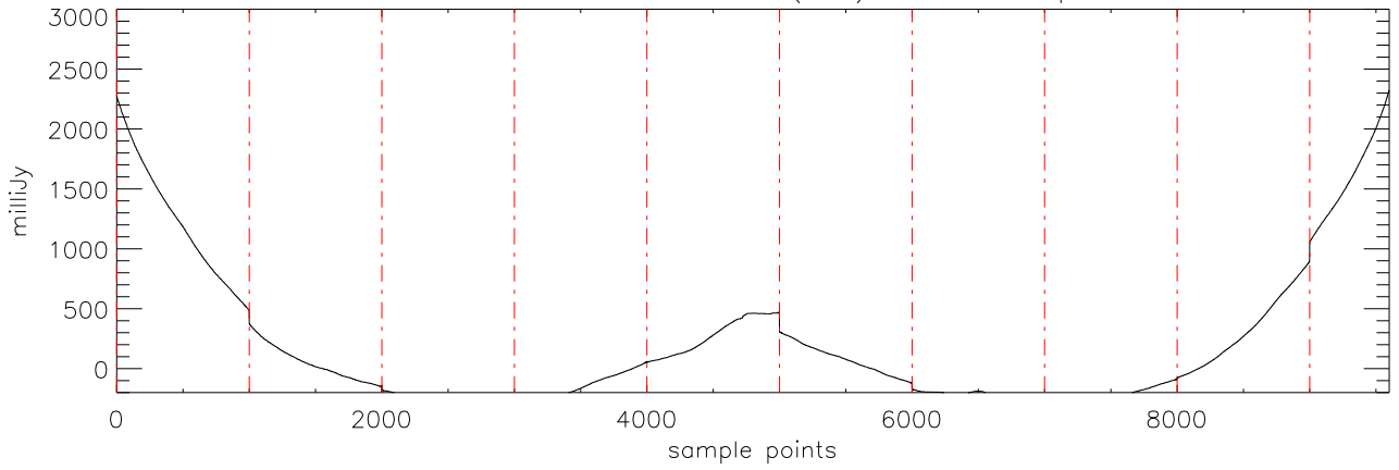
a2430 2MASS0036 04dec09 (AST) StokesI freq:5125.
