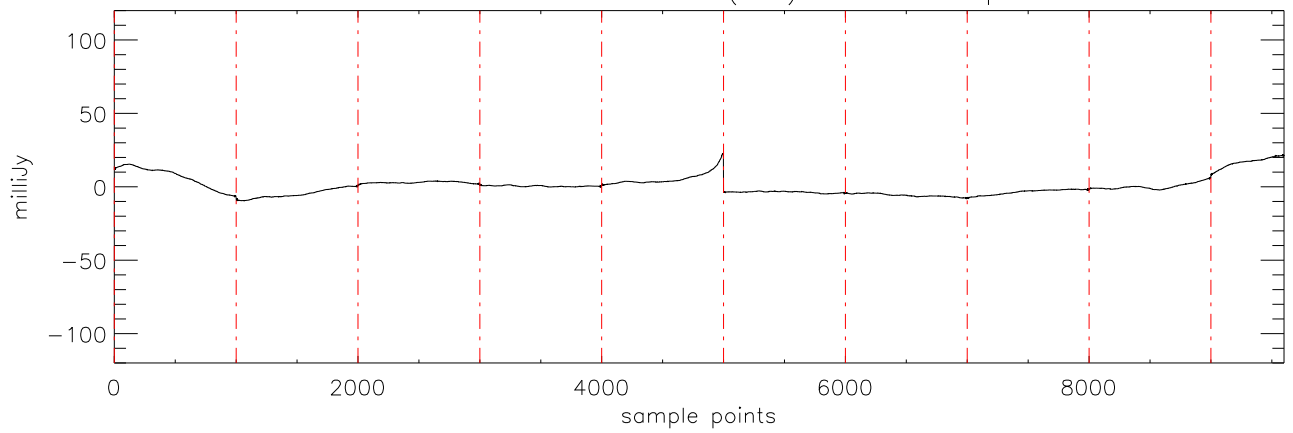
a2430 2MASS0036 04dec09 (AST) StokesU freq:4695.
