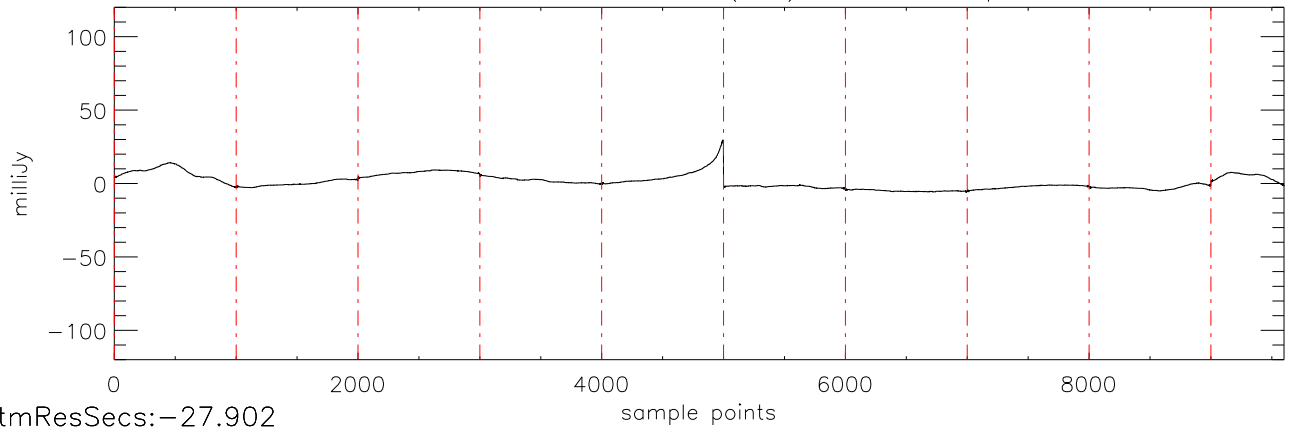
a2430 2MASS0036 04dec09 (AST) StokesU freq:4975.
