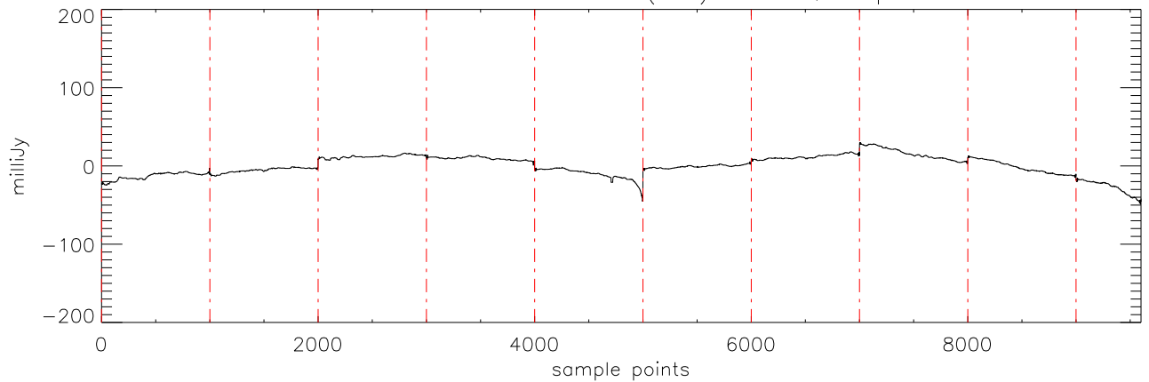
a2430 2MASS0036 04dec09 (AST) StokesQ freq:5125.
