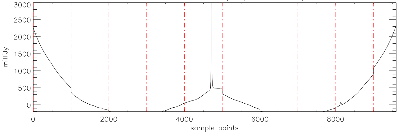
a2430 2MASS0036 04dec09 (AST) StokesI freq:4545.
