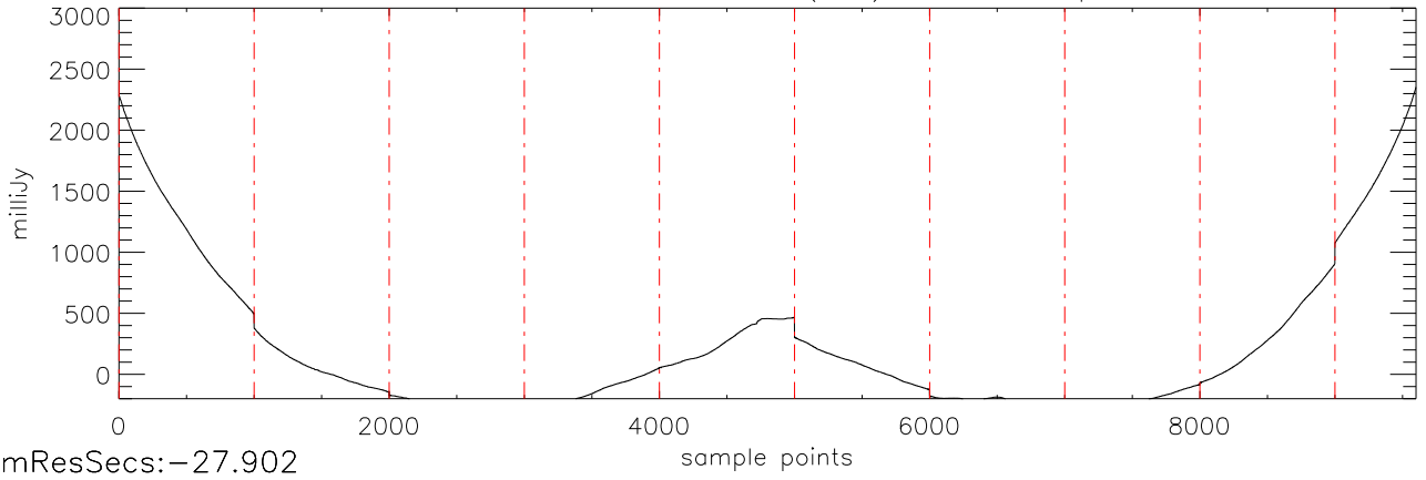
a2430 2MASS0036 04dec09 (AST) StokesI freq:4975.
