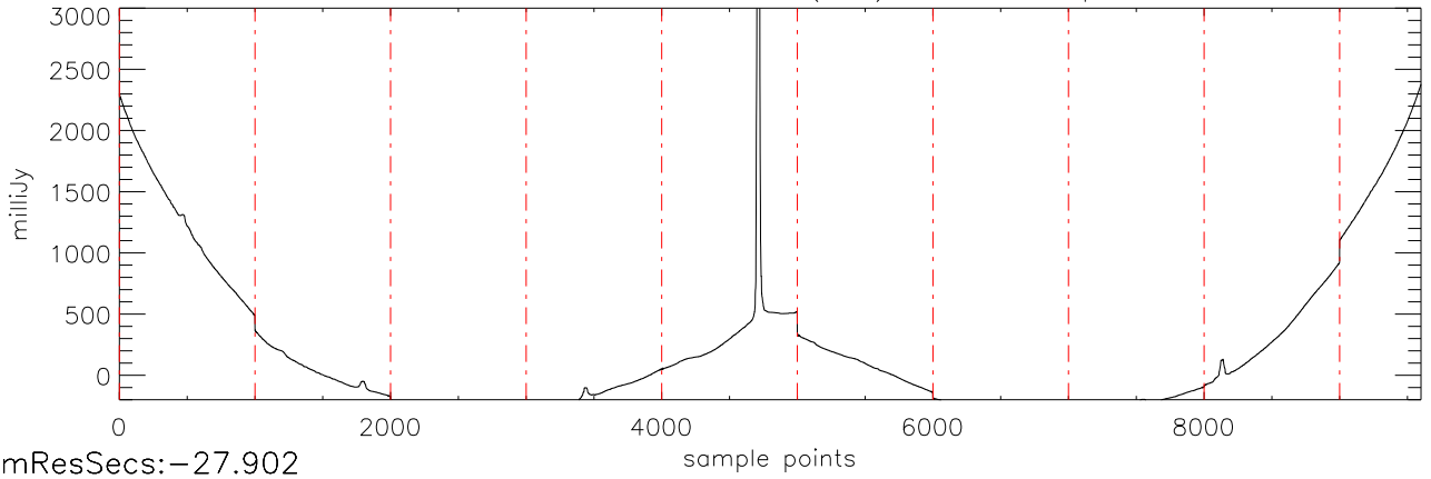
a2430 2MASS0036 04dec09 (AST) StokesI freq:4405.
