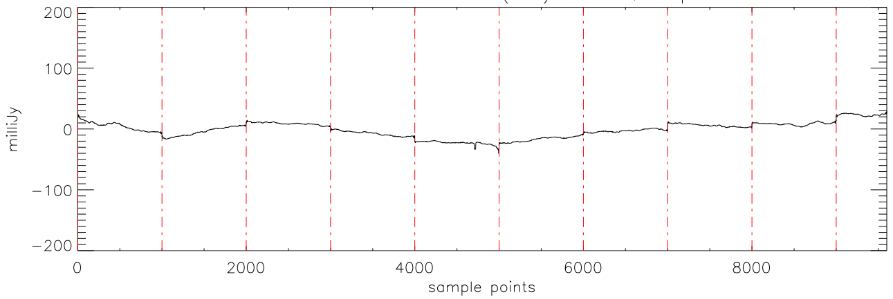
a2430 2MASS0036 04dec09 (AST) StokesQ freq:4695.
