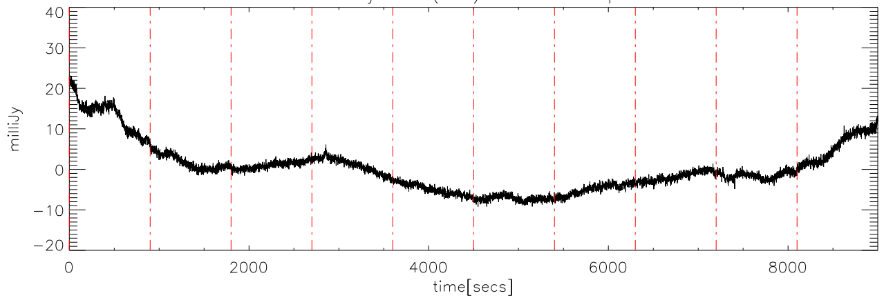
a2414 12jun09 (AST) StokesV freq:4725.
