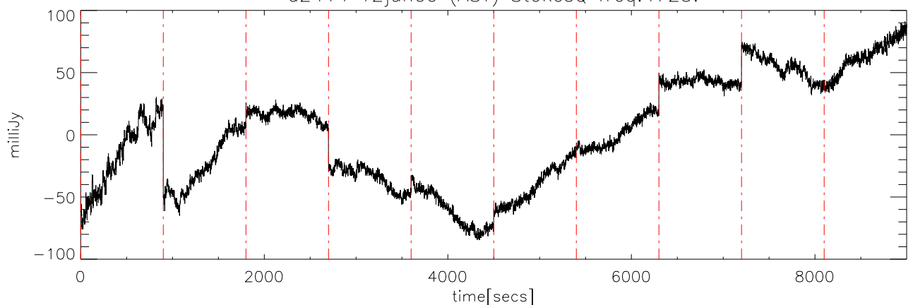
a2414 12jun09 (AST) StokesQ freq:4725.
