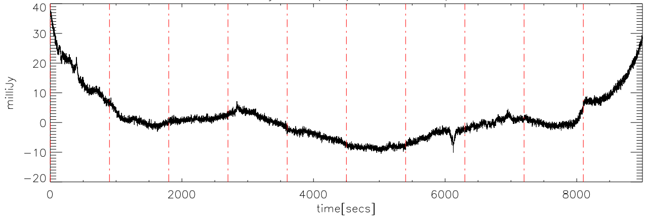
a2414 12jun09 (AST) StokesV freq:5000.
