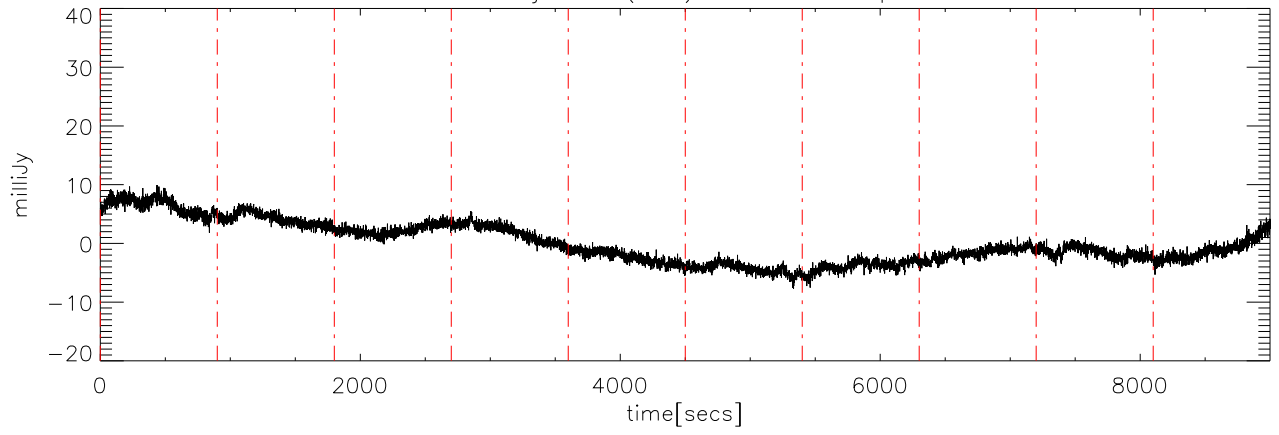
a2414 12jun09 (AST) StokesV freq:4600.
