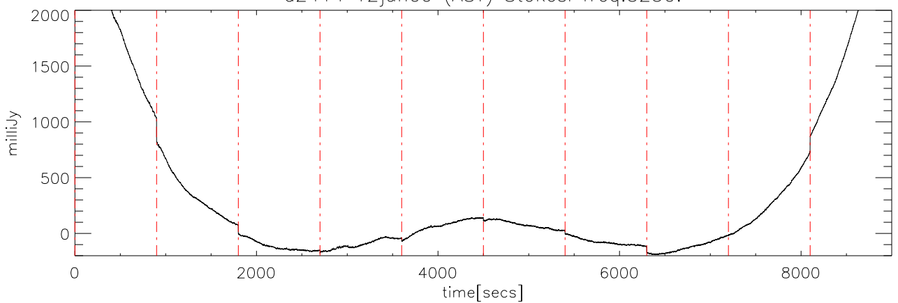
a2414 12jun09 (AST) StokesI freq:5250.
