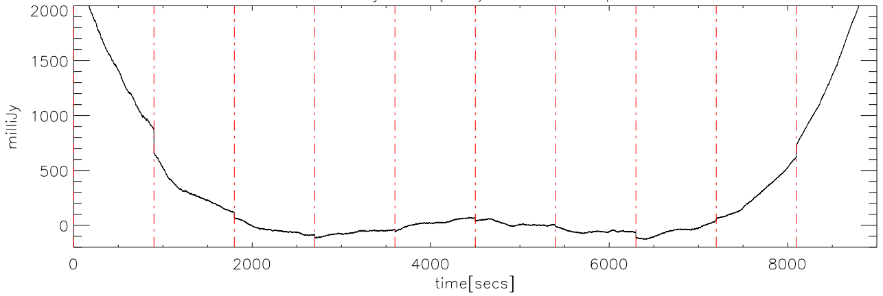
a2414 12jun09 (AST) StokesI freq:4600.
