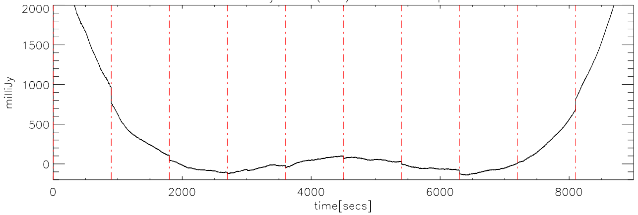
a2414 12jun09 (AST) StokesI freq:5125.
