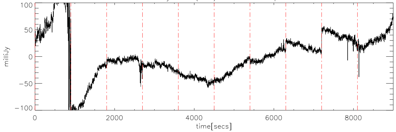
a2414 12jun09 (AST) StokesQ freq:4475.
