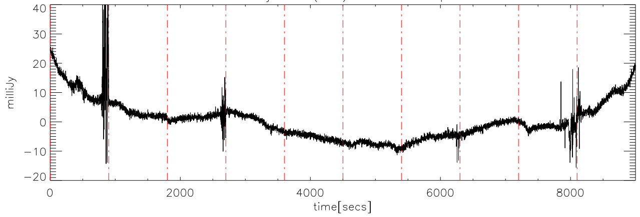
a2414 12jun09 (AST) StokesV freq:4475.
