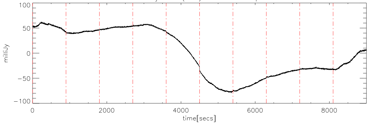
a2414 12jun09 (AST) StokesU freq:5125.
