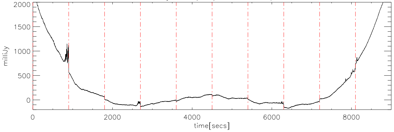
a2414 12jun09 (AST) StokesI freq:4475.
