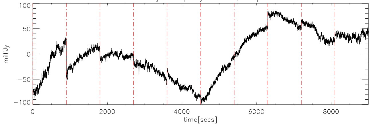
a2414 12jun09 (AST) StokesQ freq:5250.
