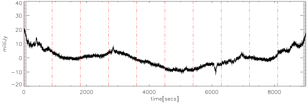
a2414 12jun09 (AST) StokesV freq:5125.
