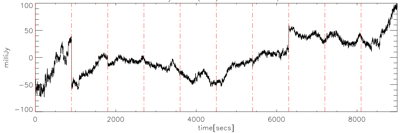
a2414 12jun09 (AST) StokesQ freq:4600.
