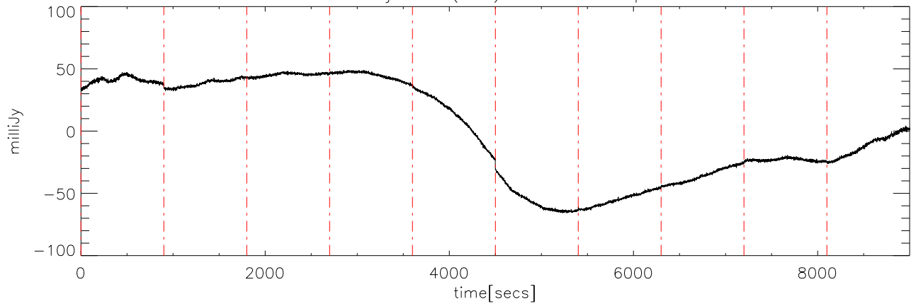
a2414 12jun09 (AST) StokesU freq:5000.
