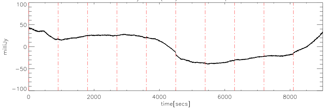
a2414 12jun09 (AST) StokesU freq:4600.
