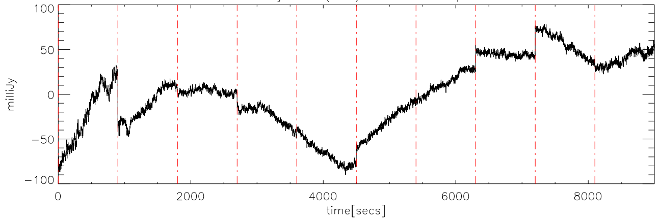
a2414 12jun09 (AST) StokesQ freq:5000.
