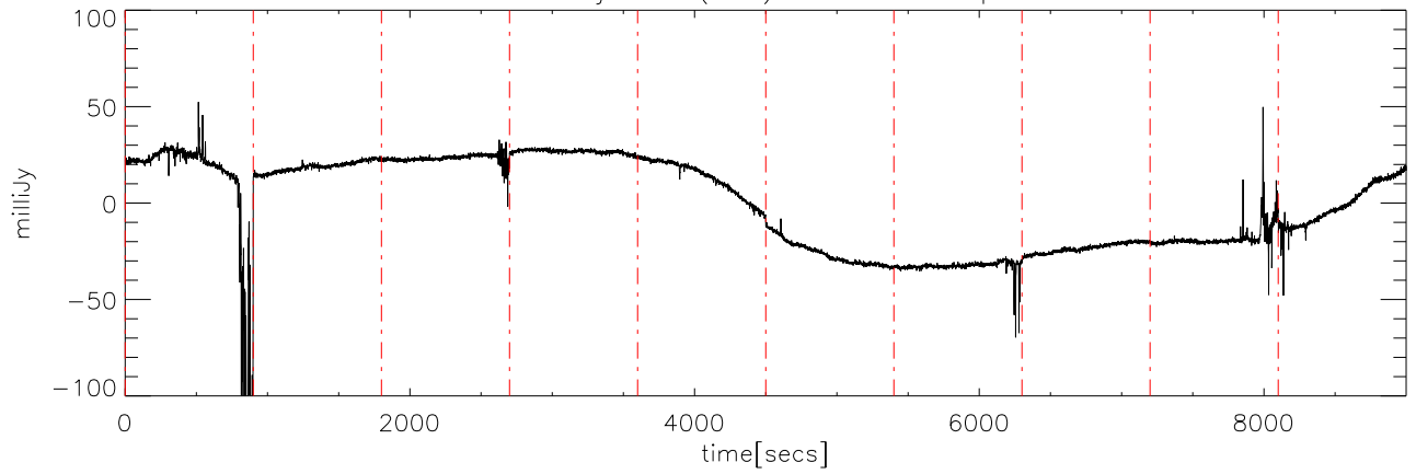
a2414 12jun09 (AST) StokesU freq:4475.
