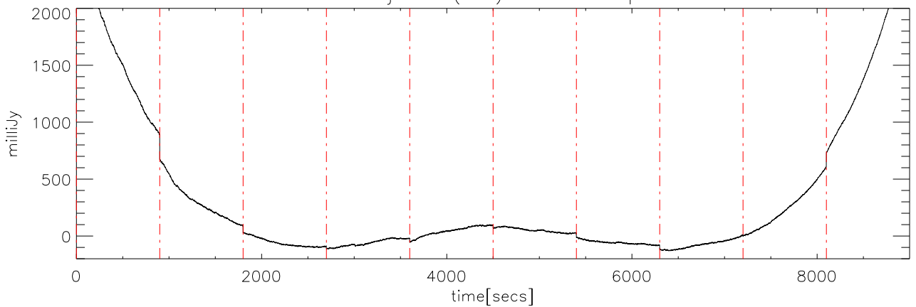
a2414 12jun09 (AST) StokesI freq:4725.
