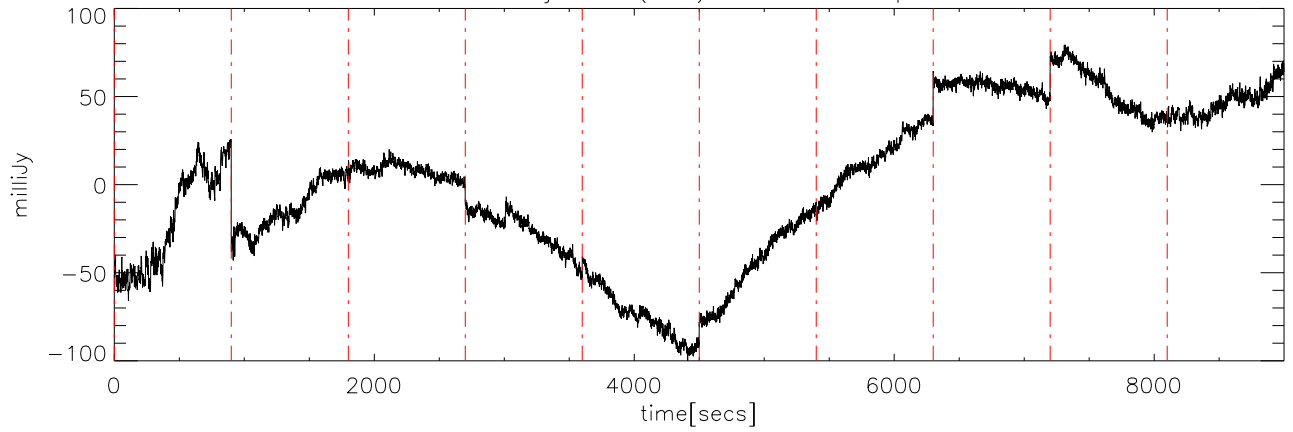
a2414 12jun09 (AST) StokesQ freq:5125.
