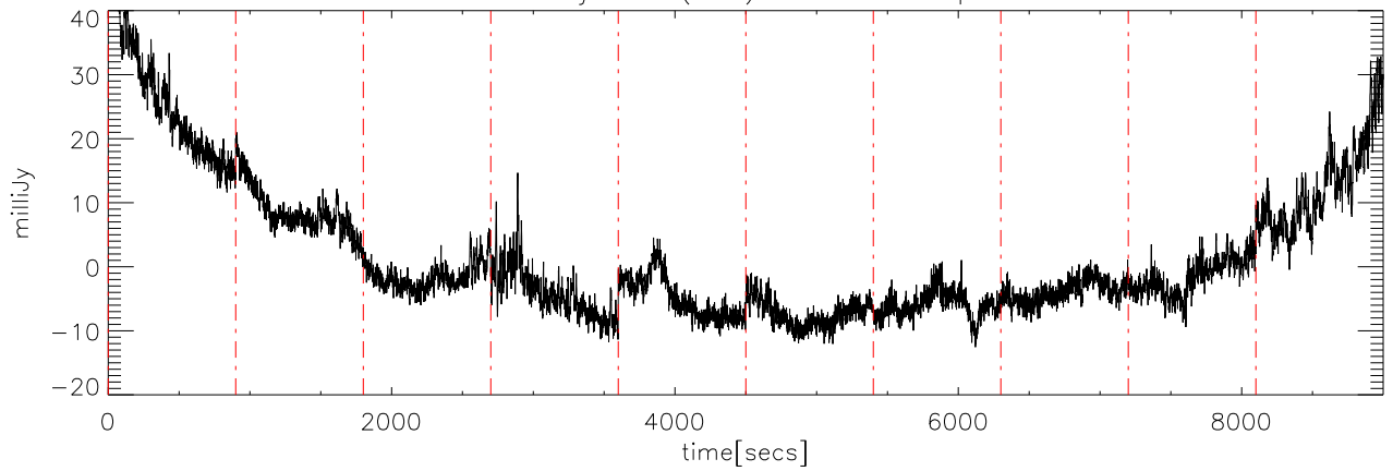
a2414 12jun09 (AST) StokesV freq:5250.
