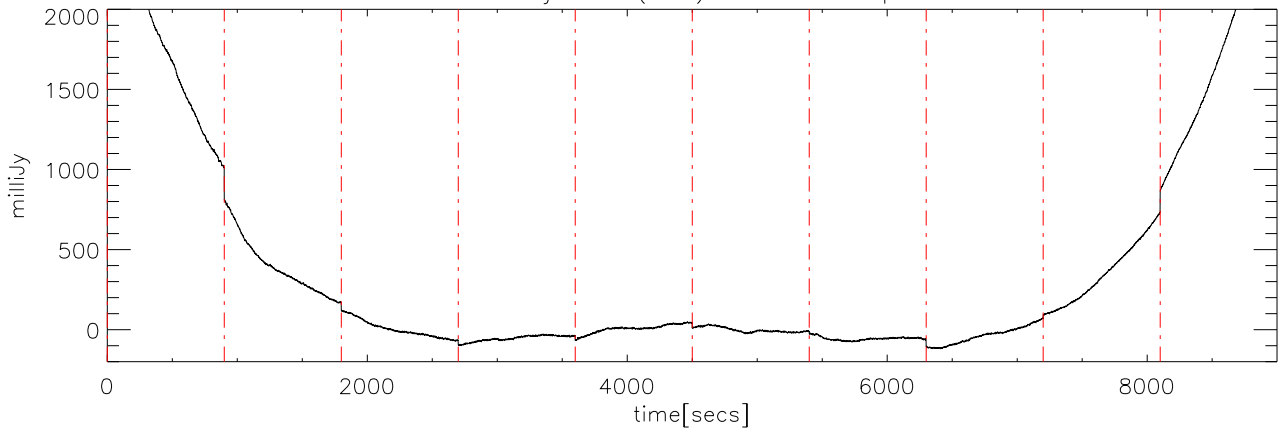
a2414 12jun09 (AST) StokesI freq:5000.
