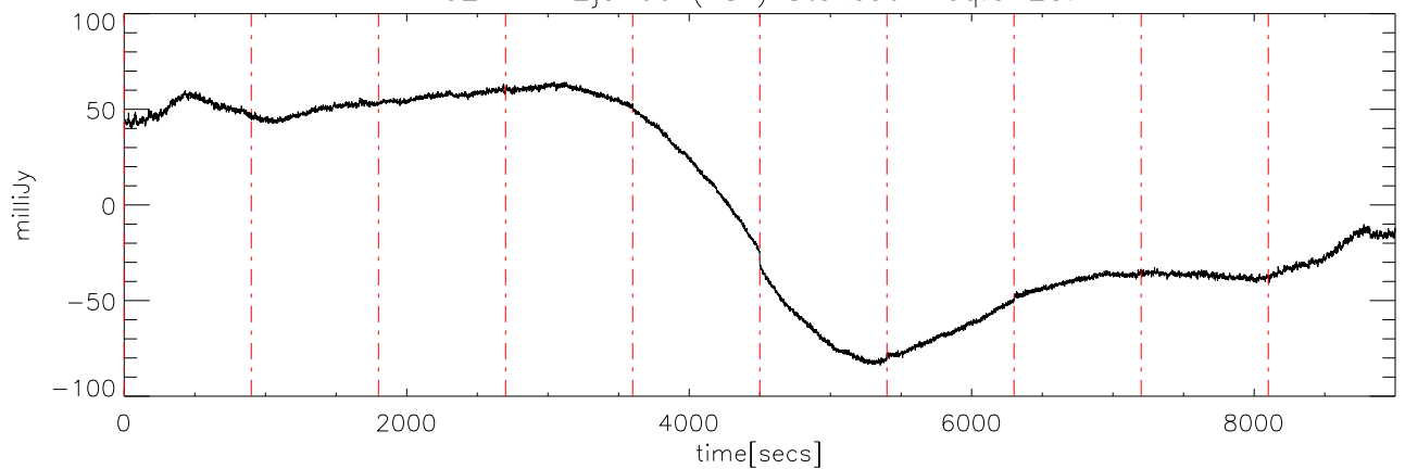
a2414 12jun09 (AST) StokesU freq:5250.
