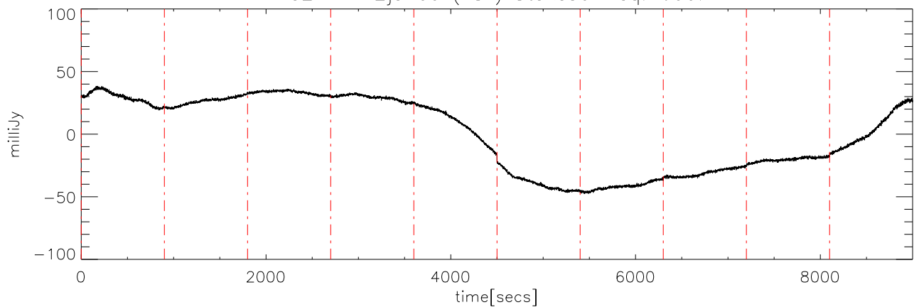
a2414 12jun09 (AST) StokesU freq:4725.
