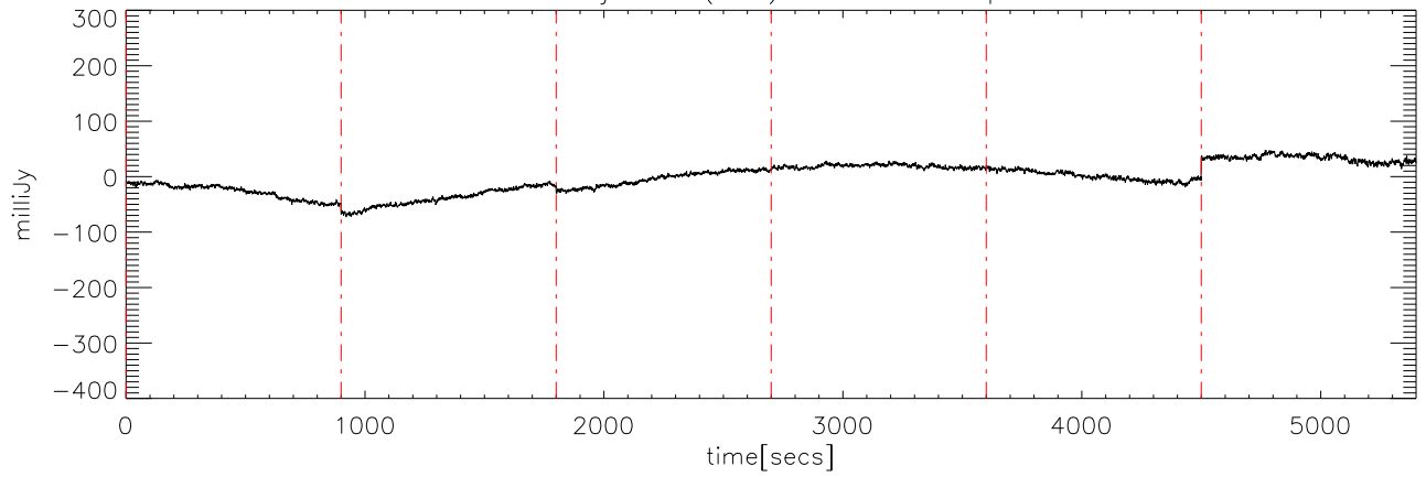
a2414 07jun09 (AST) StokesQ freq:5000.
