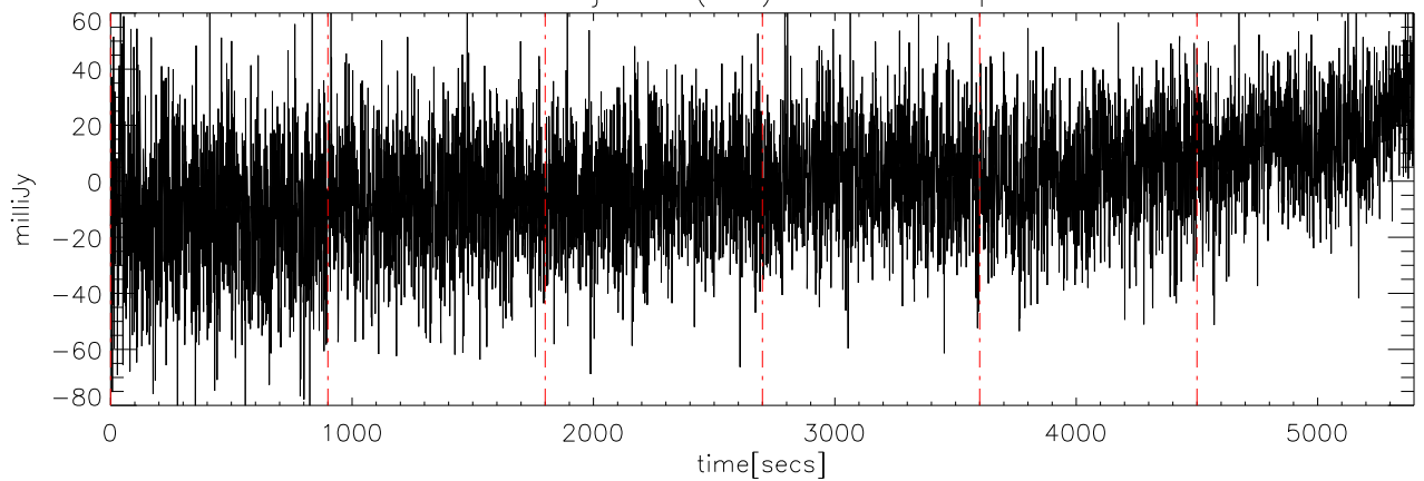
a2414 07jun09 (AST) StokesV freq:4725.
