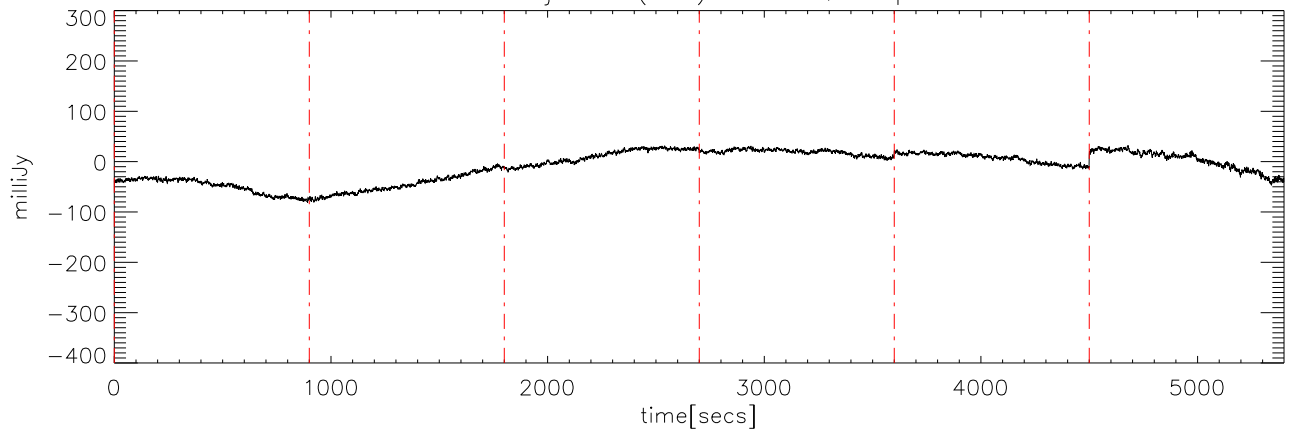
a2414 07jun09 (AST) StokesQ freq:5250.
