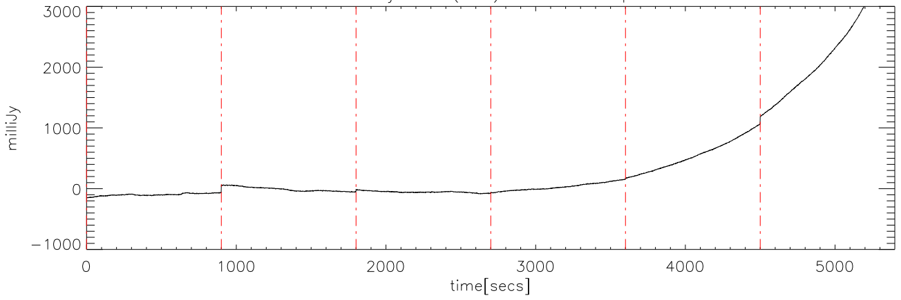
a2414 07jun09 (AST) StokesI freq:5000.
