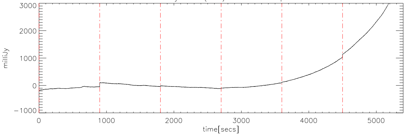
a2414 07jun09 (AST) StokesI freq:5125.
