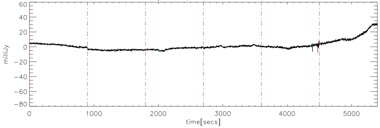
a2414 07jun09 (AST) StokesV freq:4475.
