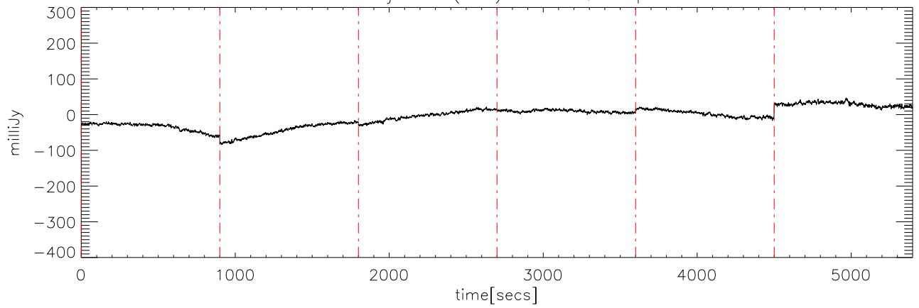
a2414 07jun09 (AST) StokesQ freq:5125.
