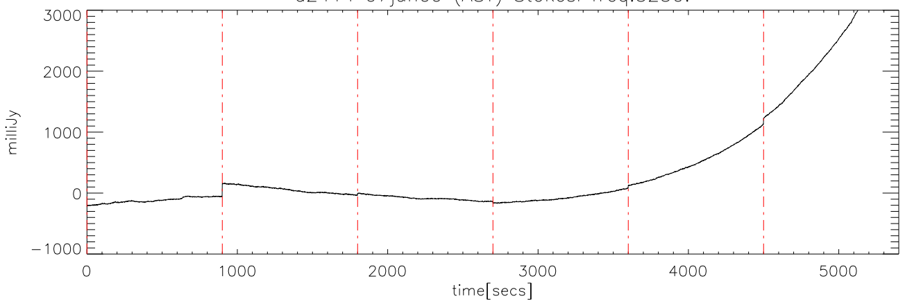
a2414 07jun09 (AST) StokesI freq:5250.
