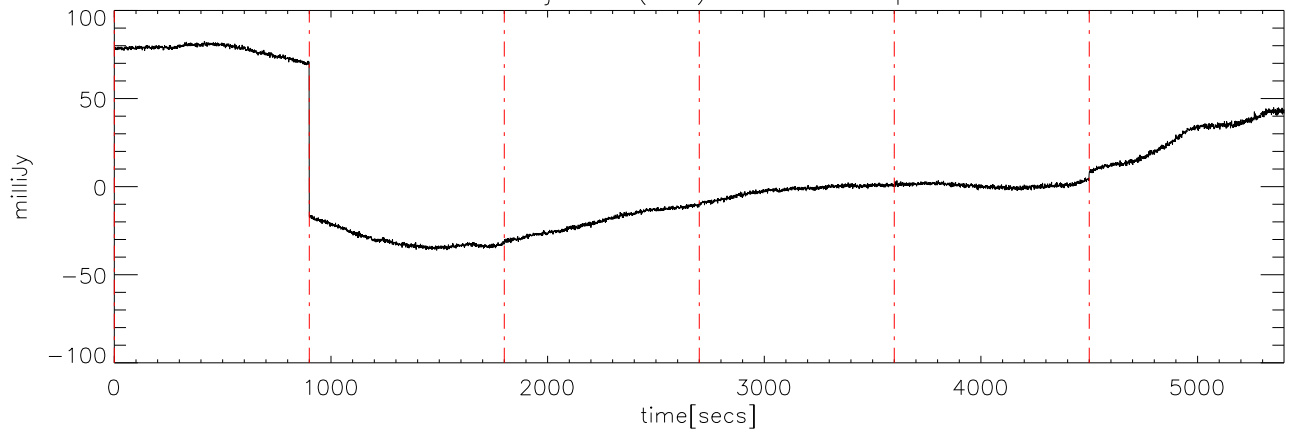
a2414 07jun09 (AST) StokesU freq:5125.
