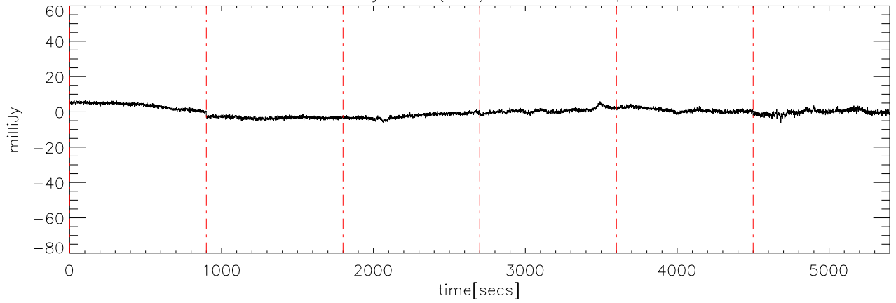
a2414 07jun09 (AST) StokesV freq:4600.
