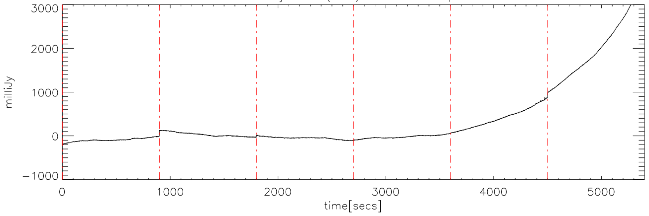
a2414 07jun09 (AST) StokesI freq:4475.
