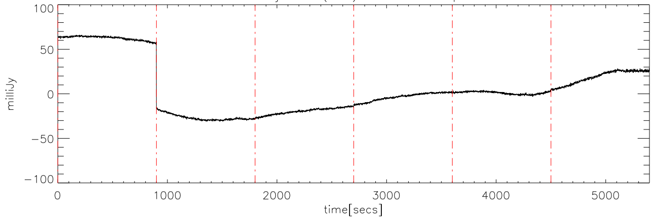
a2414 07jun09 (AST) StokesU freq:5000.
