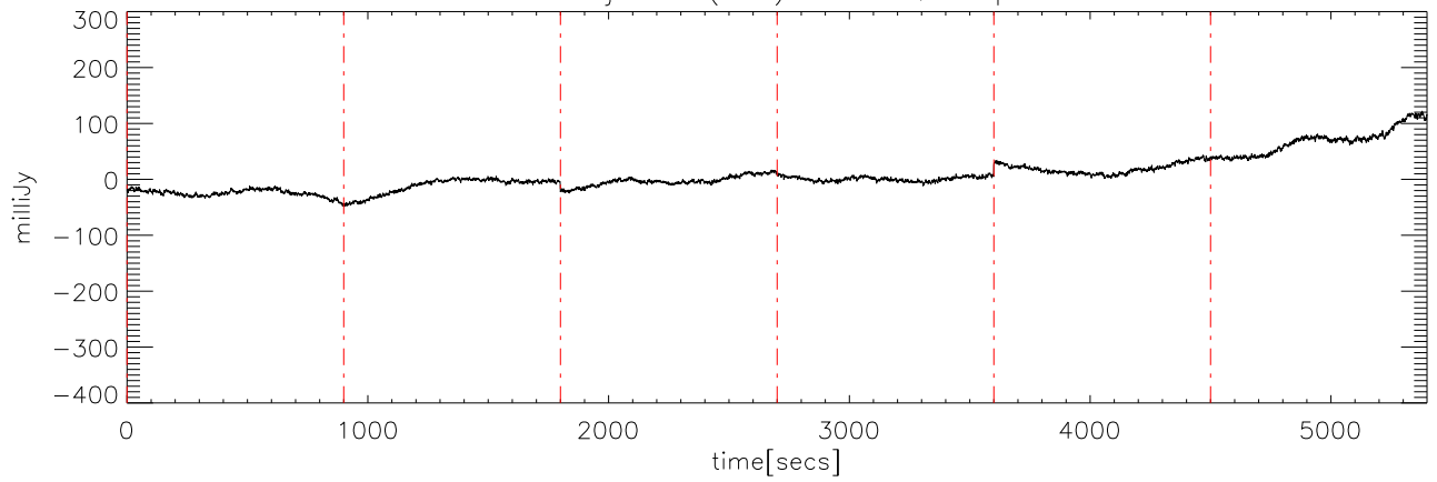
a2414 07jun09 (AST) StokesQ freq:4600.
