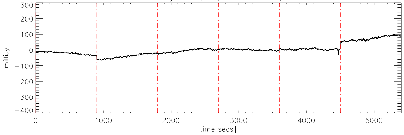
a2414 07jun09 (AST) StokesQ freq:4475.
