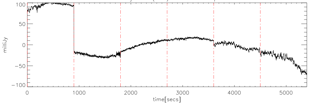
a2414 07jun09 (AST) StokesU freq:5250.
