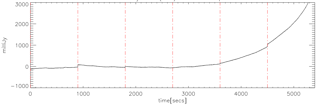
a2414 07jun09 (AST) StokesI freq:4600.
