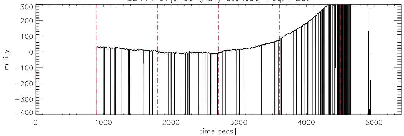
a2414 07jun09 (AST) StokesQ freq:4725.
