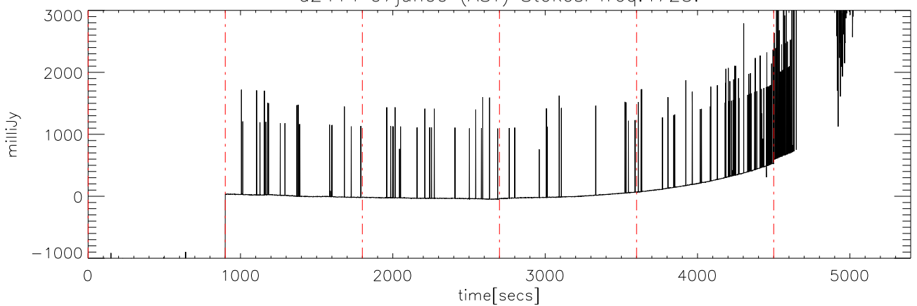
a2414 07jun09 (AST) StokesI freq:4725.
