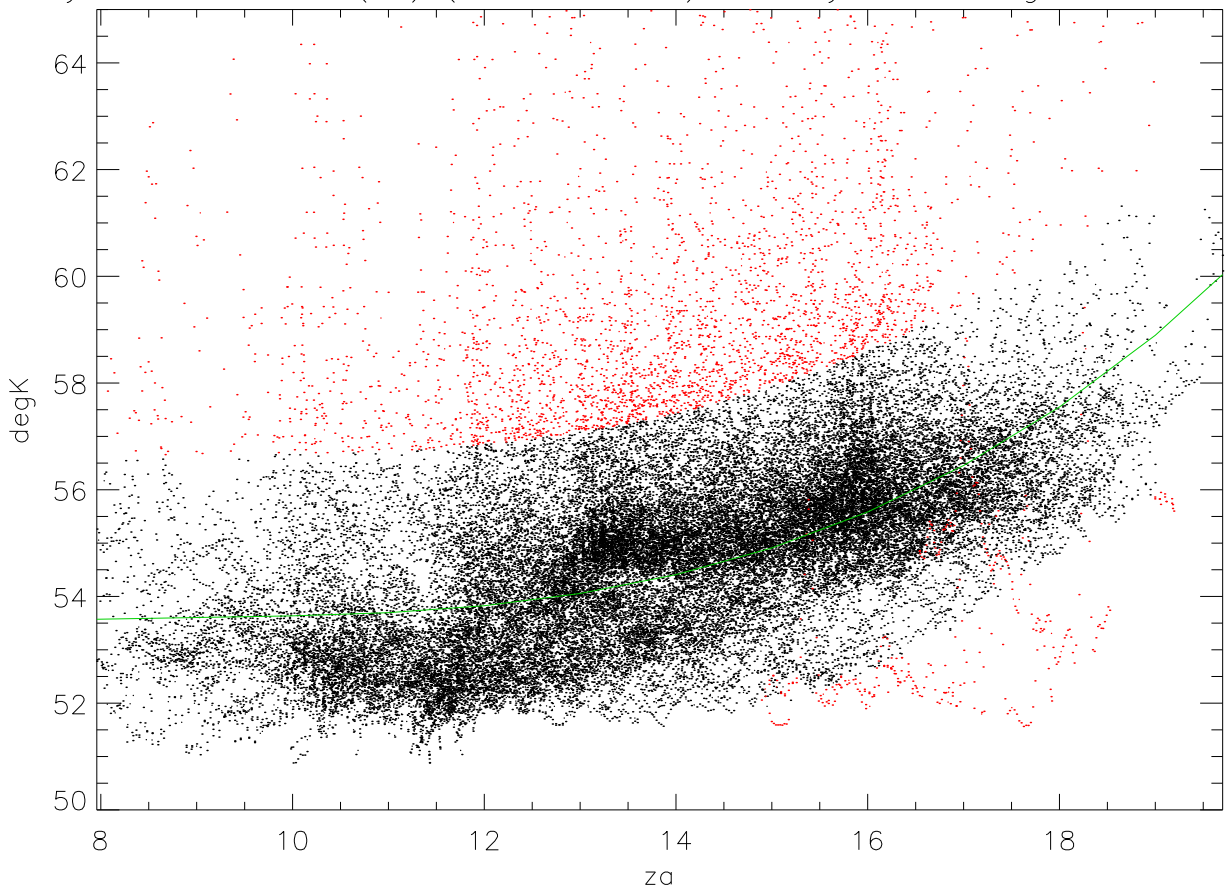
tsys vs za and Fit(za) (all data PoIB) coefTsys:53.64 sigmaFit: 1.20 K
