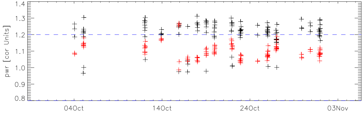
a2048 median strip power vs date. pixel:0
