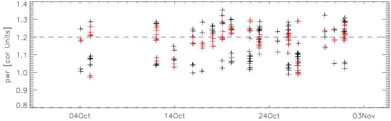
a2048 median strip power vs date. pixel:4
