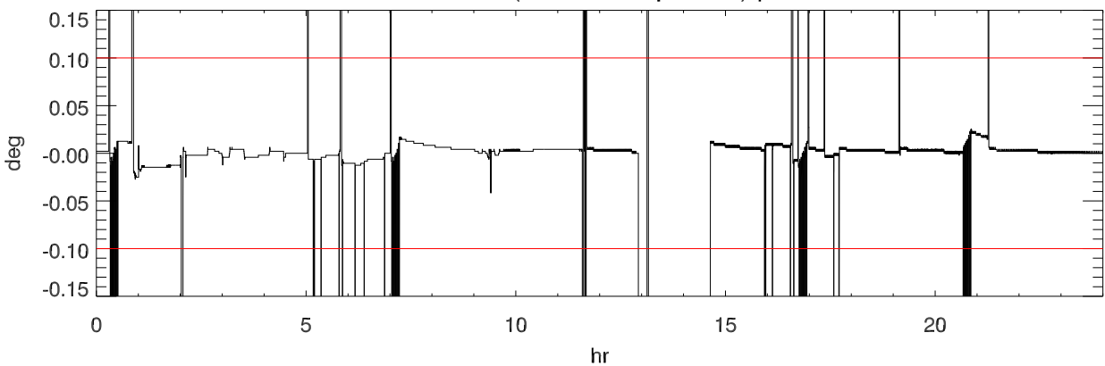
150601 turret (Actual - Requested) position
