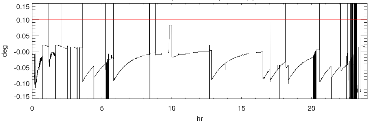
151201 turret (Actual - Requested) position
