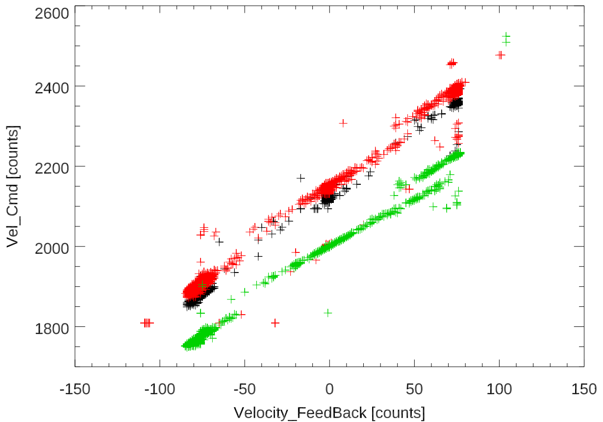
Velocity Command vs velFdbck (by epoch)
