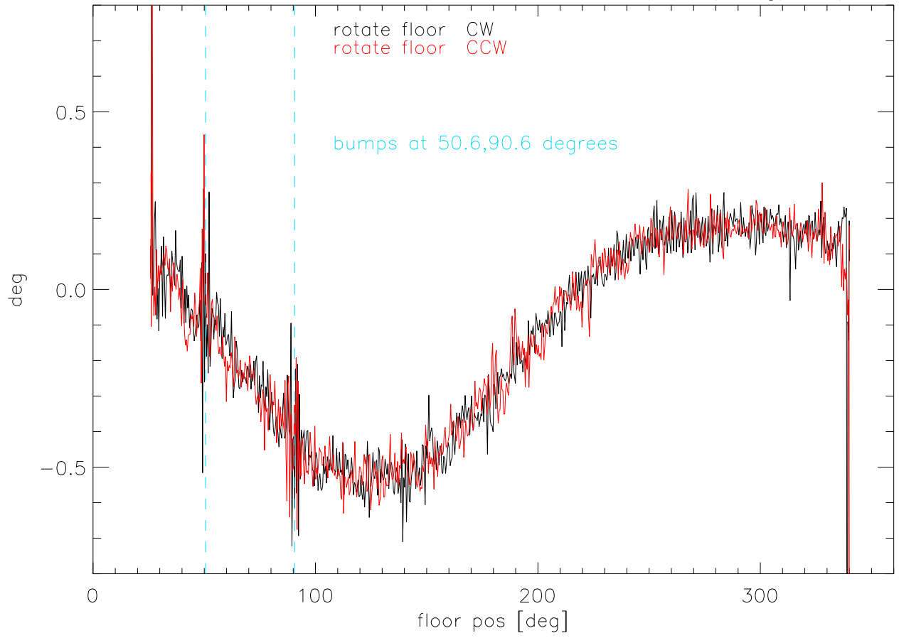
12sep04 tilt sensor roll as turret floor spins (3deg/sec)
