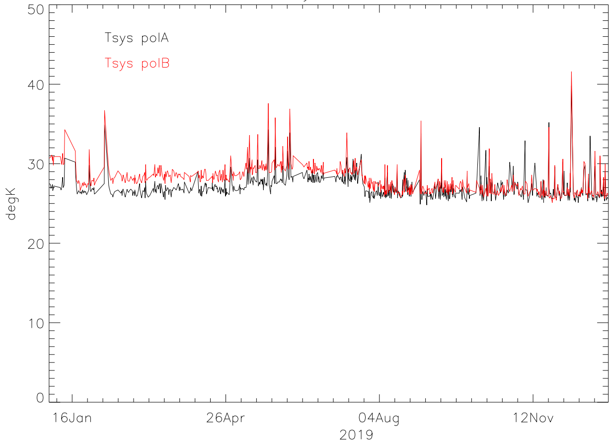
lbw TsysA-TsysB 2019
