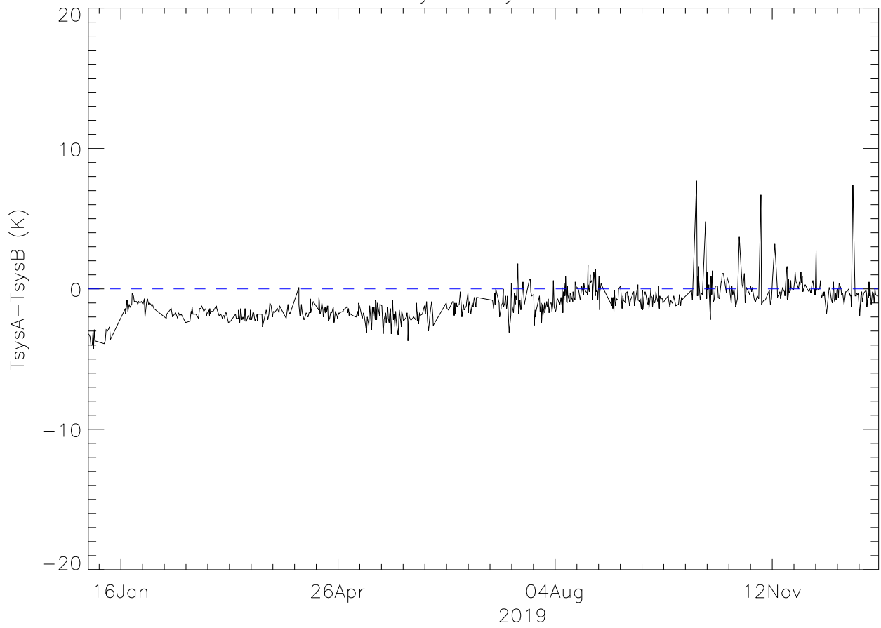
lbw TsysA-TsysB 2019
