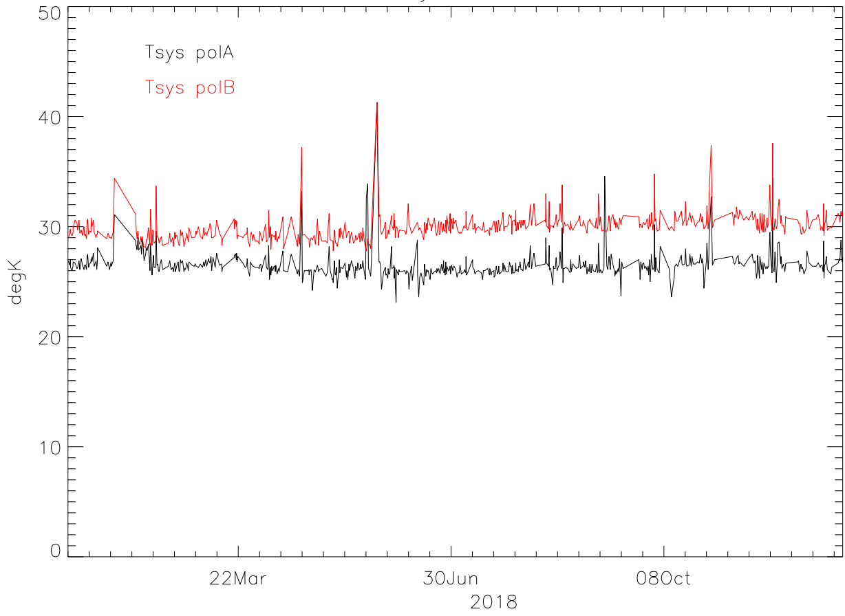
lbw TsysA-TsysB 2018
