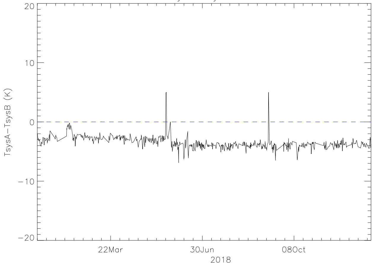
lbw TsysA-TsysB 2018
