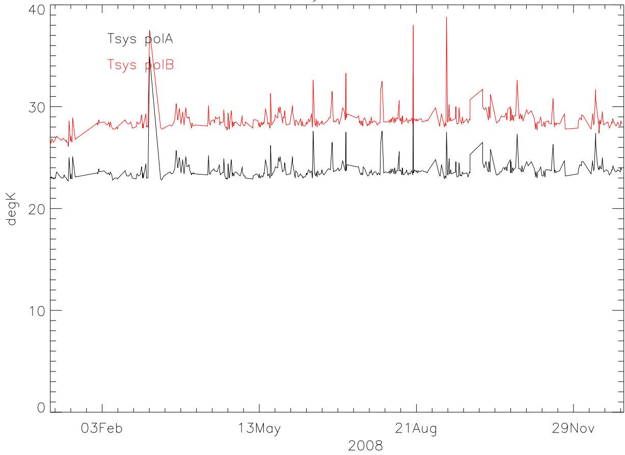
sbn TsysA-TsysB 2008
