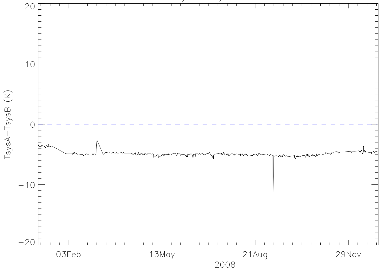
sbn TsysA-TsysB 2008
