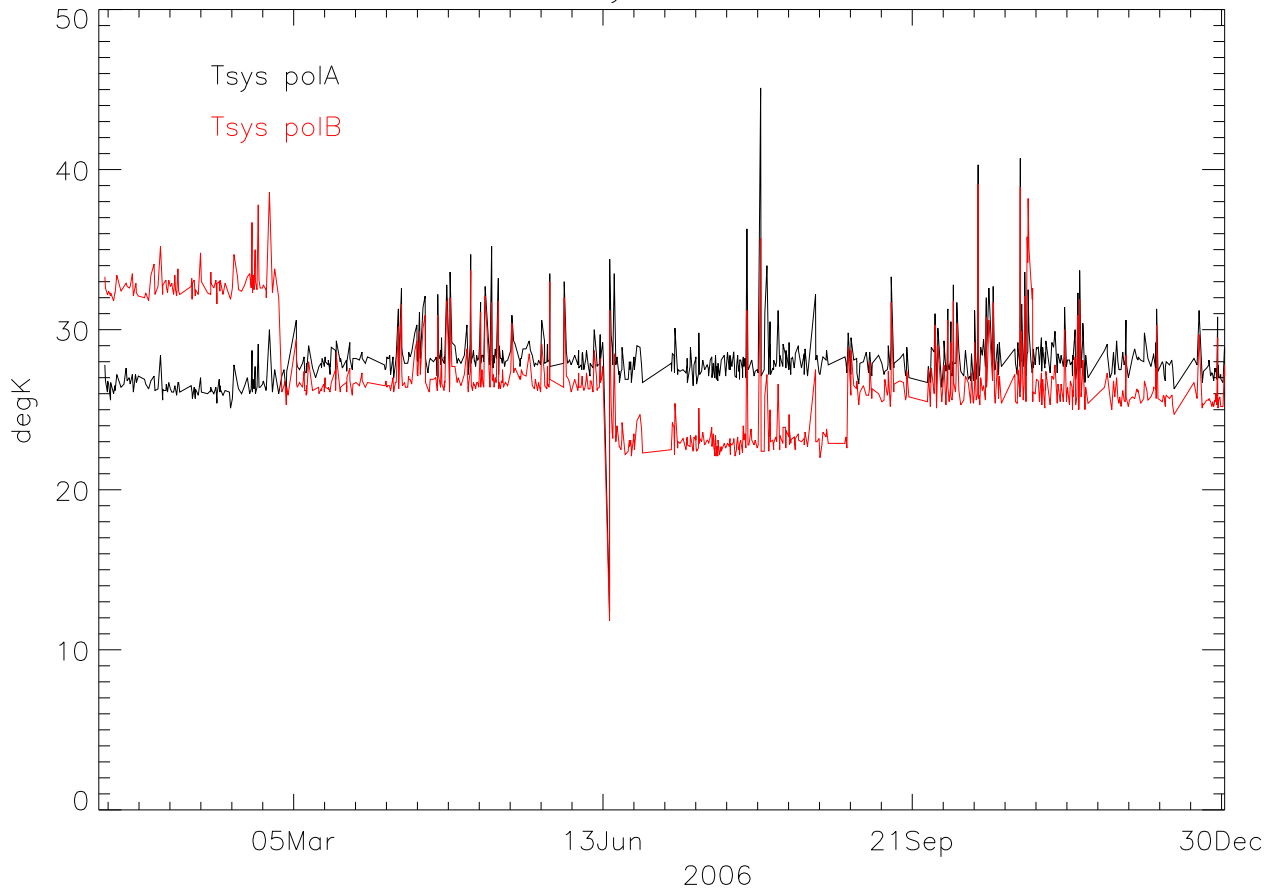
lbw TsysA - TsysB 2006
