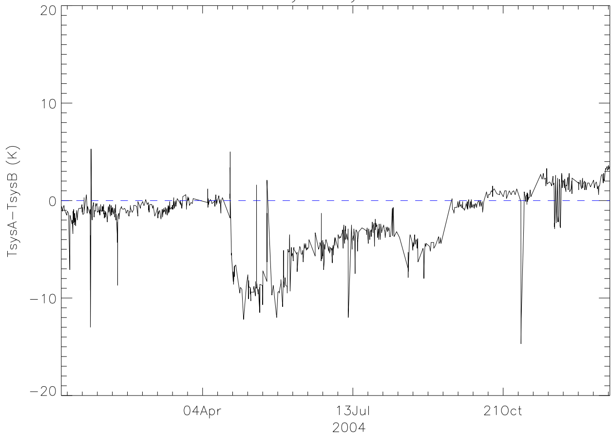
lbw TsysA-TsysB 2004
