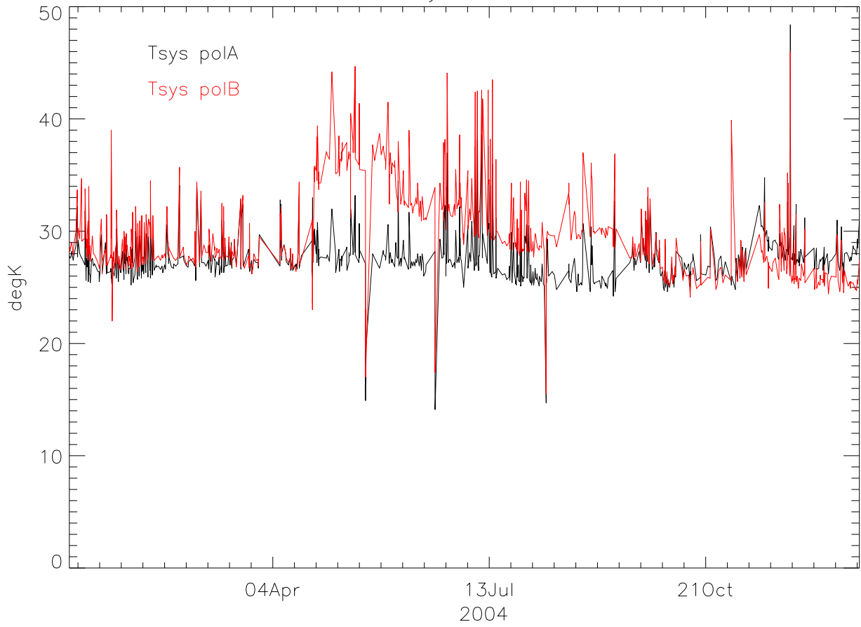
lbw TsysA-TsysB 2004
