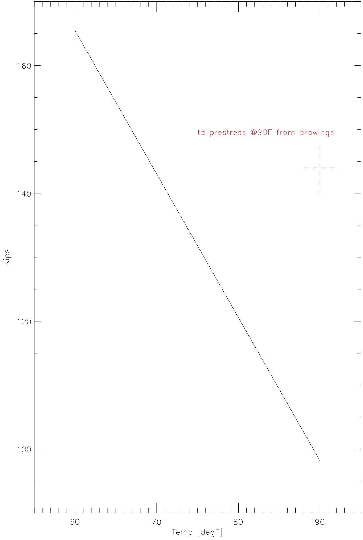
Total tiedown tension vs temp
