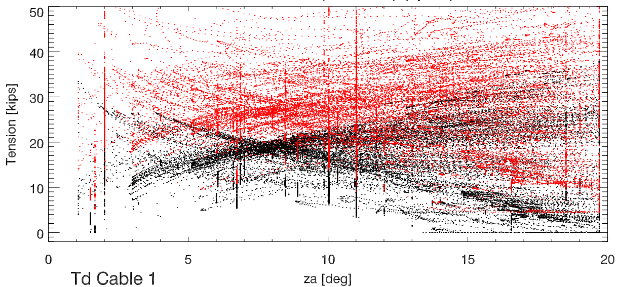
tiedown tensions vs za (ch@stow) (apr13). Td12
