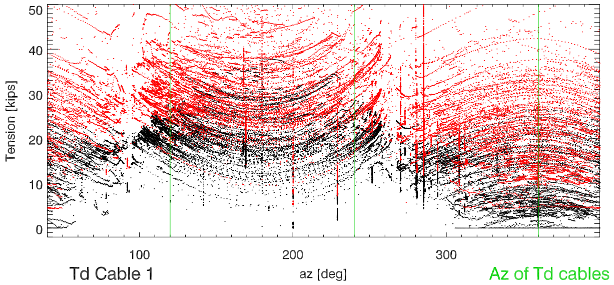
tiedown tensions vs azimuth.ch@stow (apr13). Td12
