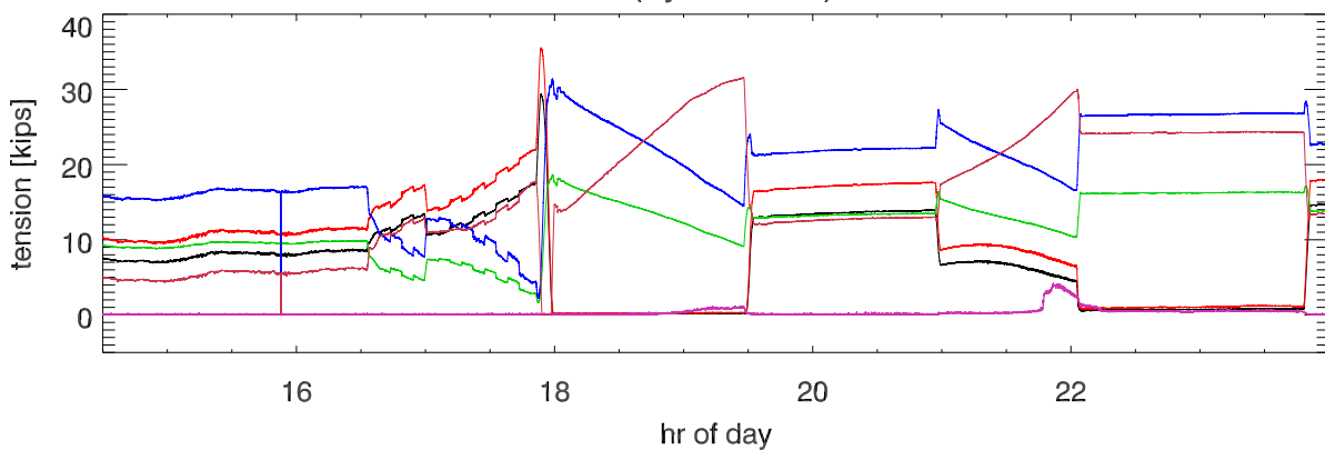
191115 td tensions (by load cell). After calibration.
