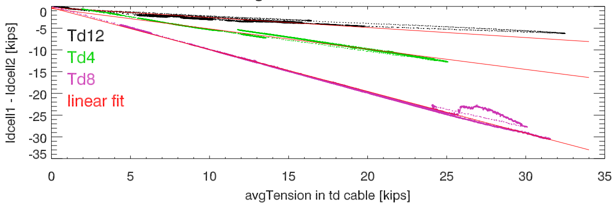
ldCell1 - ldCell2 vs avg tension for 3 tiedowns. After calibration.
