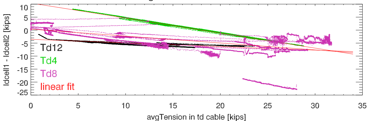
ldCell1 - ldCell2 vs avg tension for 3 tiedowns. Before calibration.
