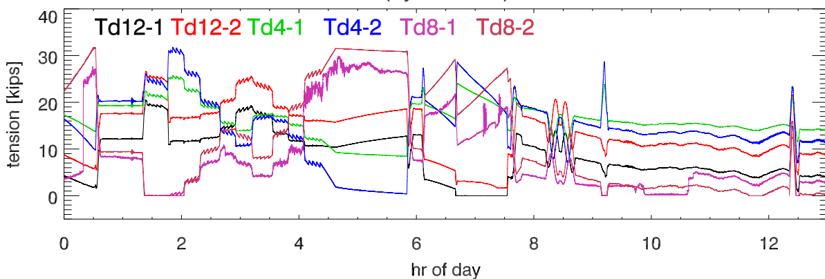
191115 td tensions (by load cell). Before calibration.
