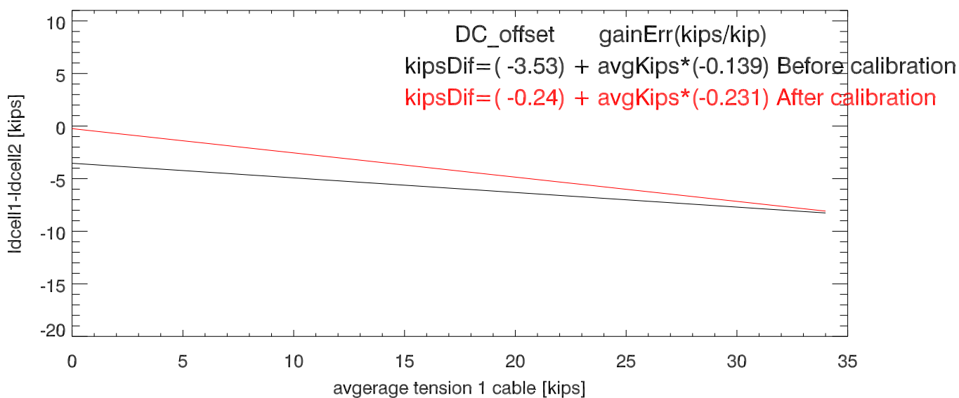
linear fits to Idcell1-Idcell2. Td12
