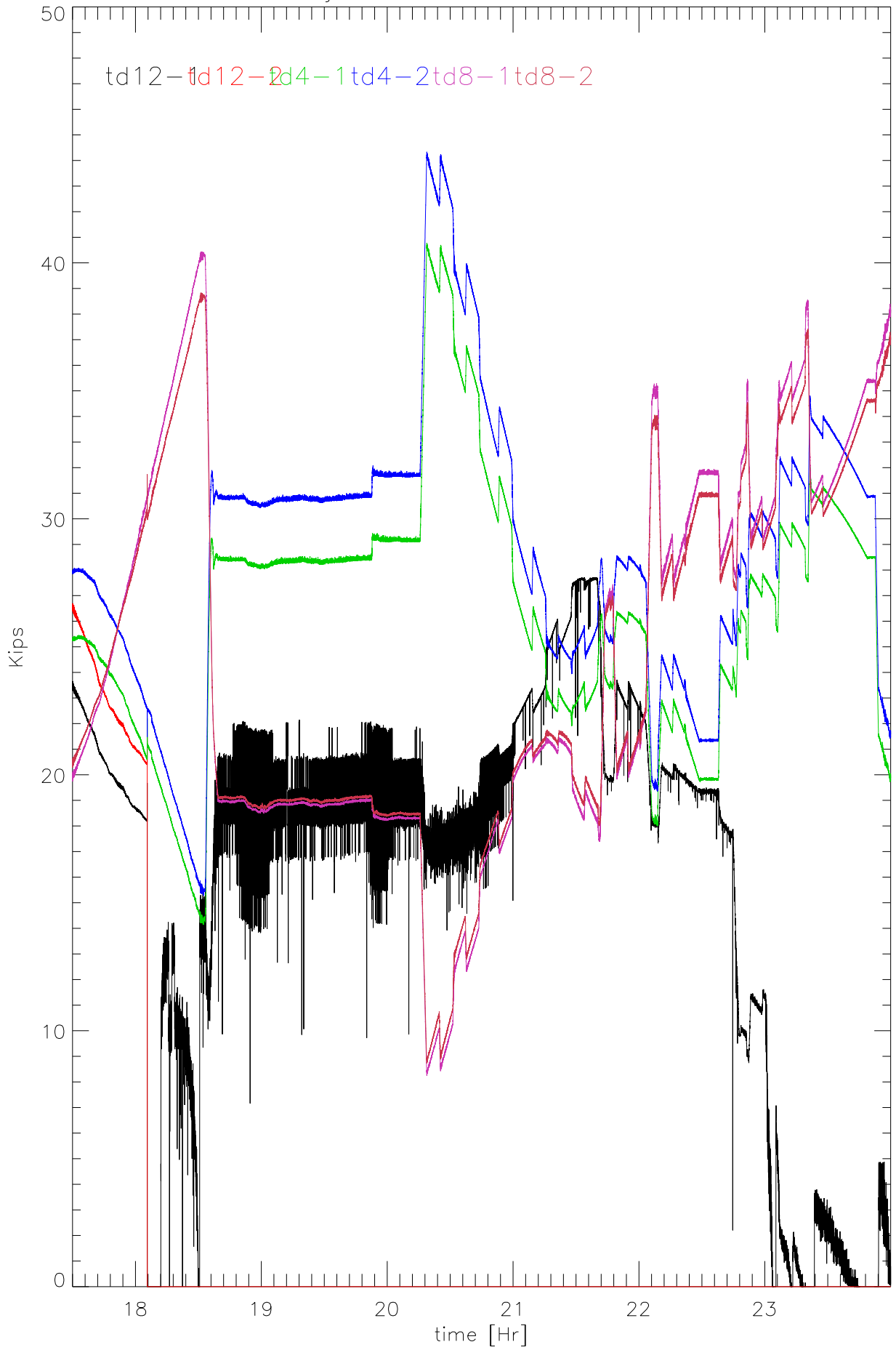
08jun08 td tensions vs time
