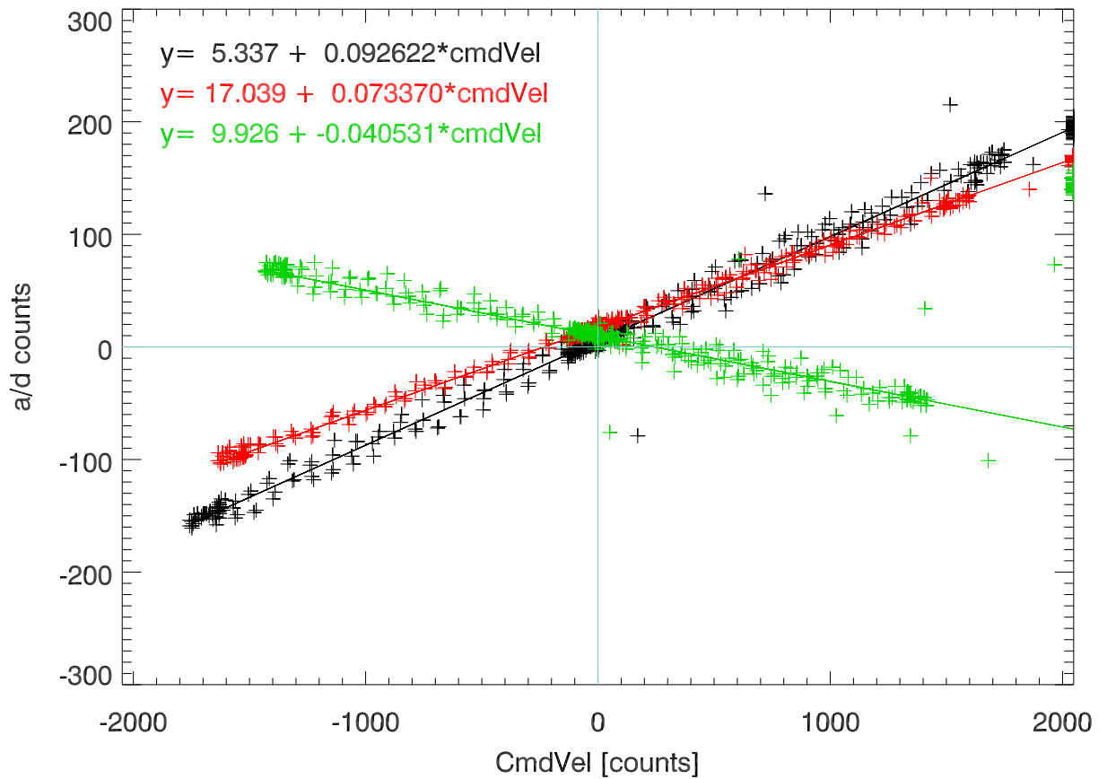
(CmdVel - SpdMon) vs CmdVel
