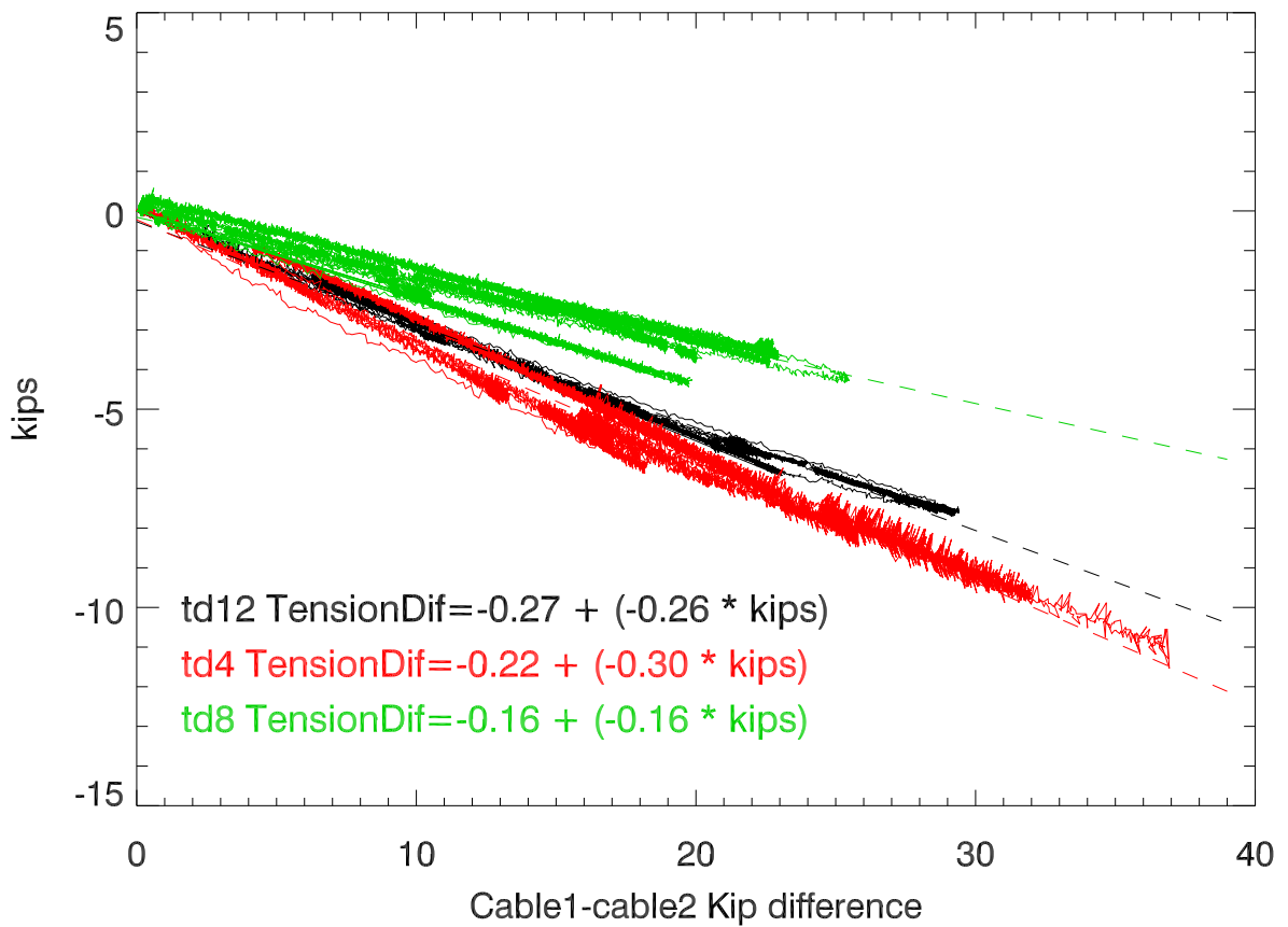
Cable 1 -cable2 kip difference vs kips in cable
