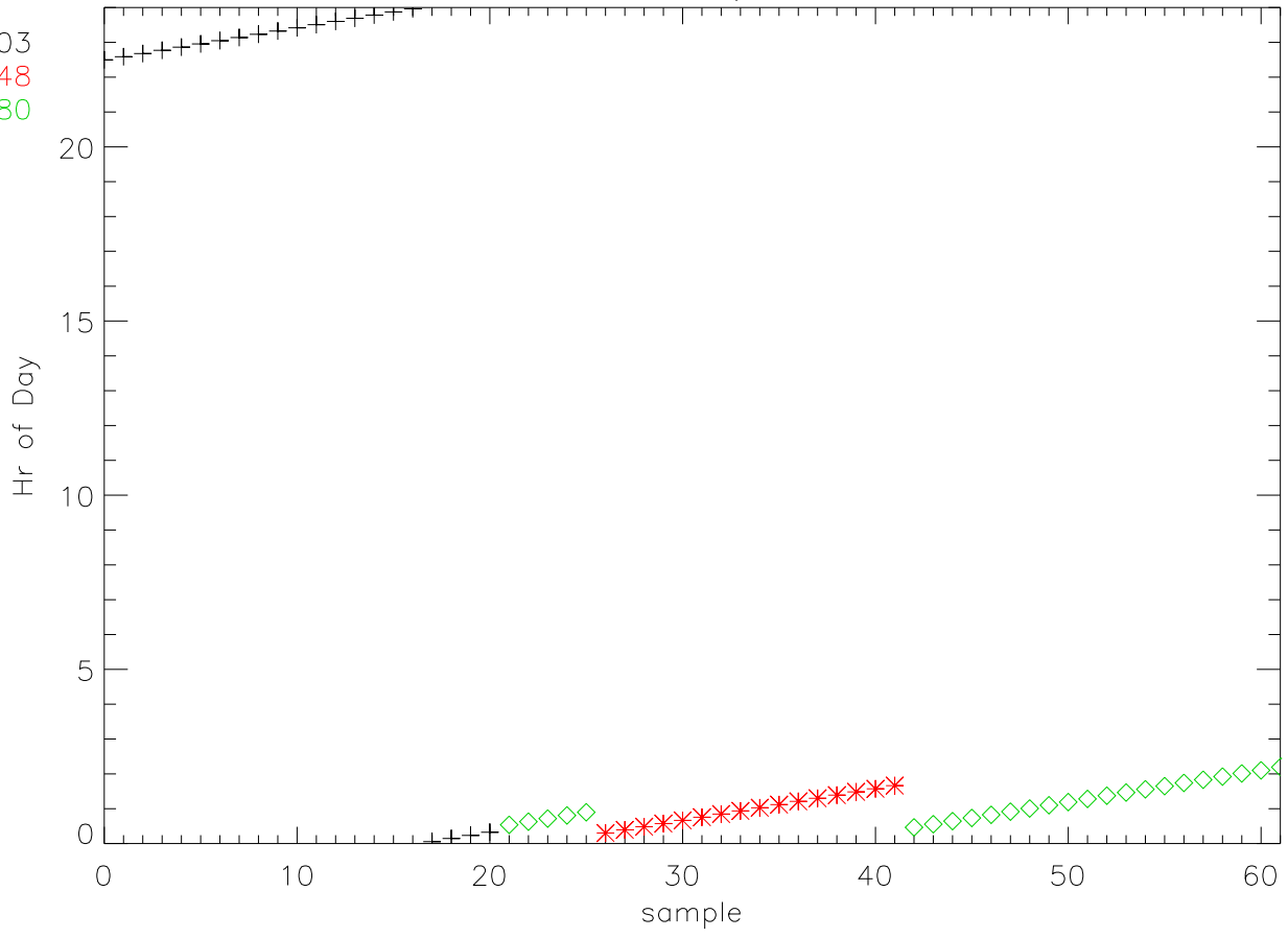
lbw hour of day for data
