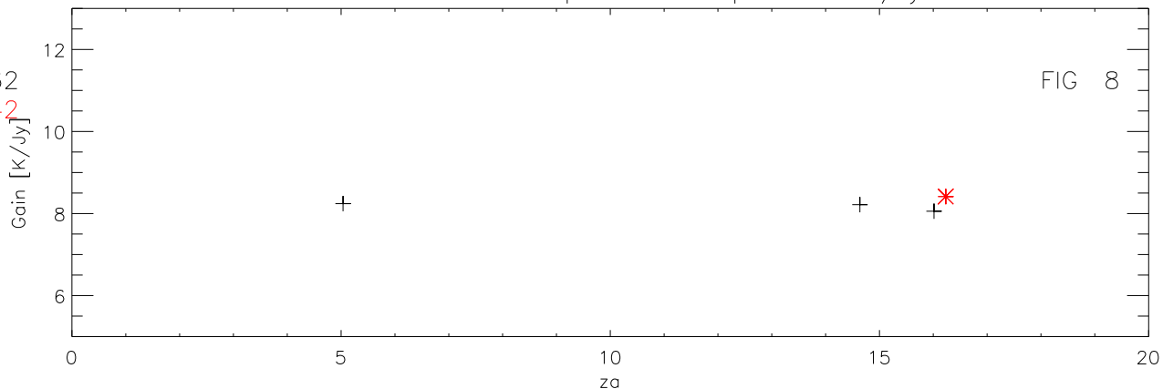
01feb10 to 28feb10 pixel 6 4 pnts. Gain K/Jy
