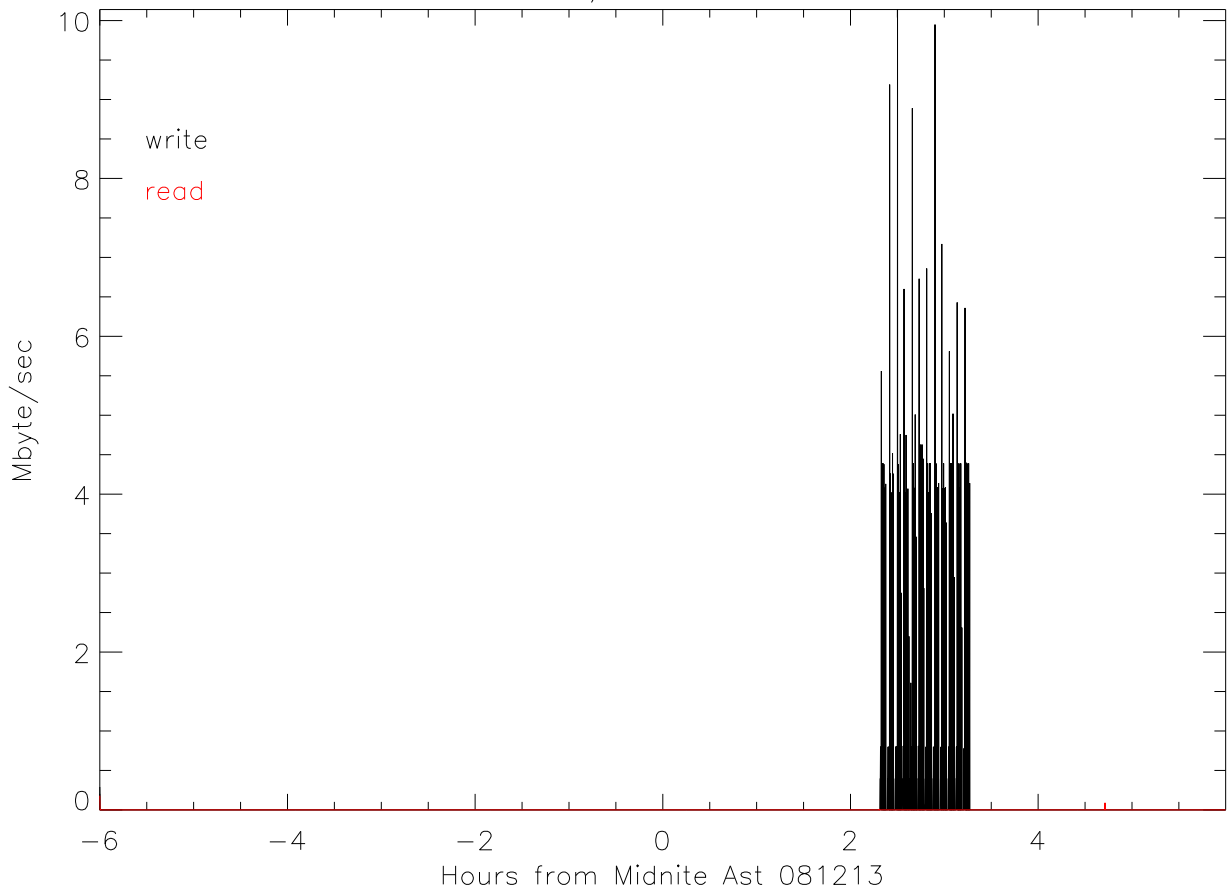
I/O rates
