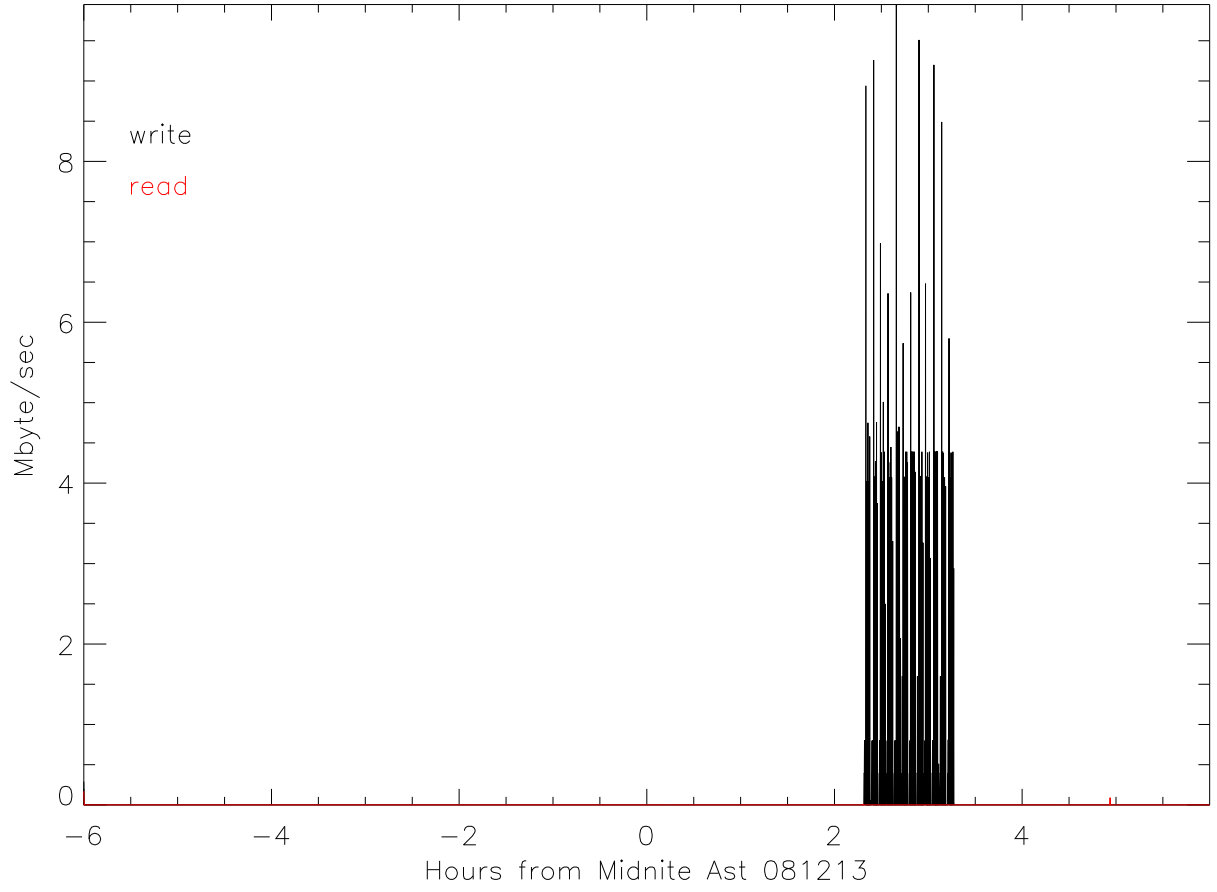
I/O rates
