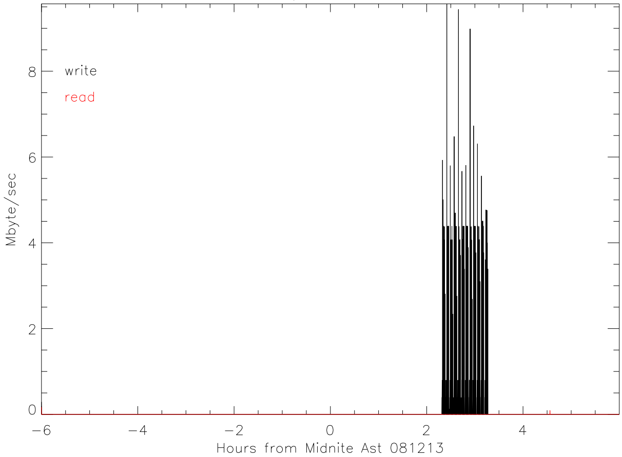
I/O rates
