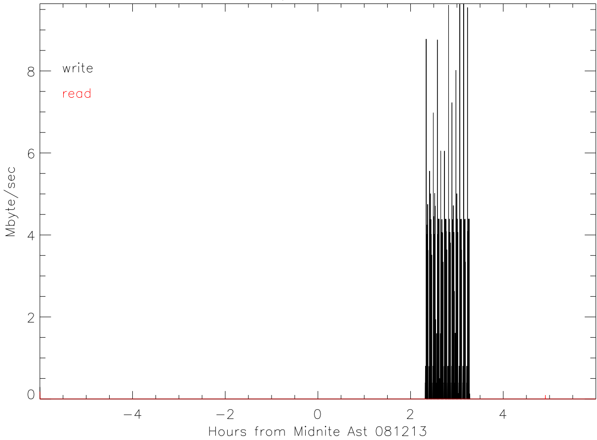
I/O rates
