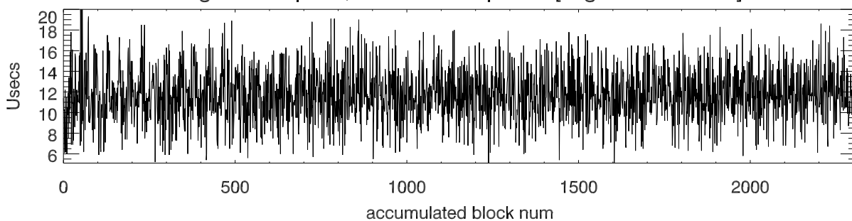
avg time cmpPwr, accum 1 4k spectra [avg: 11.7 rms: 2.6]
