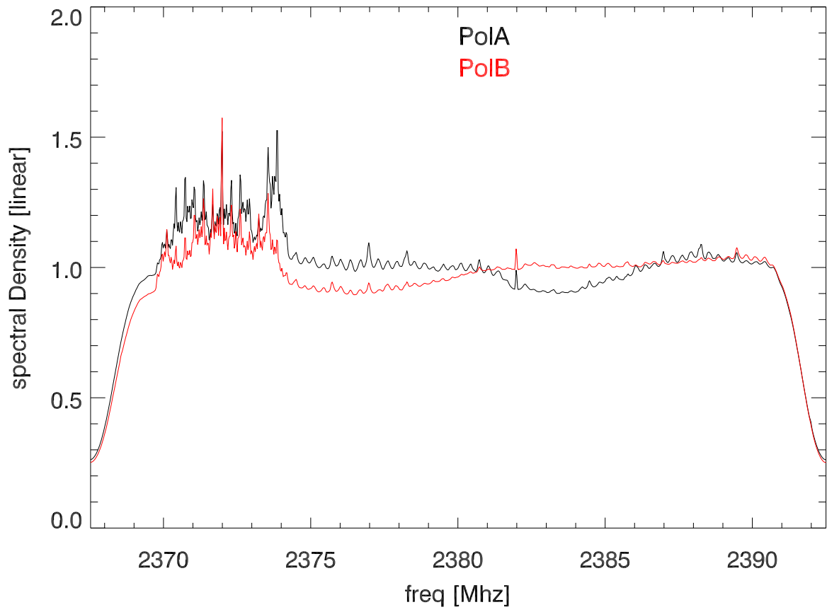
30dec15 x111 60 second average sbn spectra
