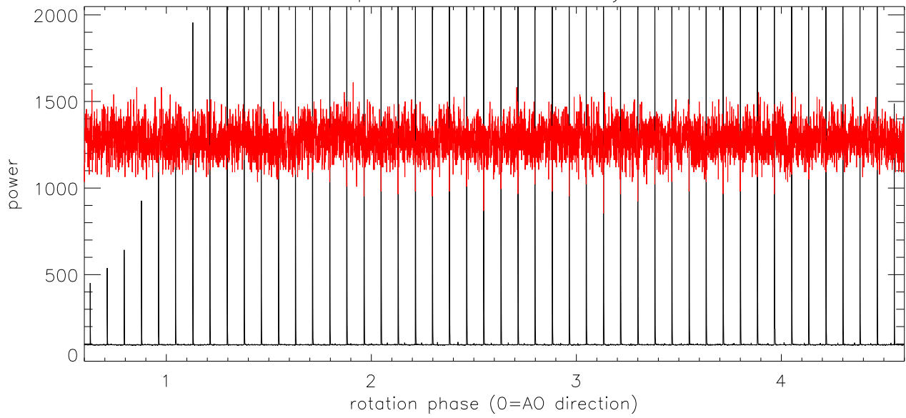
Blowup birdie at az=60 FAA radar
