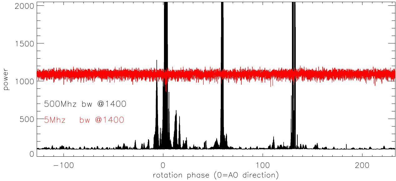
Blowup birdie at az=0. Remy radar
