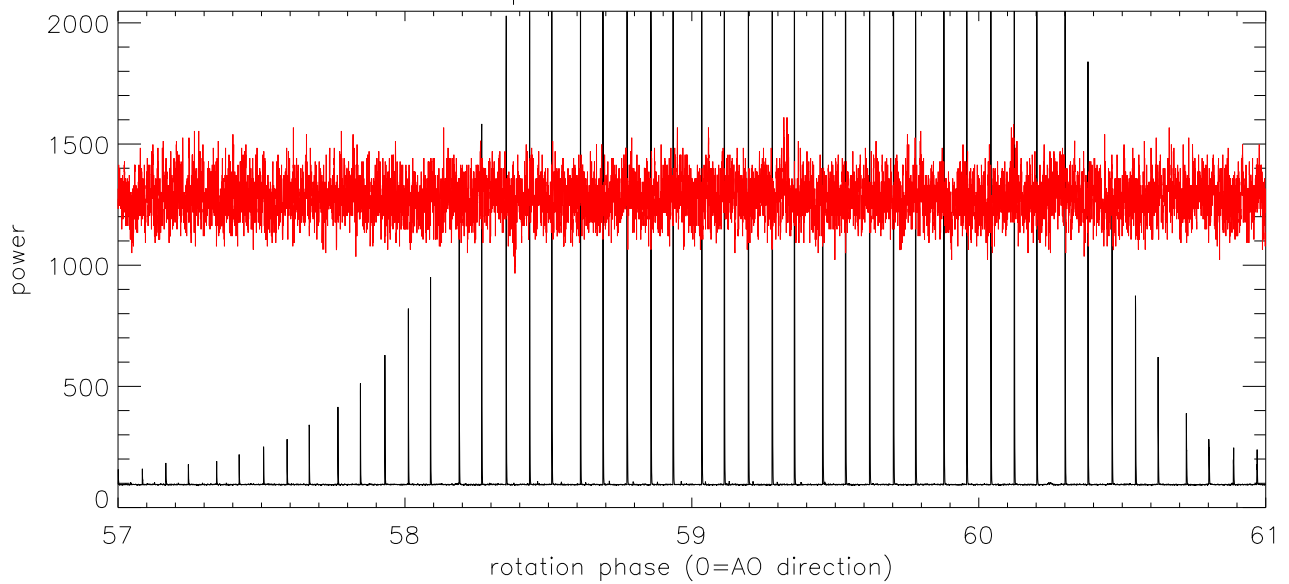
Blowup birdie at az=60 FAA radar
