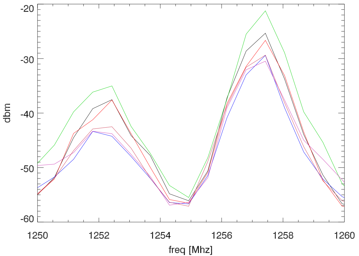
faa radar 1257.6 Mhz
