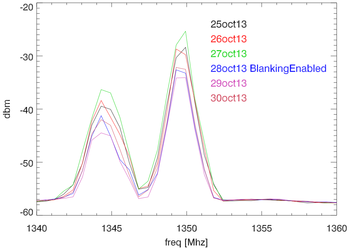
hilltop rfi monitor. 27-30 oct13 faa radar. 1349.6 Mhz
