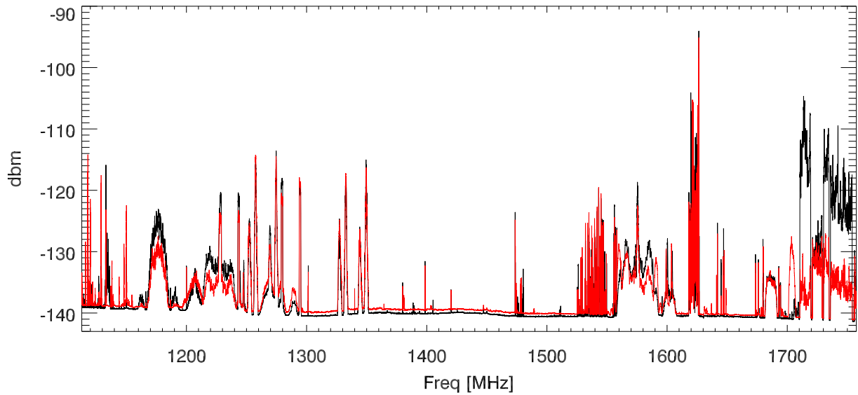
Peak hold spectra over swing
