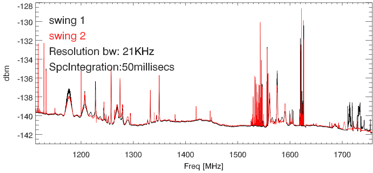
20190222 lbw azswing. Average spectra
