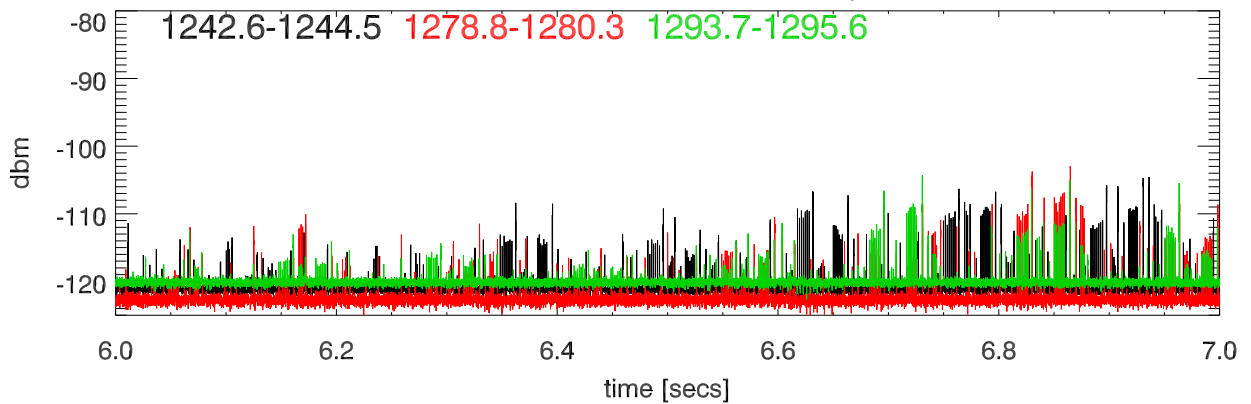
TotPwr vs time PuntaSalinas modeA (only 3 frequencies)
