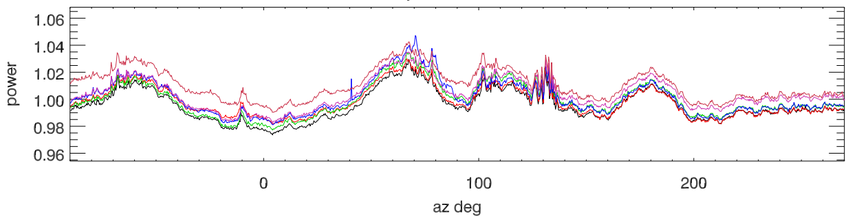
freq:4910. to 4920.
